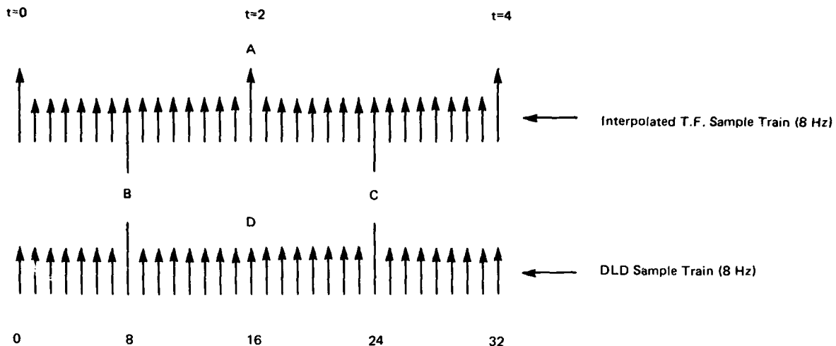
FIG. 2: TIME ALIGNMENT OF DATA TO COMPLEMENTARY FILTER
