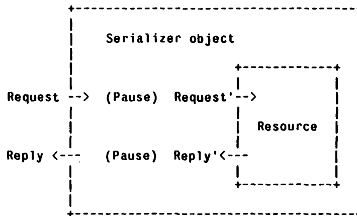
Figure 1. A picture of a serializer object
