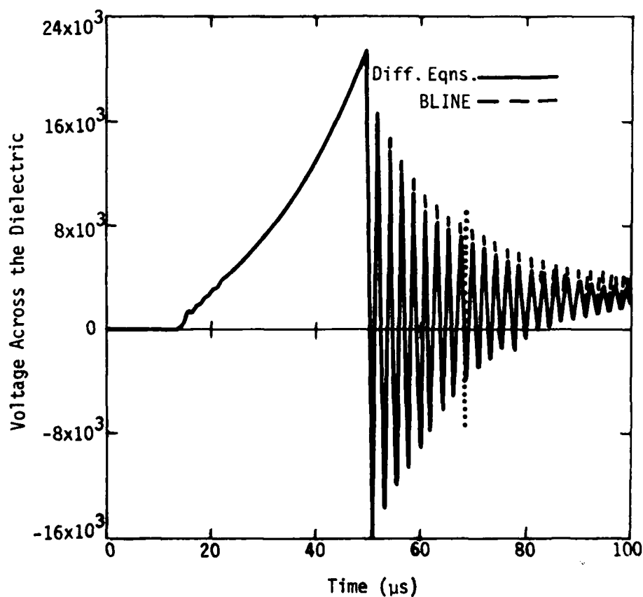
Figure 10. Dielectric Voltages Predicted by BLINE and the Differential Equation Technique at the Cable Termination
