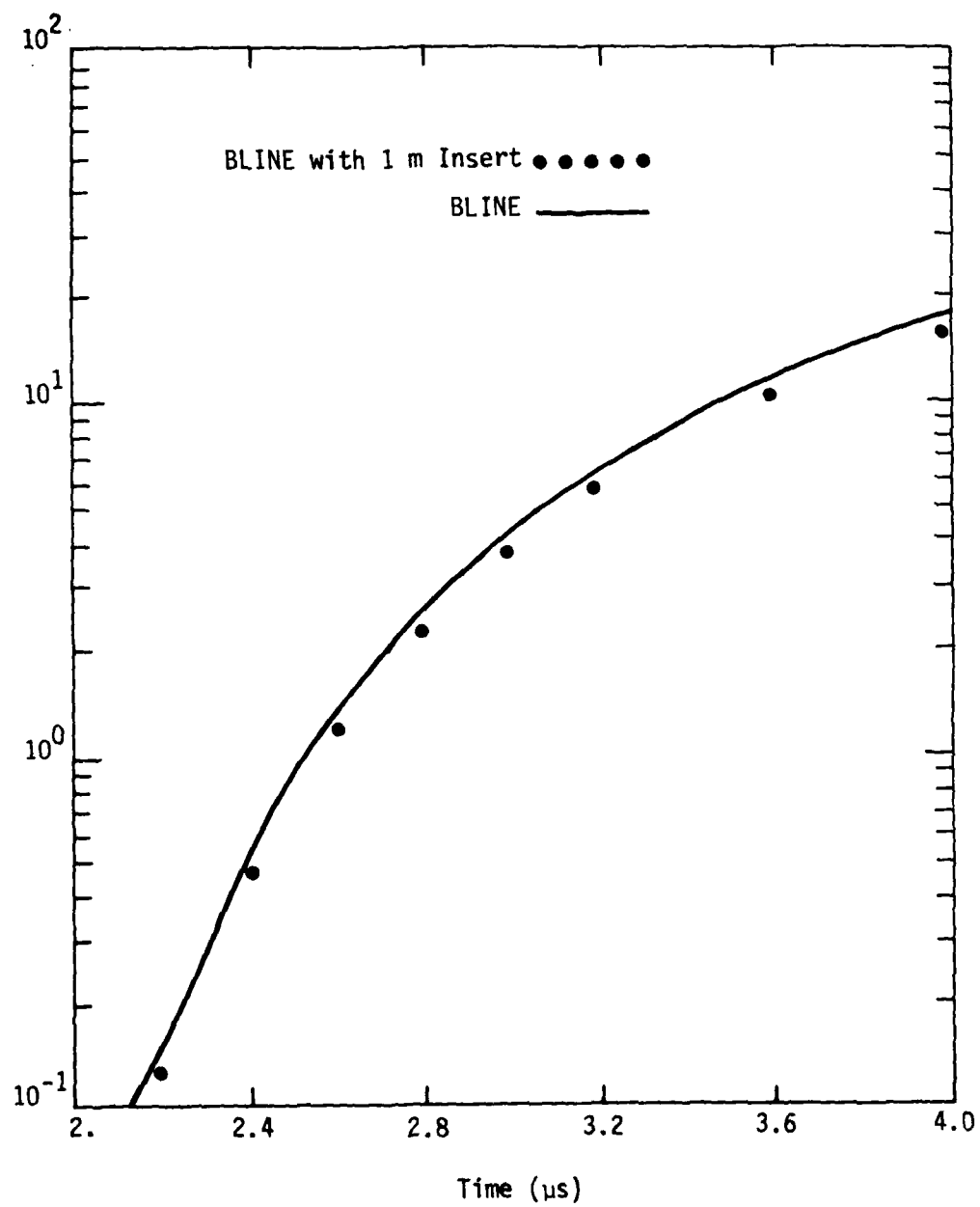
Figure 5. Predicted Voltage at the Load End of the Cable
