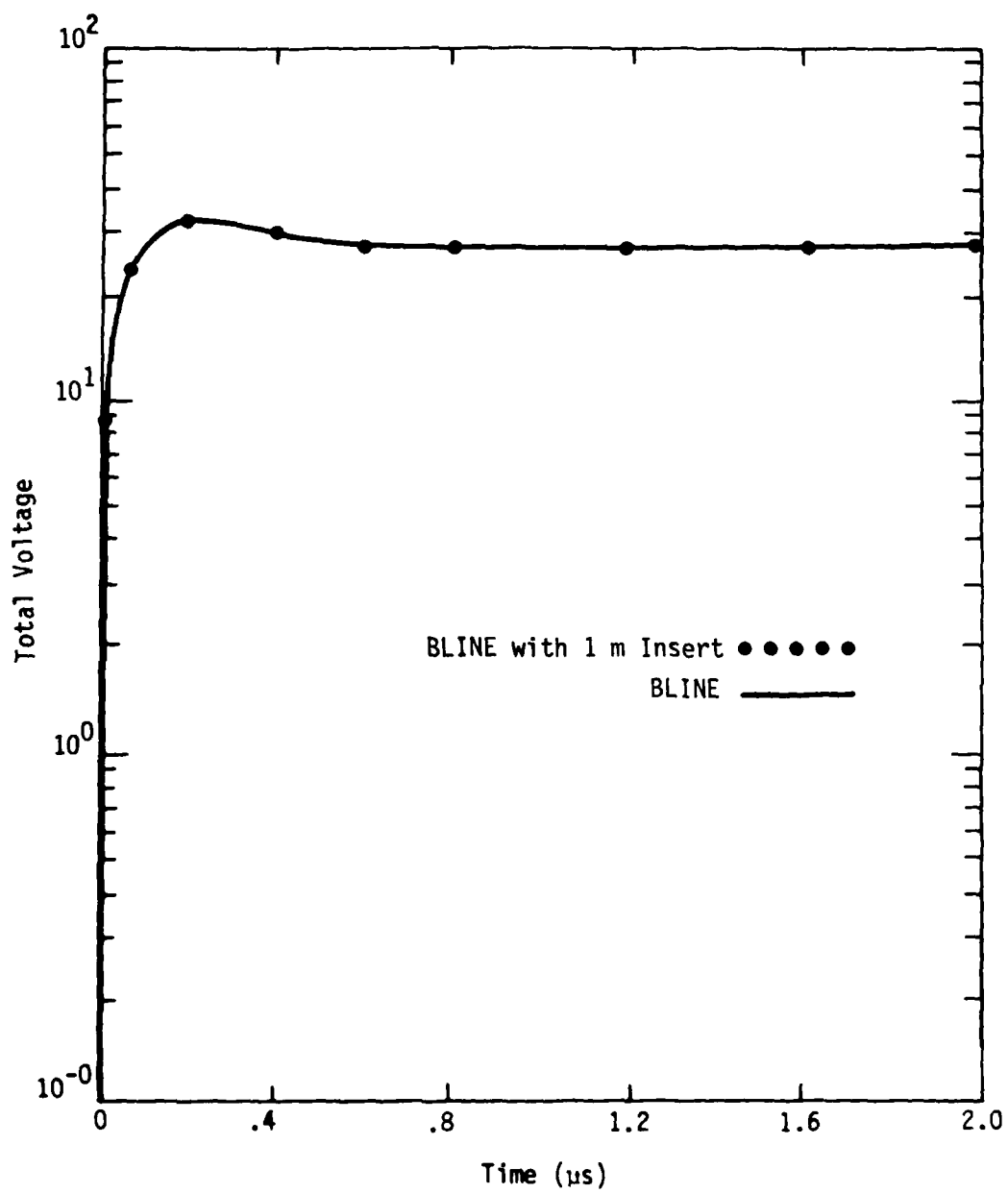
Figure 4. Predicted Voltage at the Source End of the Cable
