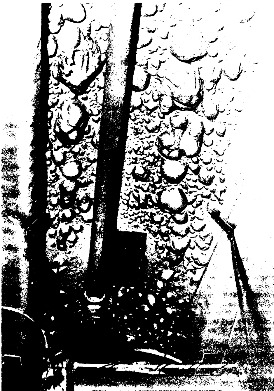
FIGURE 22. SEVERE BLISTERING OF THE CEILING PANELS BETWEEN FUSELAGE STATIONS 466 AND 526 WITHOUT EVIDENCE OF FLAMING
