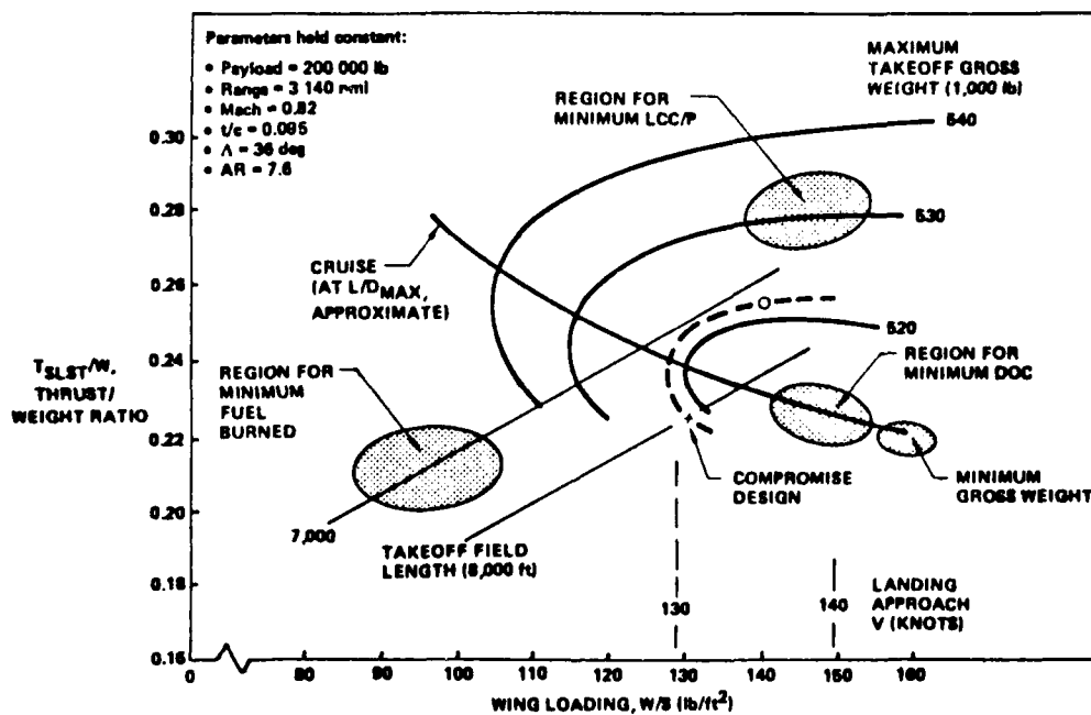
Figure 3.6.10 Engine/Airframe Matching
