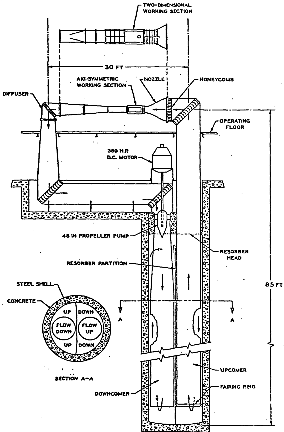
High Speed Water Tunnel Circuit Schematic
