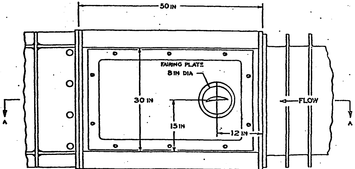
FLEXGLAS WINDOWS TOP AND BOTTOM Two-Dimensional Working Section Schematic
