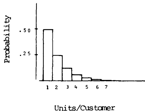
Figure 9. Typical Geometric Distribution
