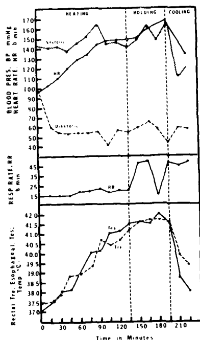
FIGURE 1. Physiological responses (RR, HR, BP, T_{re} and T_{es} ) of a male patient (National Cancer Institute) to induced hyperthermia (holding T_{es} = 41.8 \pm 0.2^{\circ}\text{C} ) using an insulated suit through which 46^{\circ}\text{C} water was circulated.
