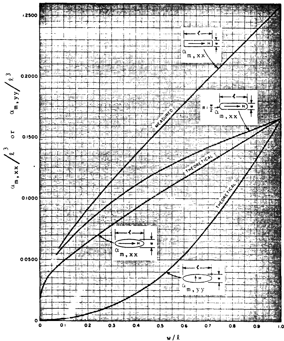
Figure C.12. Normalized Magnetic Polarizability
