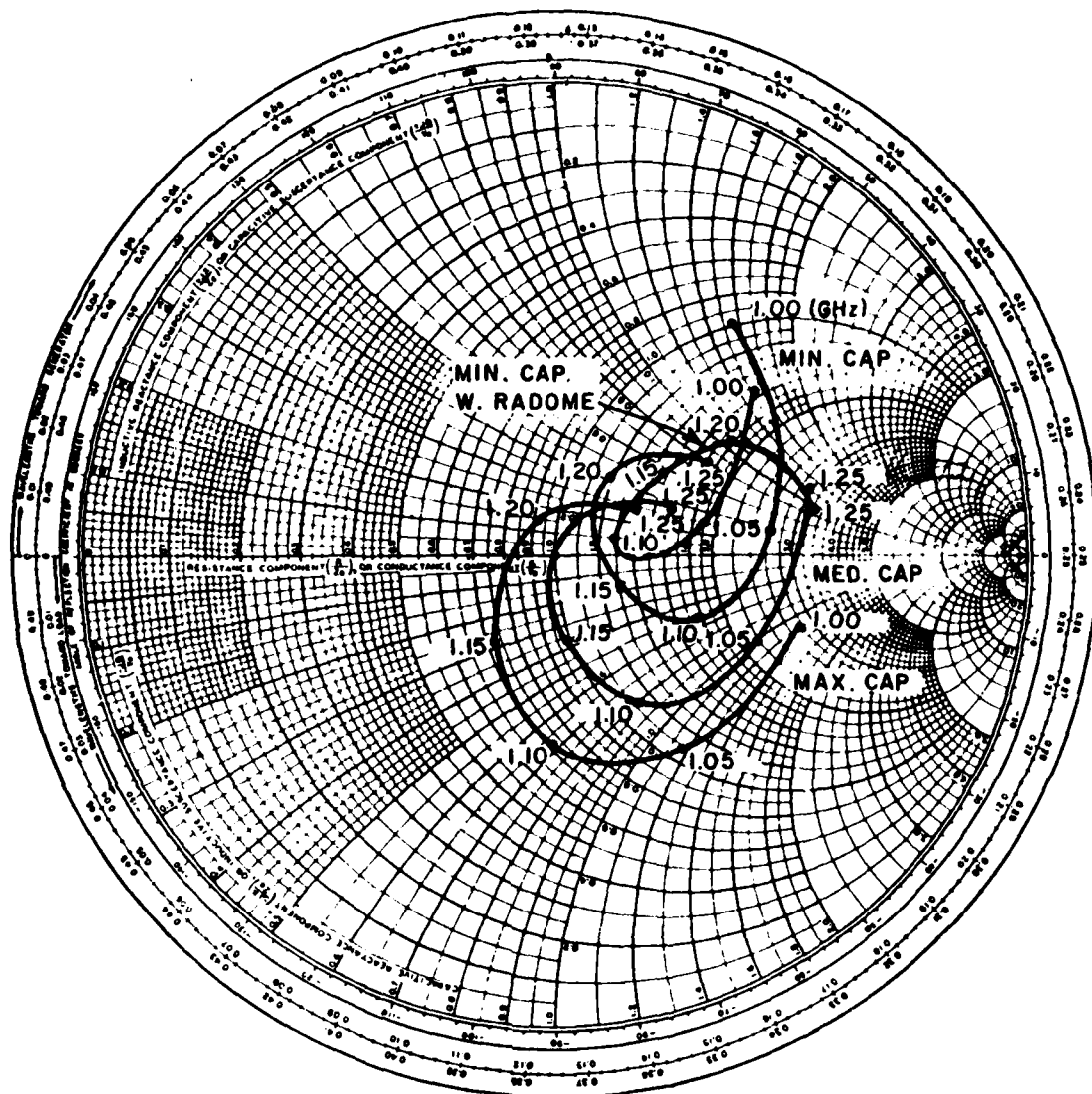
Figure 8. The input impedance of a single loop for positions of the capacitor shown in Figure 7. The other three loops were open circuited.
