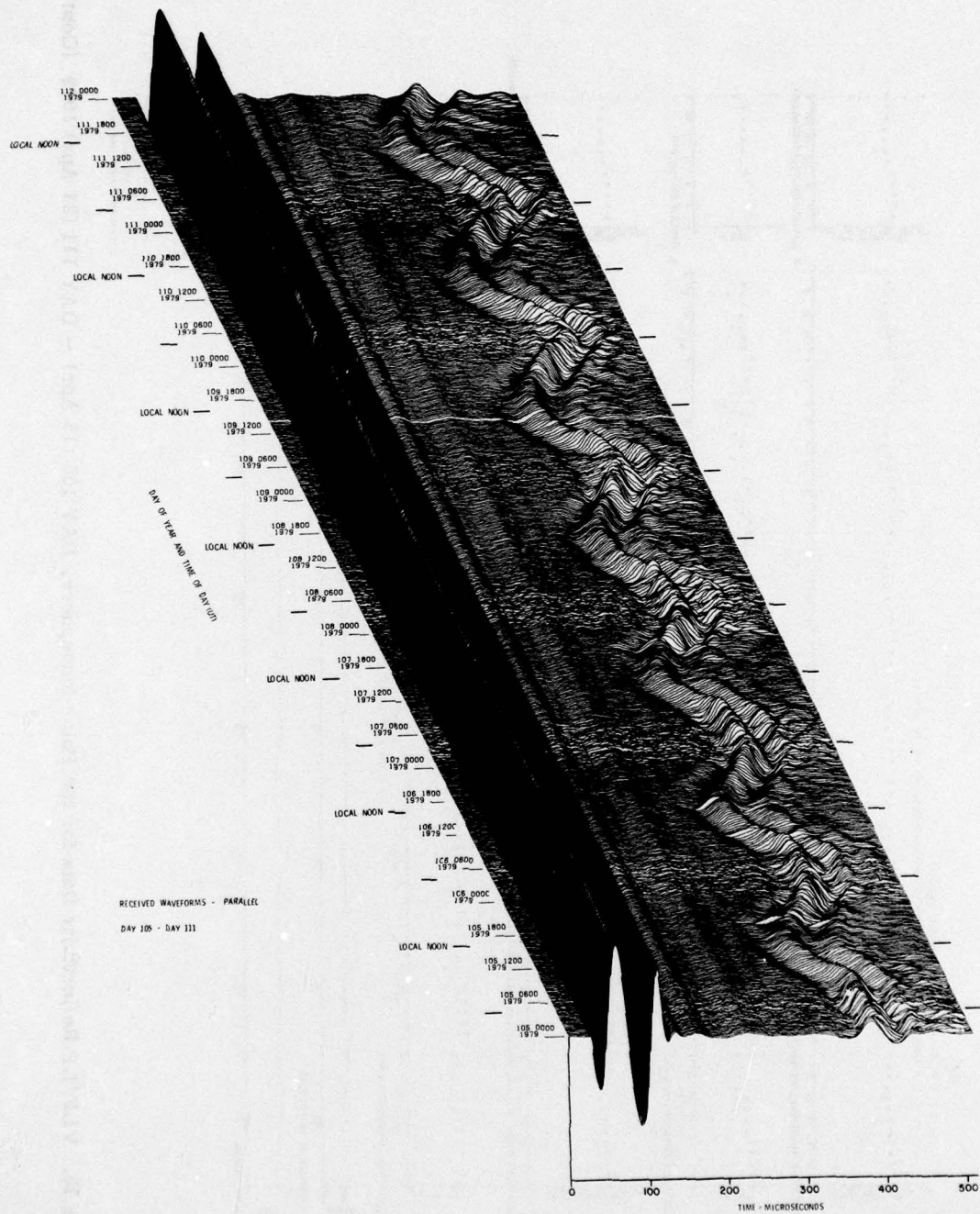
Figure 18. VLF/LF Reflectivity Data for the Polar Ionosphere, DAY 105 (15 Apr) - DAY 111 (21 Apr) 1979 (Cont) Part R. || Waveform Display
