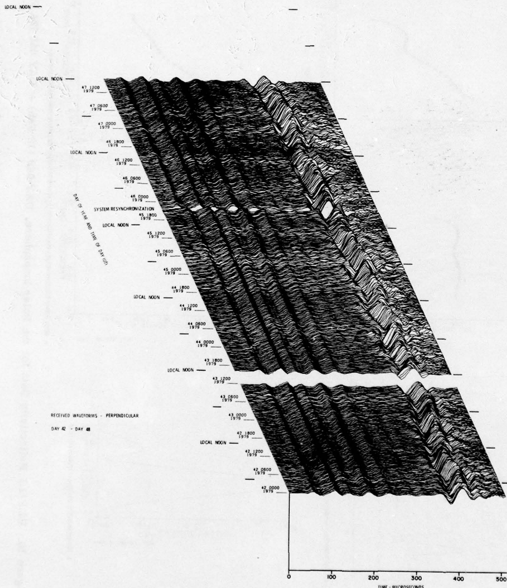
Figure 9. VLF/LF Reflectivity Data for the Polar Ionosphere, DAY 042 (11 Feb) - DAY 048 (17 Feb) 1979 (Cont) Part S. \perp Waveform Display
