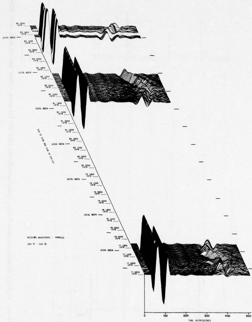
Figure 14. VLF/LF Reflectivity Data for the Polar Ionosphere, DAY 077 (18 Mar) - DAY 083 (24 Mar) 1979 (Cont) Part R. || Waveform Display
