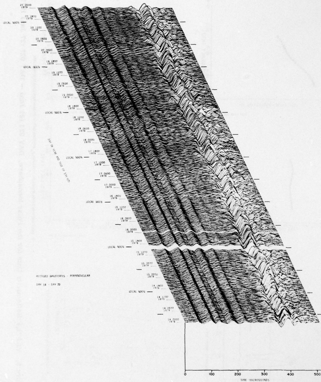
Figure 5. VLF/LF Reflectivity Data for the Polar Ionosphere, DAY 014 (14 Jan) - DAY 020 (20 Jan) 1979 (Cont) Part S. \perp Waveform Display
