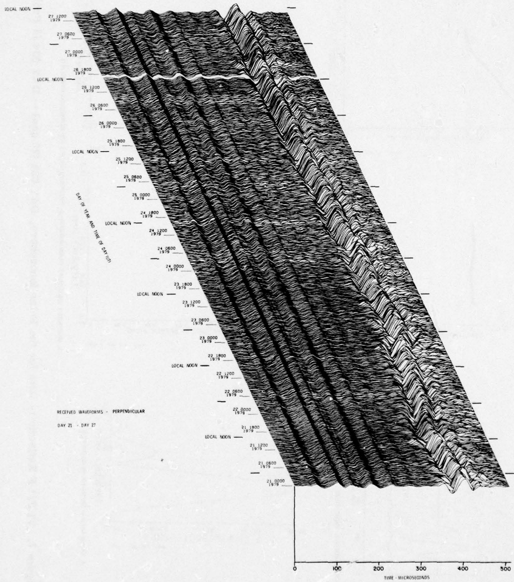
Figure 6. VLF/LF Reflectivity Data for the Polar Ionosphere, DAY 021 (21 Jan) - DAY 027 (27 Jan) 1979 (Cont) Part S. \perp Waveform Display
