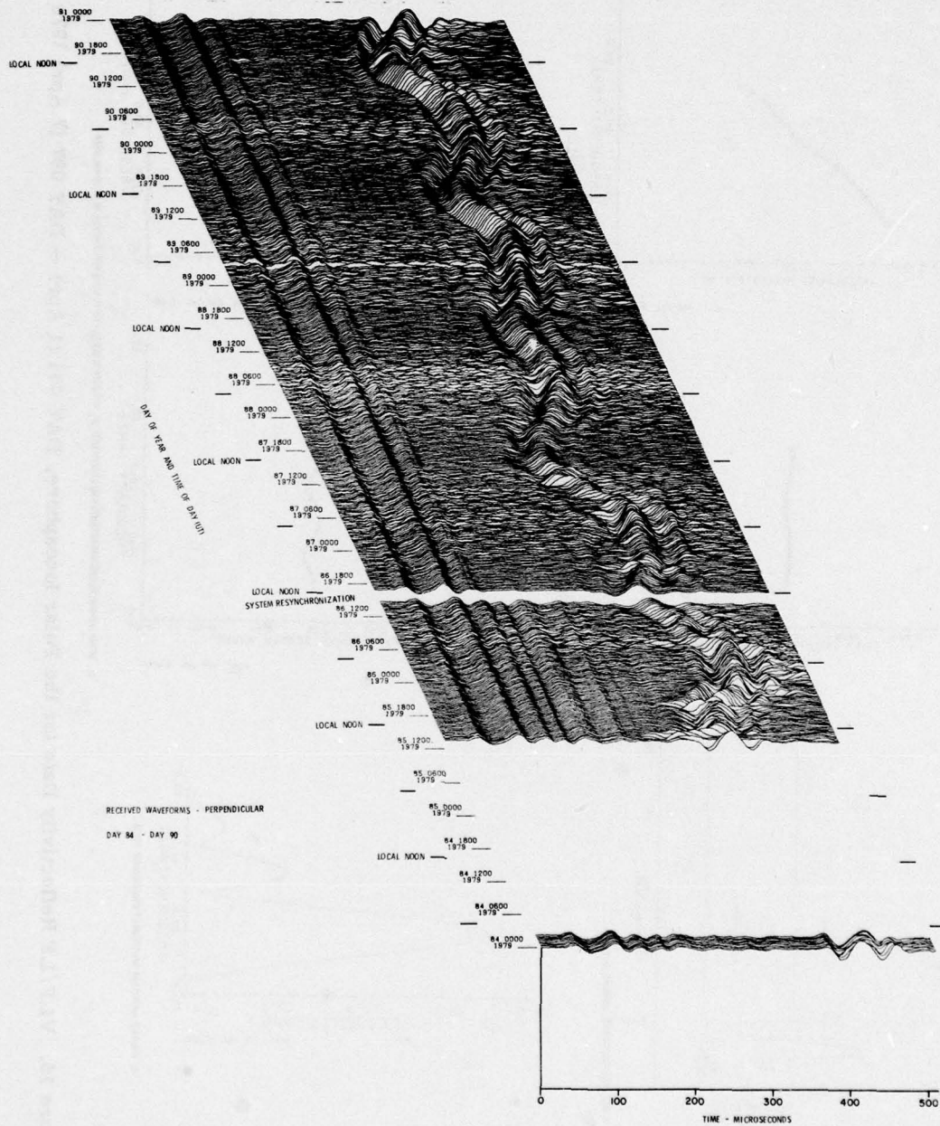
Figure 15. VLF/LF Reflectivity Data for the Polar Ionosphere, DAY 084 (25 Mar) - DAY 090 (31 Mar) 1979 (Cont) Part S. 1 Waveform Display
