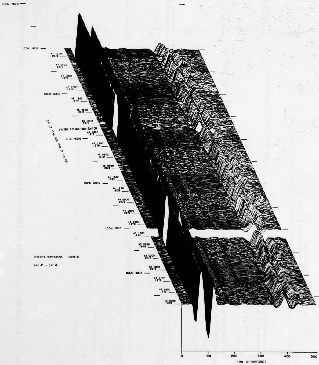
Figure 9. VLF/LF Reflectivity Data for the Polar Ionosphere, DAY 042 (11 Feb) - DAY 048 (17 Feb) 1979 (Cont) Part R. || Waveform Display
