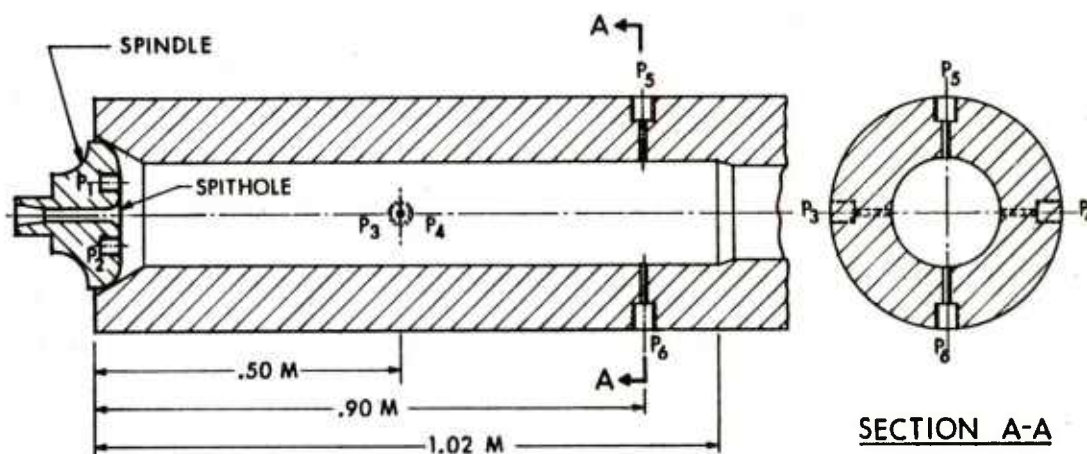
Figure 11. Locations of Pressure Taps in the Modified, M185 Cannon (Range 18)
