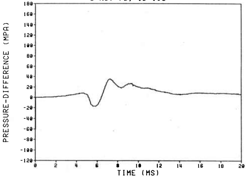
37-PERF M30A1 (SUBCALIBER CHARGE) 9 NOV 78; ID 103
