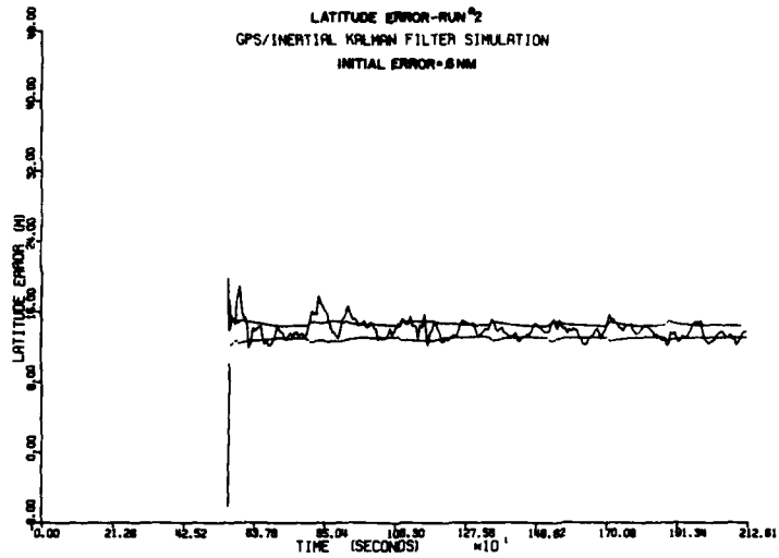
FIGURE 19 LONGITUDE ERROR-RUN #2 GPS/INERTIAL KALMAN FILTER SIMULATION INITIAL ERROR=5NM
