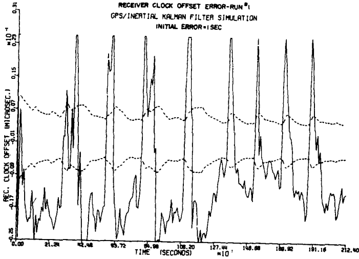
FIGURE 17 RECEIVER CLOCK DRIFT-RUN #1 GPS/INERTIAL KALMAN FILTER SIMULATION INITIAL ERROR=10^-8 SEC/SEC
