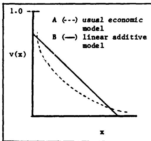
Fig 3.3 Value Functions
