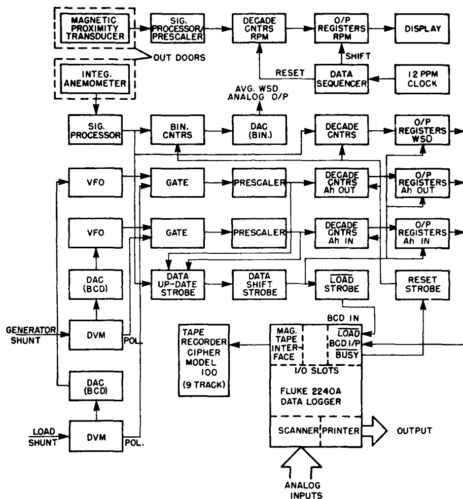
Fig. 18: Data acquisition system.
