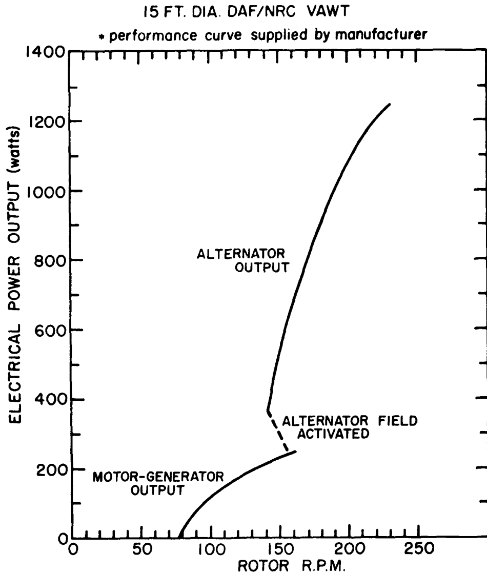
Fig. 7: VAWT power output v's rotor RPM.
