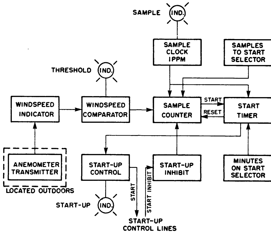
Fig. 17: Block diagram of the anemometer start-up control circuit.
