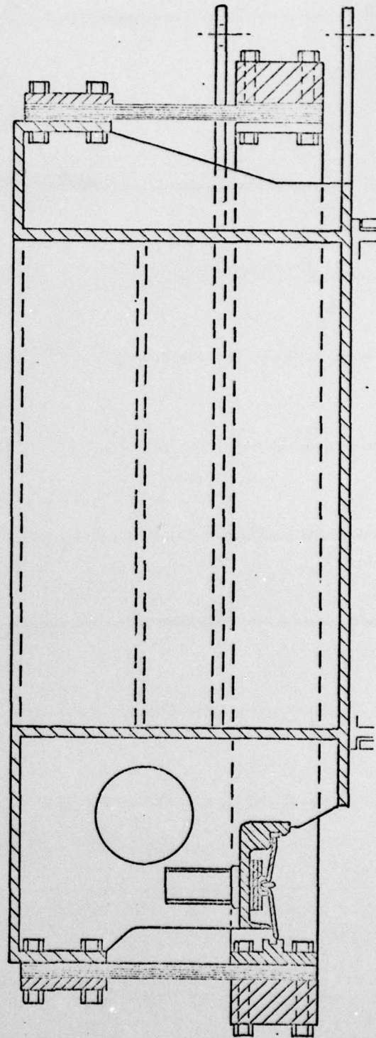
SECTIONAL ELEVATION (Scale \frac{2}{5} full size)
