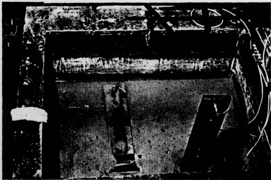
PLATE 14 - Towers on wet sand, after foundation failure
