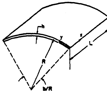
Fig. 1 Shell geometry.
