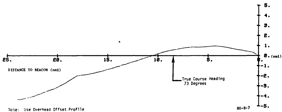
FIGURE 7. INITIAL SEGMENT OF AN APPROACH FLOWN ON NOVEMBER 3, 1978
