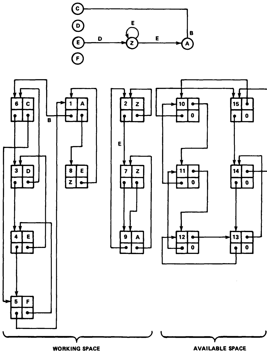
Figure 36 - Example of Graph Structure and Associated Internal GIRS Pointer Graph
