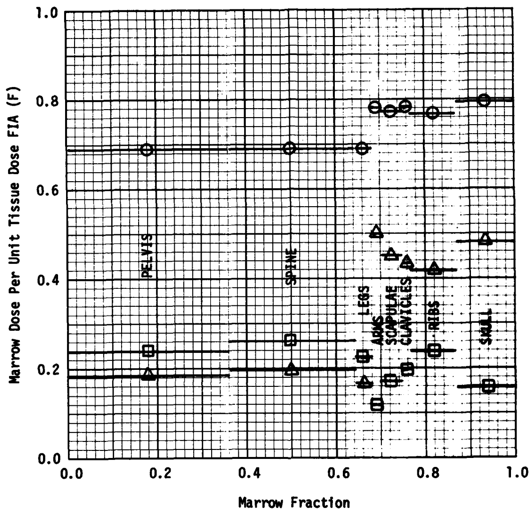
Figure IV-10. Marrow Dose Distribution Per Unit Incident Isotropic Fluence from a Boosted Fission Implosion Weapon (5 kt, Ground Range = 1.2 km), \circ : F_{\gamma-\gamma} , \triangle : F_{n-n} , \square : F_{n-\gamma} .
