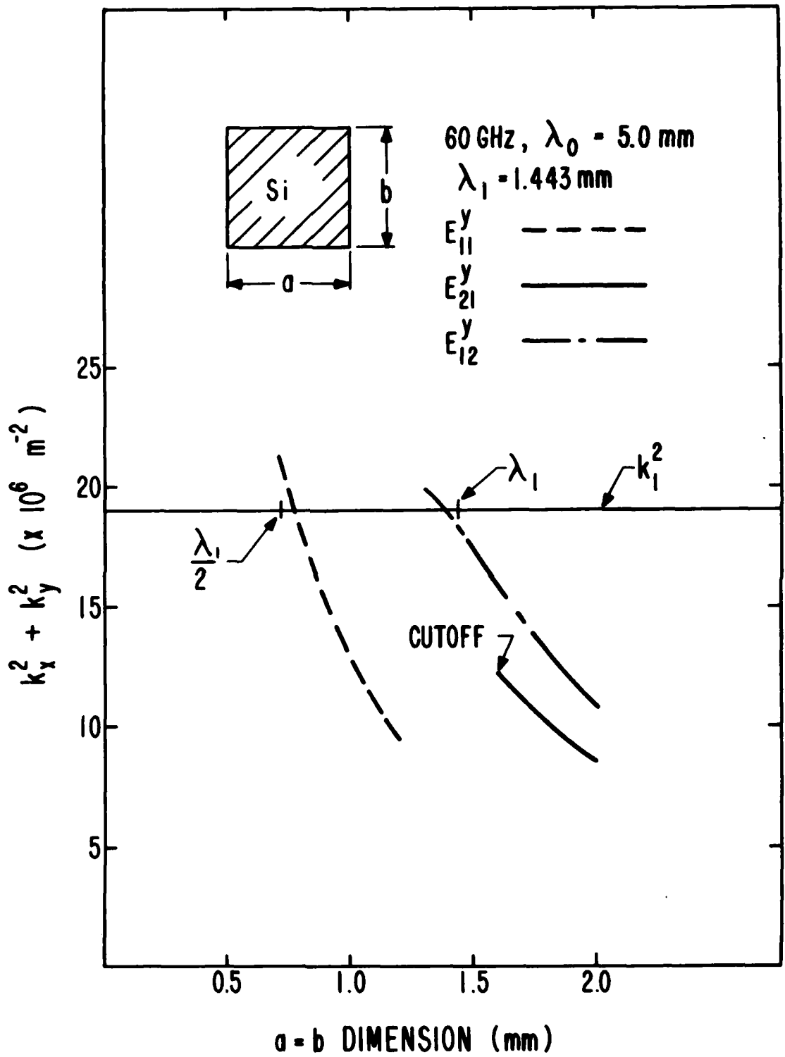
Figure 1 Minimum and Maximum Waveguide Dimensions. 60 GHz
