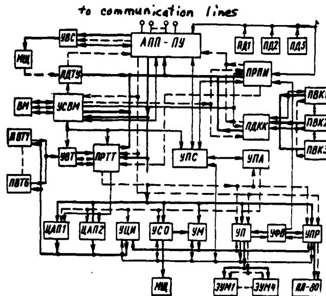
Figure 1. Structural diagram of the PU equipment: ПМЦ - mimic panel; ПД1 - ПД3 - dispatcher panels; ВМ - computer; АПП-ПУ - equipment of receiving-transmitting point of control; УВС - device for reproduction of signalization; ПДТУ - telecontrol command transmitter; ПРПИ - receiver of periodic informatio of telemeasurements of integrated values of parameters and statistical information (TII and SI); ПВК1-ПВК3 - panels for input of coded commands; ПДКК - transmitter of coded commands (TR, TsS, SK); ПРТТ - receiver of current telemeasurements; ПВТ1-ПВТ6 - panels for selection of current telemeasurements; УВТ - device for selection of current telemeasurements; ЦАП1, ЦАП2 - digital-analog converters; УСО - device for signalization of deviations of TIT parameters from assigned settings; УПА - program-address device; УФВ - time formation device; УП - reading device; ЗУИ1-ЗУИ4 - electrocontrol reading devices; УПР - perforation device; ПЛ-80 - tape puncher; УЦИ - digital indication device; УПС - program-synchronizing device; УСВМ - device for conjugation with the computer; УМ - scaling device.
