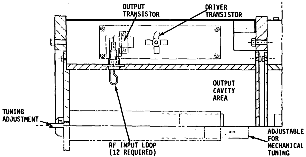
FIGURE 2-22. LONGITUDINAL SECTIONAL VIEW - OUTPUT RESONATOR
