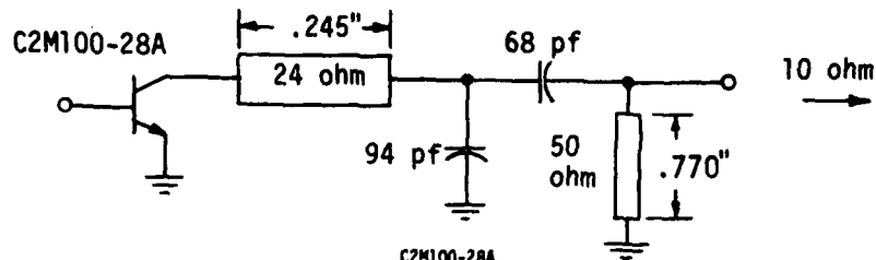
C2M100-28A OUTPUT IMPEDANCE (CALCULATED)
