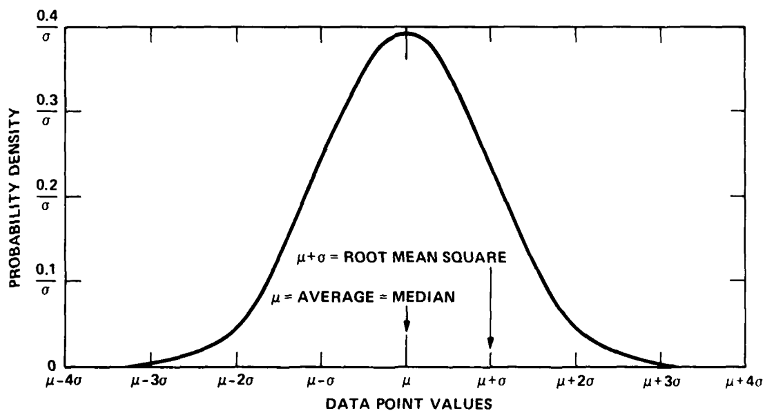
Figure B.2 - Gaussian Distribution
