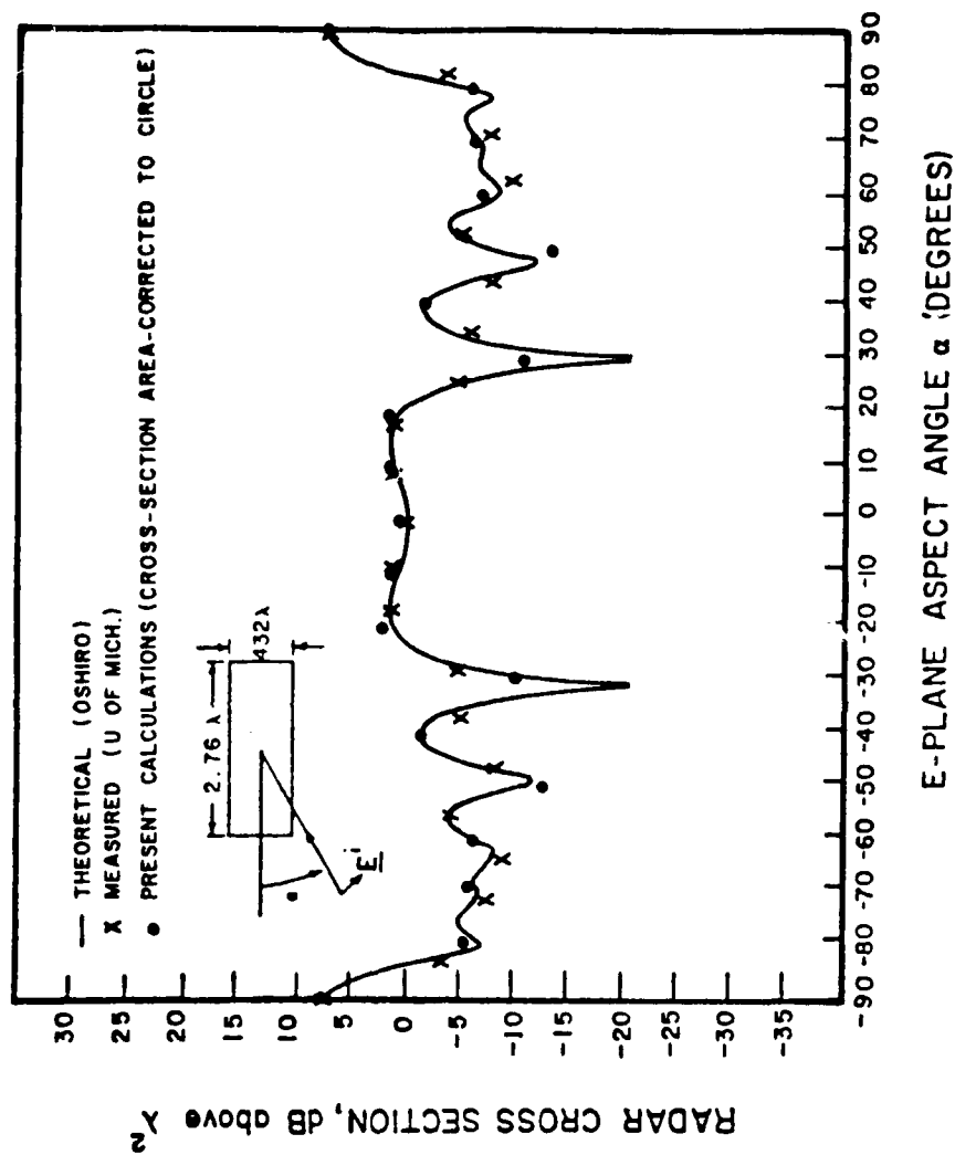
Figure 12. Backscattering cross section of a finite circular cylinder in the E-plane.
