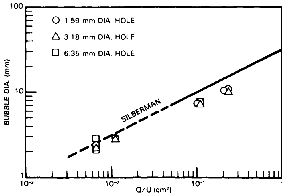
Figure 10. Mean bubble diameter as a function of Q/U : U = \text{constant} .
