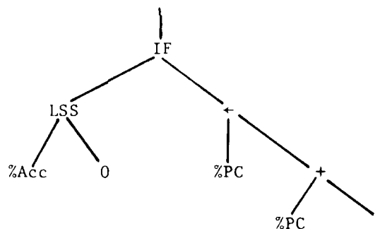
Figure 4.14 M-op Matching
