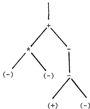
Figure 4.6 ORD Example Input
