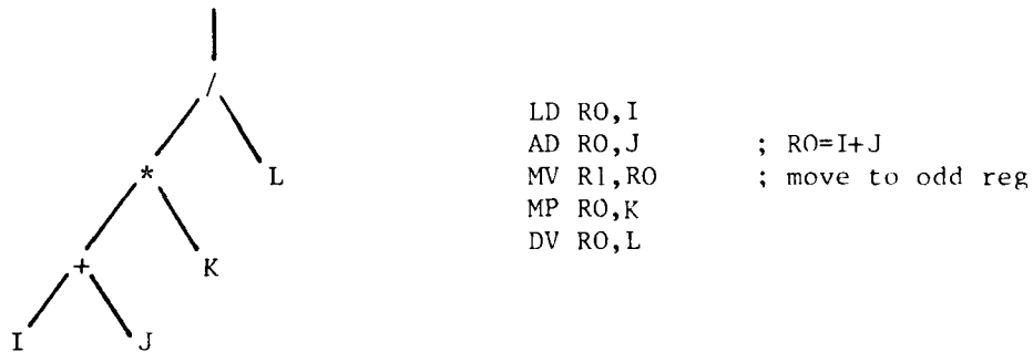
Figure 4.8 Register Preference Example
