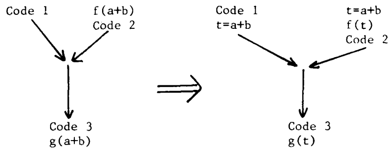
Figure 3.2 Rho Motion Optimization
