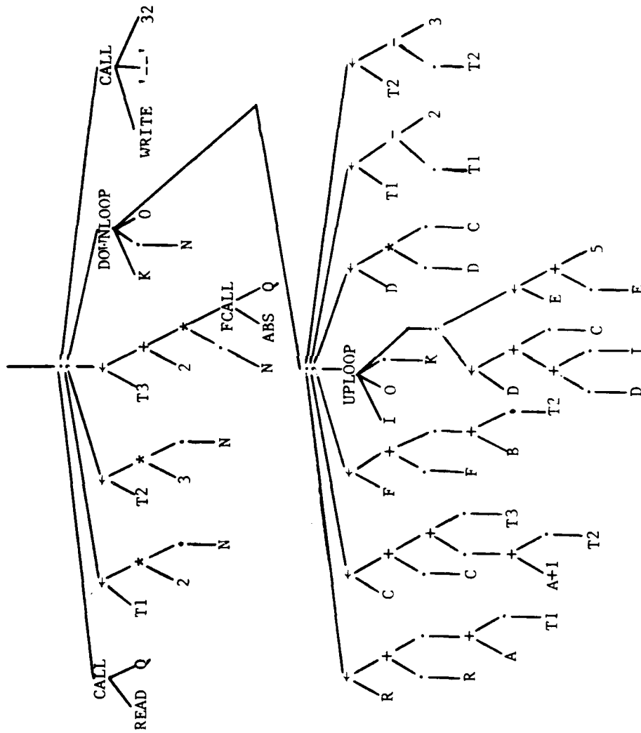
Figure 6.6 - Optimized Tree
