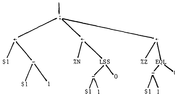
Figure 4.13 LISP notation
