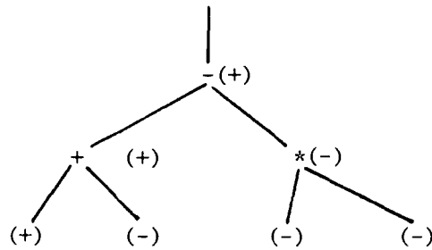
Figure 4.7 ORD Example Output
