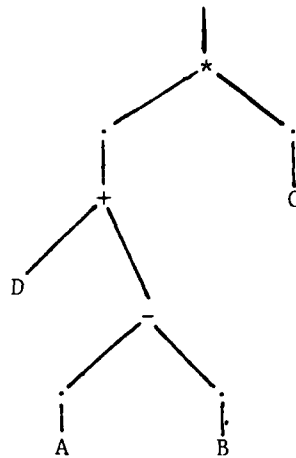
Figure 4.9 Addressing Mode Example
