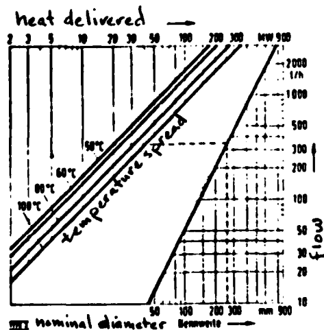
Figure 3. Determination of nominal pipe diameter, as a function of heat capacity at a water flow rate of 1.8 m/s
