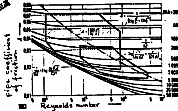
Figure 2. Flow domains for water networks and district heating system networks cold water ///// hot water XXXXXX
