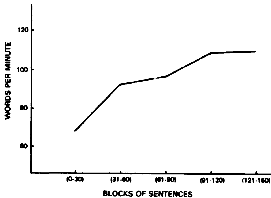
Figure 10. Computer-assisted reading.
