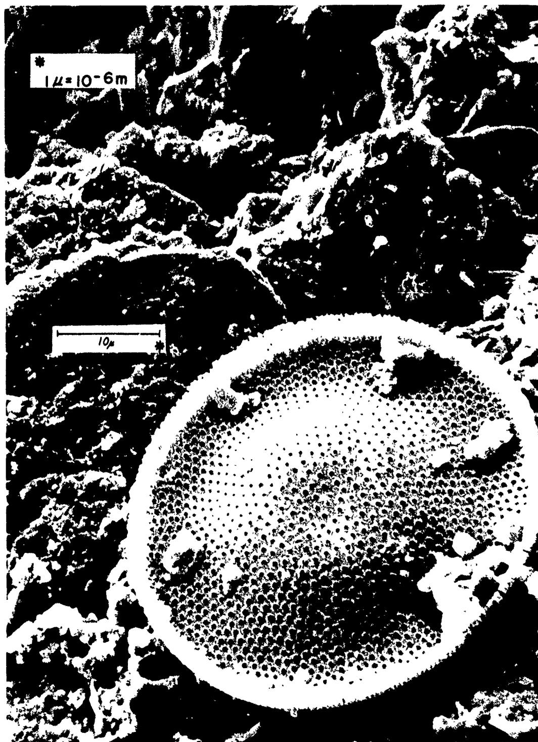
Scanning Electron Micrograph (2420x) of Coscinodiscus species of diatom frustule in Marcus Hook shoal sediments. This diatom variety is more abundant in this shoal than at other locations in the estuary.
