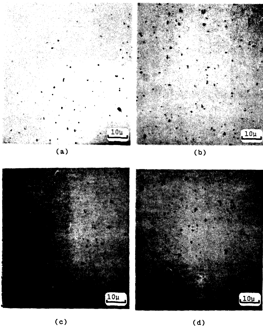
Figure 9. Photomicrographs taken of the "as-polished" specimen subjected to the original two-pass weld only. The locations represented are the interface (a), approximately 6 mm (b), 18 mm (c) and 27 mm (d) from the interface. (100X)
