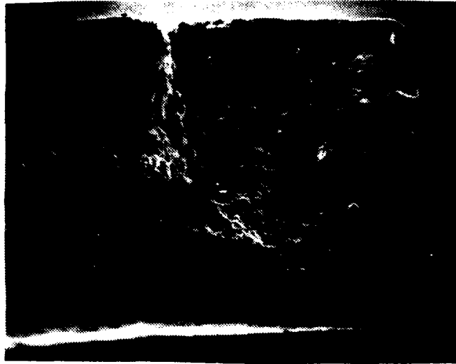
Figure 18. Observation of the fracture surface of a sample from the unwelded original. (25X). The fatigue crack seems to have begun at the free surface of the material and propagated inward.
