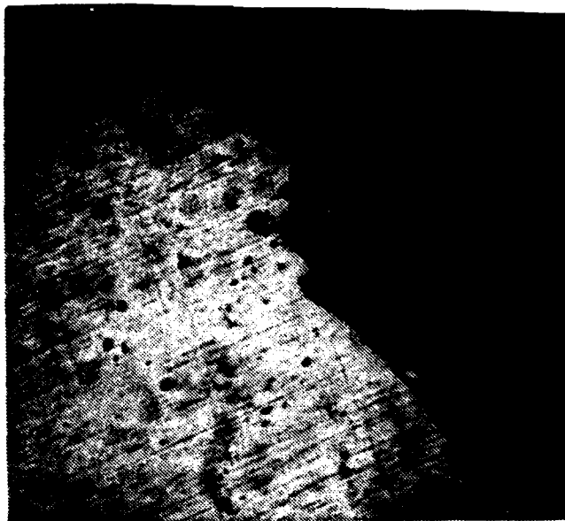
Figure 21. Observation of transverse section of the fracture surface of a 14 weld repaired sample. (100X). Note the porosity at or near the fracture surface. This observation along with that in Figure 12 indicate that the fatigue fracture in all welded samples was probably initiated at porosity located in the weld filler material.
