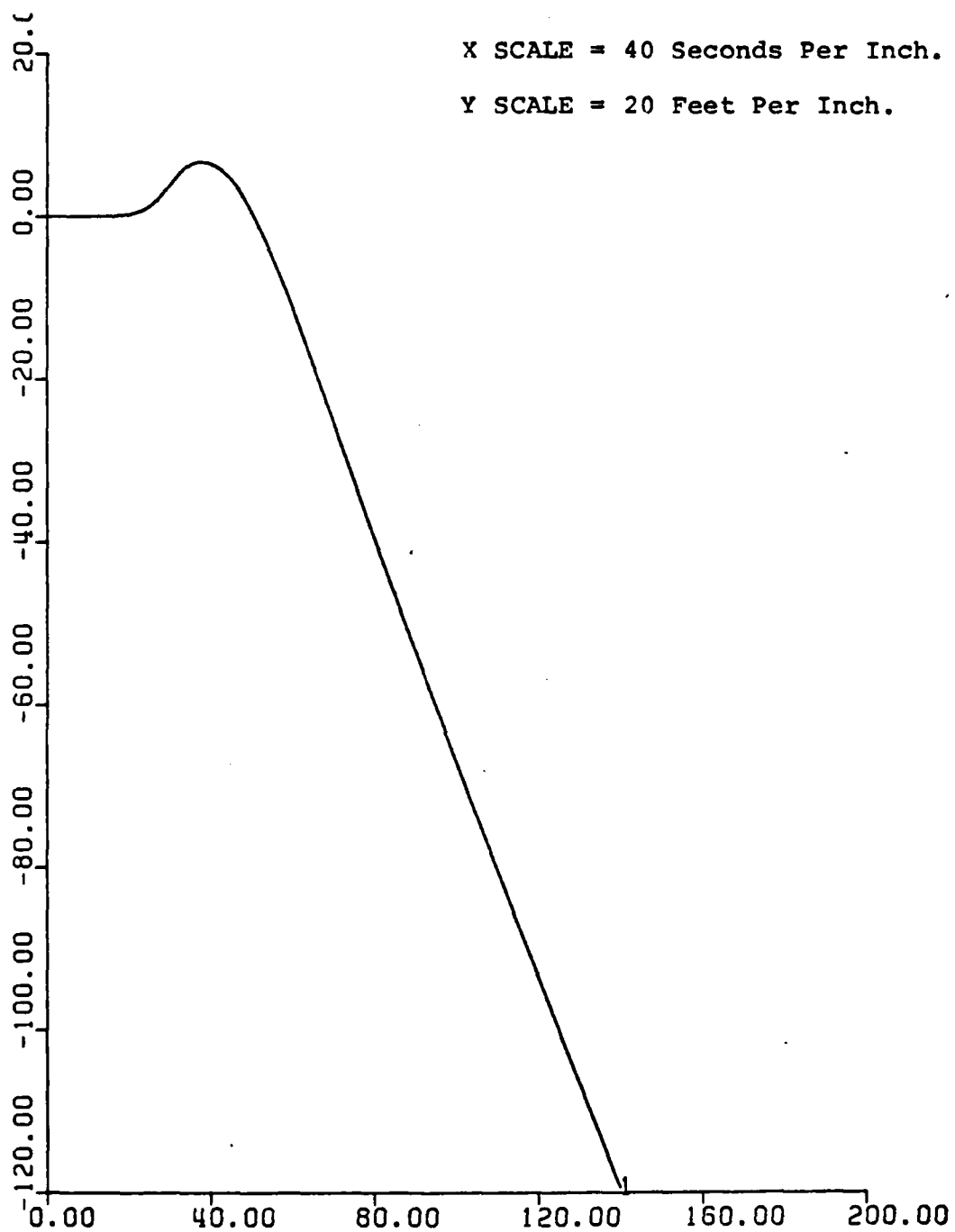
Figure 14. Depth vs. Time. With No Controller. UCK = 12 Knots. Rudder Ordered = 35^{\circ} .
