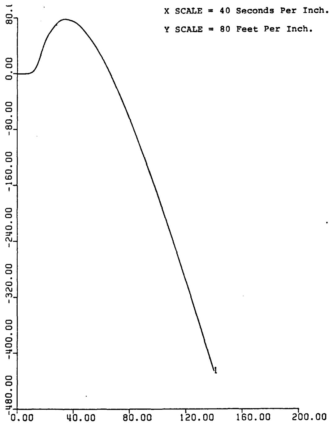
Figure 3. Depth vs. Time. With No Controller UCK = 24 Knots. Rudder Ordered = 35^{\circ} .
