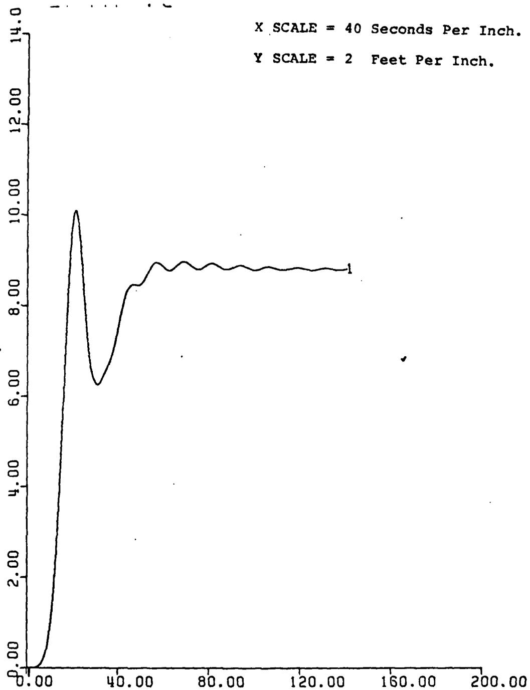
Figure 48. Depth vs. Time. With Depth-Pitch Controller. UCK = 18 Knots. Rudder Ordered = 35^{\circ} .
