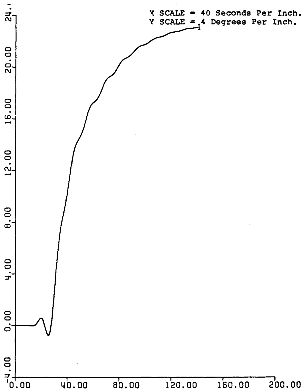
Figure 9. Pitch vs. Time. With No Controller. UCK = 18 Knots. Rudder Ordered = 35^{\circ} .
