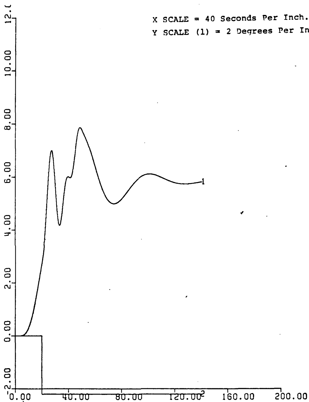
Figure 117.1. Pitch vs. Time. Roll Stability Step Test. UCK = 12 Knots. Rudder Ordered = 35^{\circ} . .2. Disturbance Moment vs. Time. ( 1.1028 \times 10^7 ft-lb.).
