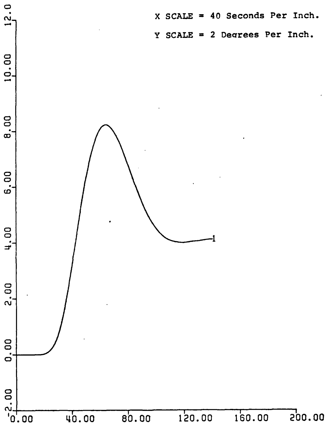
Figure 21. Pitch vs. Time. With No Controller. UCK = 6 Knots. Rudder Ordered = 35^{\circ} .
