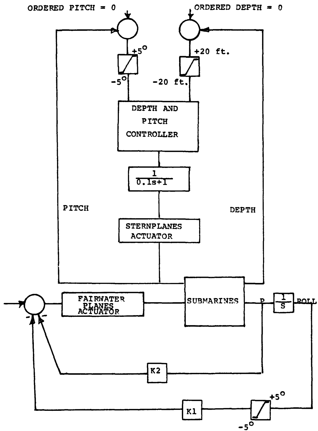
Figure 72. Complete Depth-Pitch-Roll Controller (Final Scheme)
