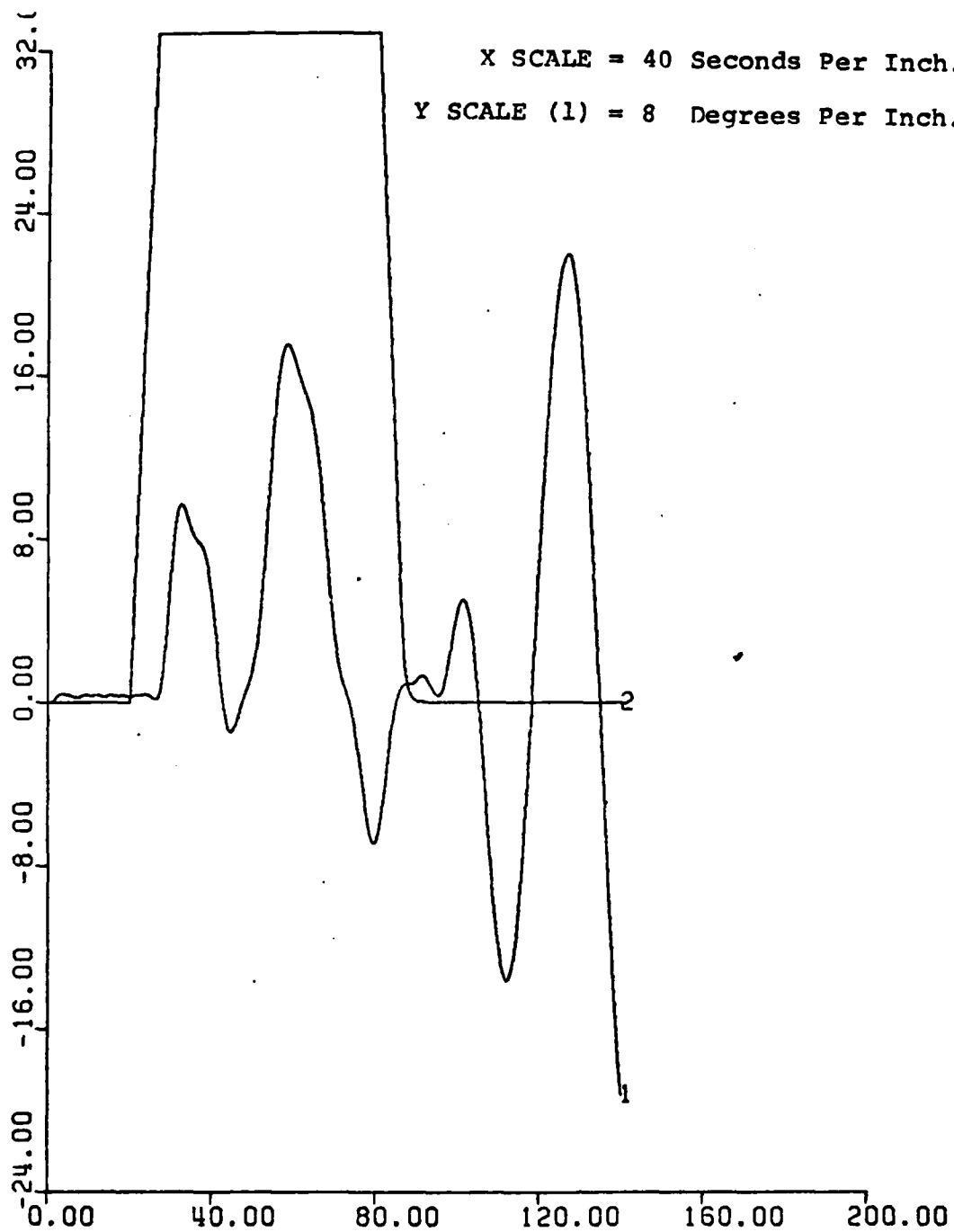
Figure 68.1. Pitch vs. Time. K_1 = 3 , K_2 = 10 . UCK = 24 Knots. Initial Roll Angle = -20^\circ .
