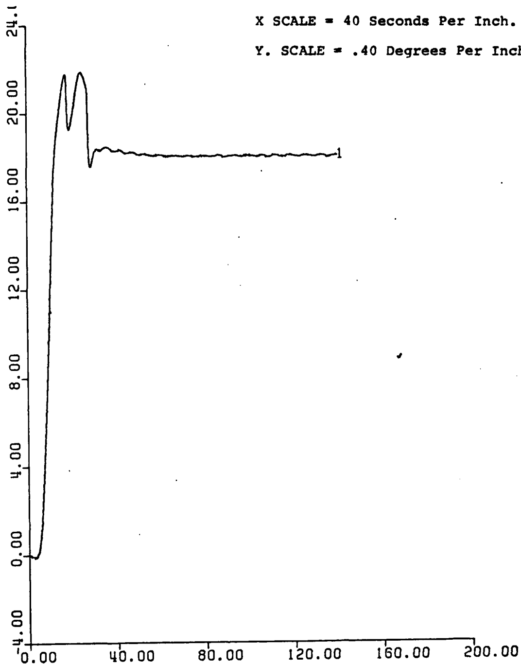
Figure 61. Sternplane Angle vs. Time. K1 = 3 . UCK = 24 Knots. Rudder Ordered = 35^\circ . Initial Roll Angle = 0^\circ .
