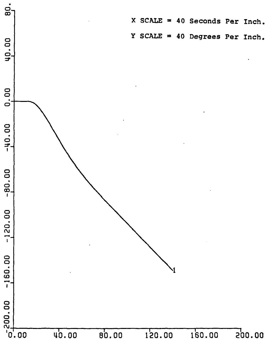
Figure 24. Yaw vs. Time. With No Controller. UCK = 6 Knots. Rudder Ordered = 35^{\circ} .
