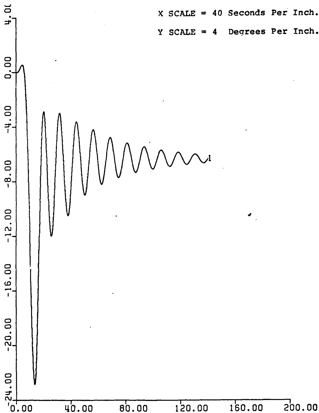
Figure 50. Roll vs. Time. With Depth-Pitch Controller, UCK = 18 Knots. Rudder Ordered = 35^{\circ} .
