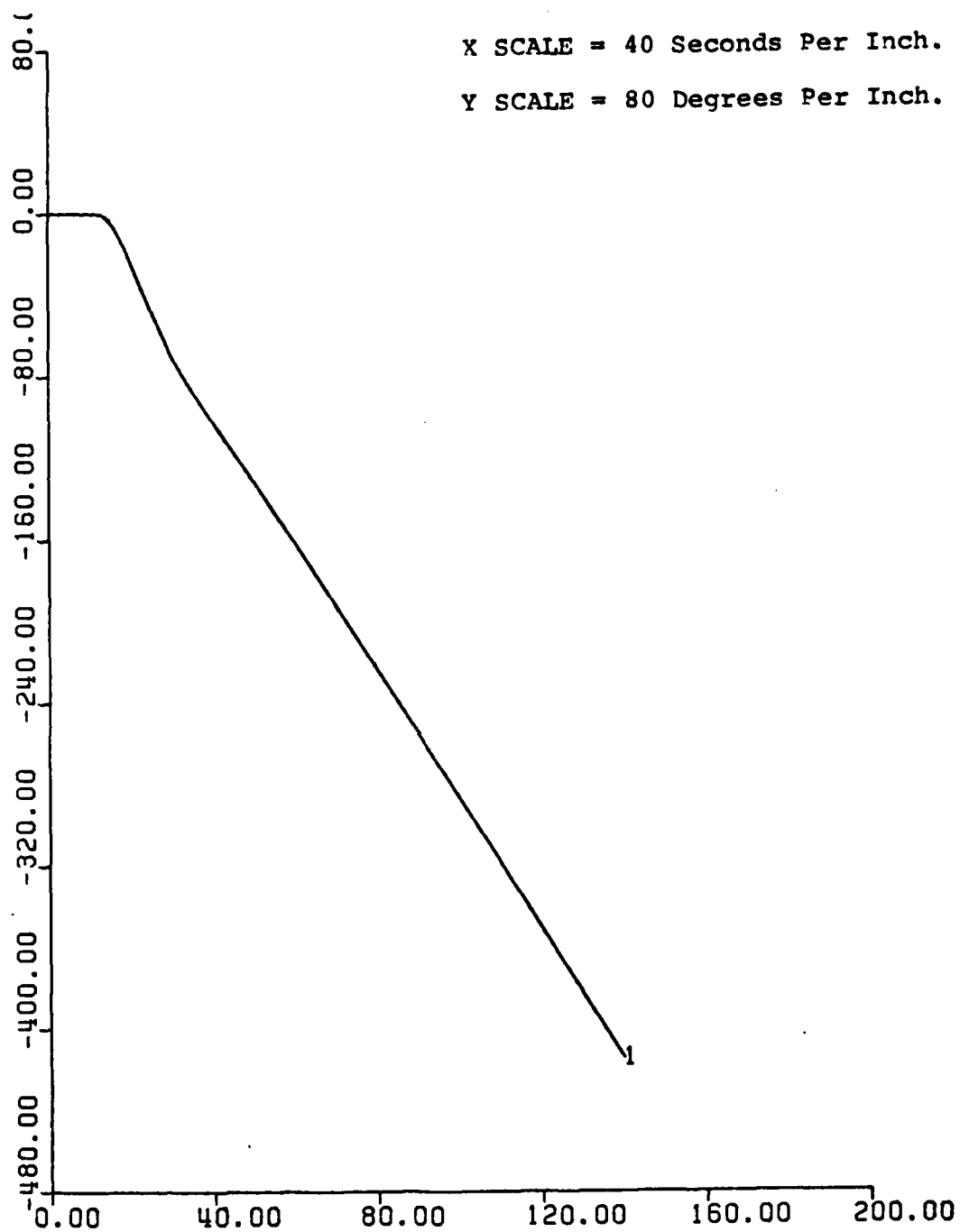
Figure 12. Yaw vs. Time. With No Controller. UCK = 18 Knots. Rudder Ordered = 35^{\circ} .
