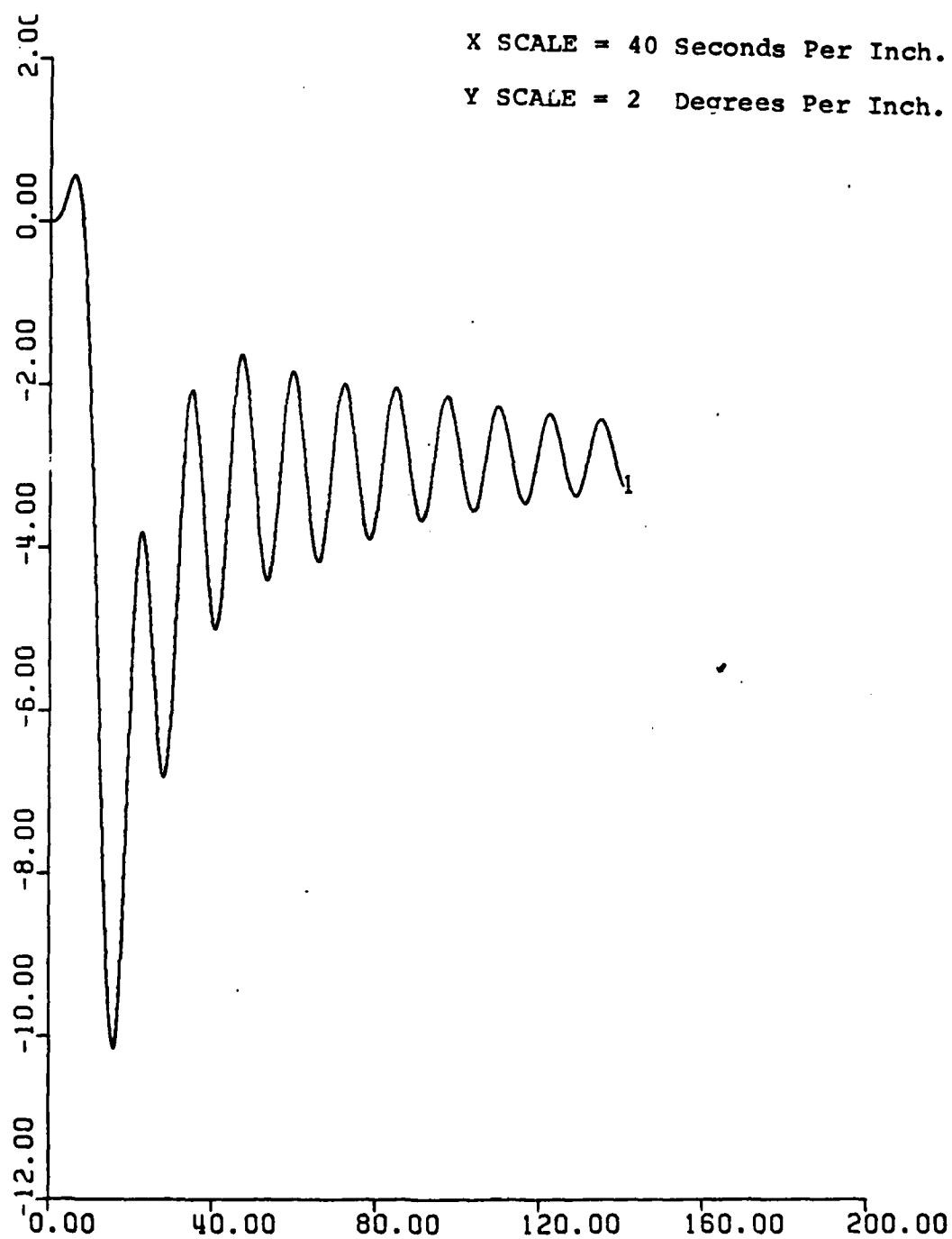
Figure 46. Roll vs. Time. With Depth-Pitch Controller. UCK = 12 Knots. Rudder Ordered = 35^{\circ} .
