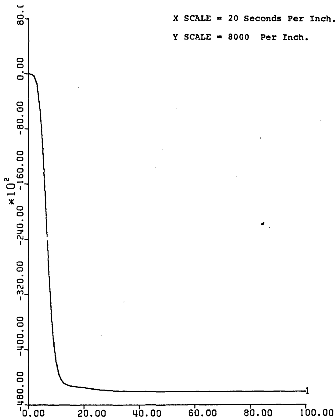
Figure 33. K24 vs. Time. UCK = 15 Knots. D = 8000, A = 0, E = 10, B = 0, C = 100.
