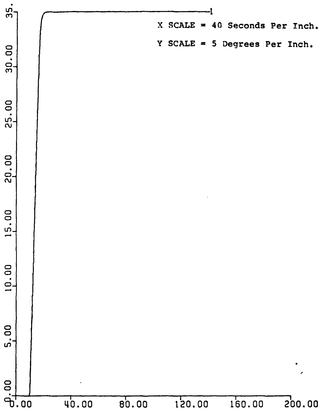
Figure 19. Rudder Response vs. Time. With No Controller. UCK = 12 Knots. Rudder Ordered = 35^{\circ} .
