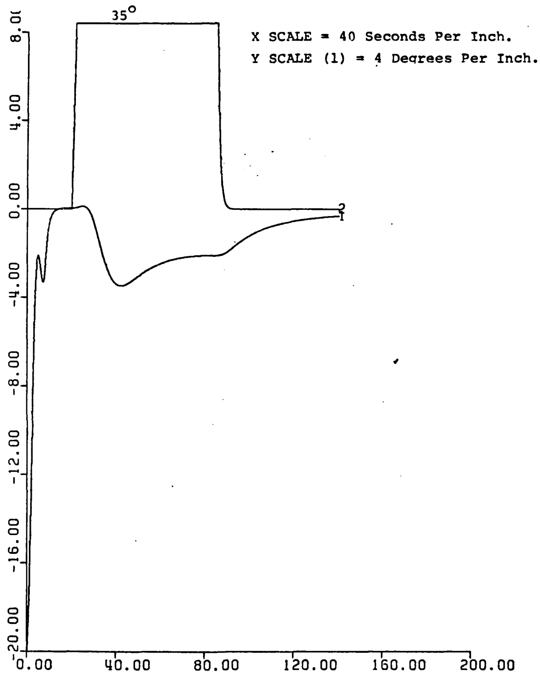
Figure 85.1. Roll vs. Time. Final Result With Roll Error Limiter K1 = 3, K2 = 10. UCK = 12 Knots. Initial Roll Angle = -20^{\circ} .
