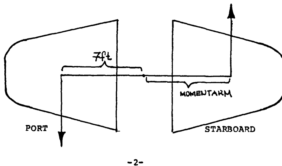
Figure 56.1. Positive Direction Of Differentially Deflected Sailplanes. .2. Negative Direction Of Rolling Moment.
