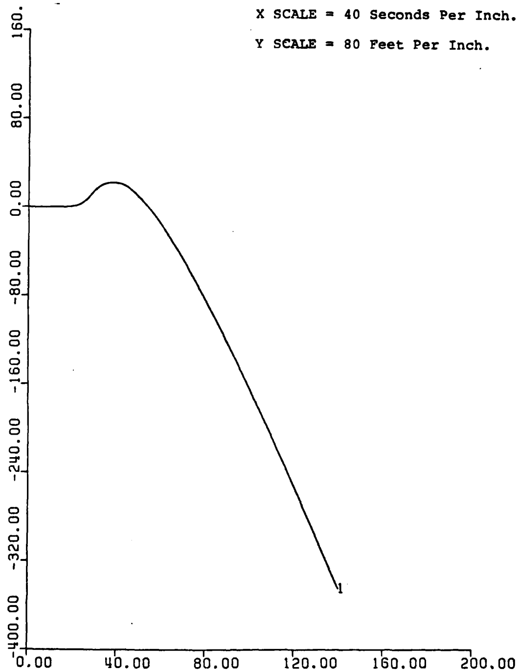
Figure 8. Depth vs. Time. With No Controller. UCK = 18 Knots. Rudder Ordered = 35^{\circ} .
