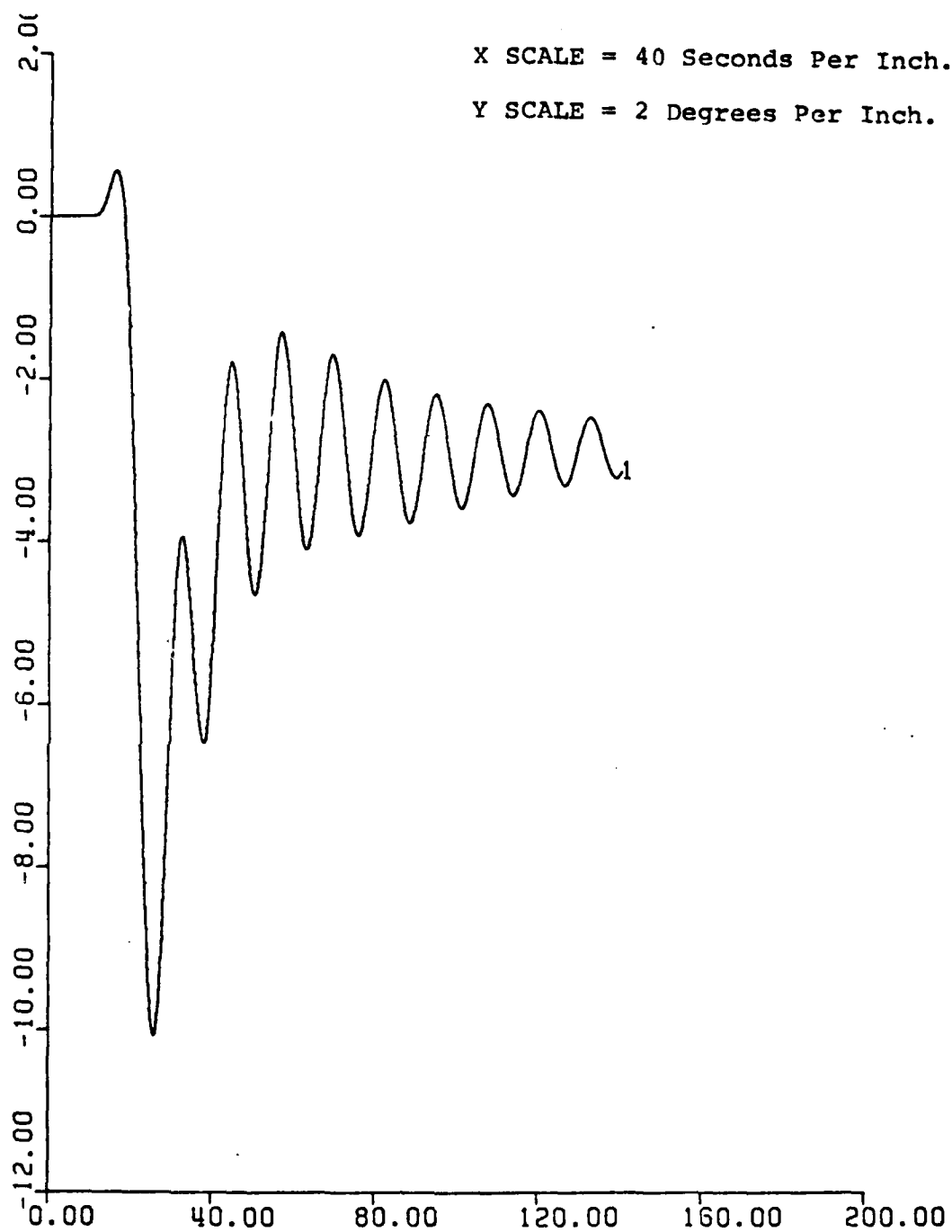
Figure 16. Roll vs. Time. With No Controller. UCK = 12 Knots. Rudder Ordered = 35^{\circ} .
