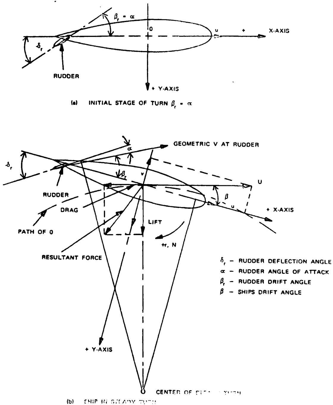
Figure 1. Hydrodynamic Forces In A Turn. (After Reference 4)
