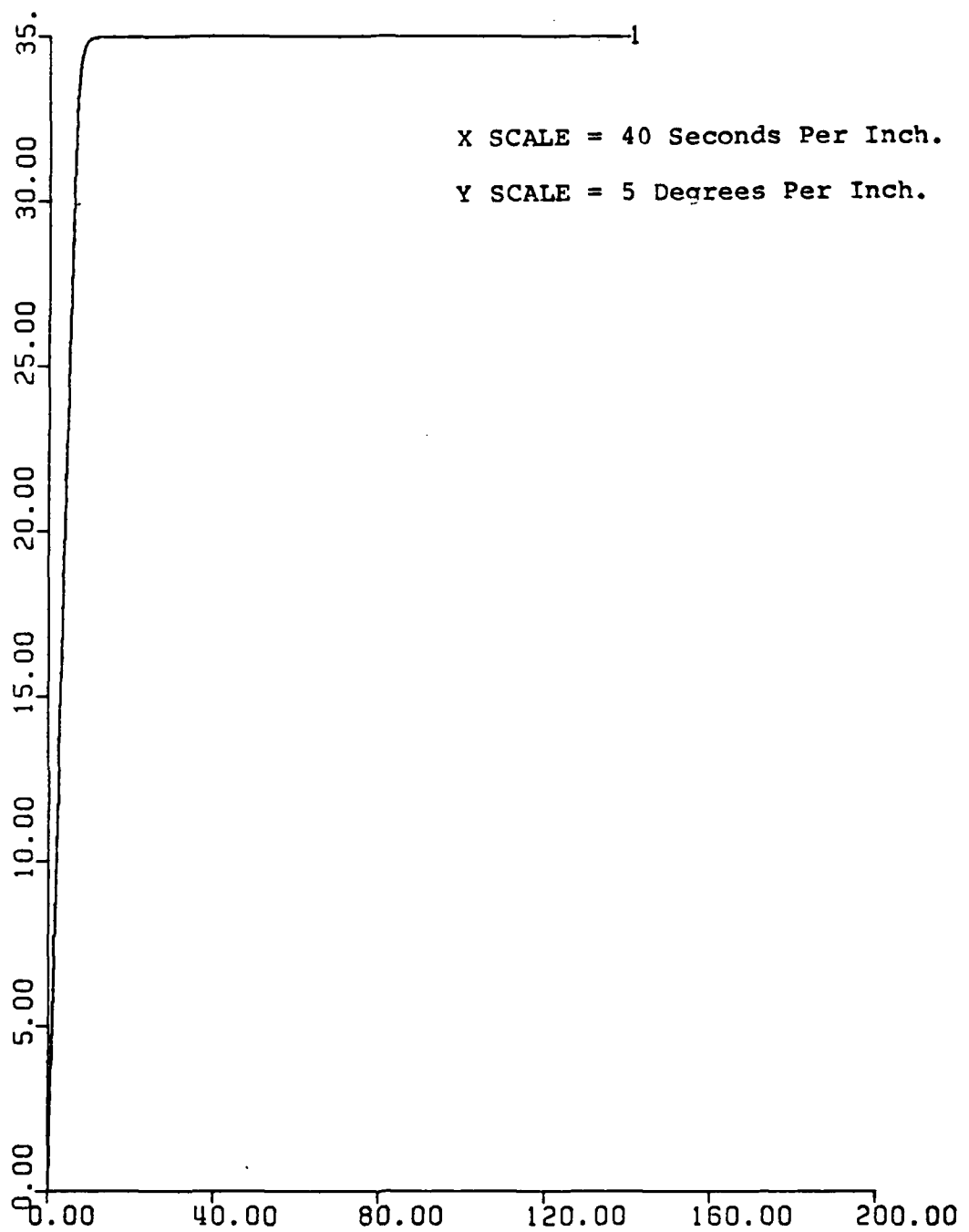
Figure 6. Rudder Response vs. Time. With No Controller. UCK = 24 Knots. Rudder Ordered = 35^{\circ} .
