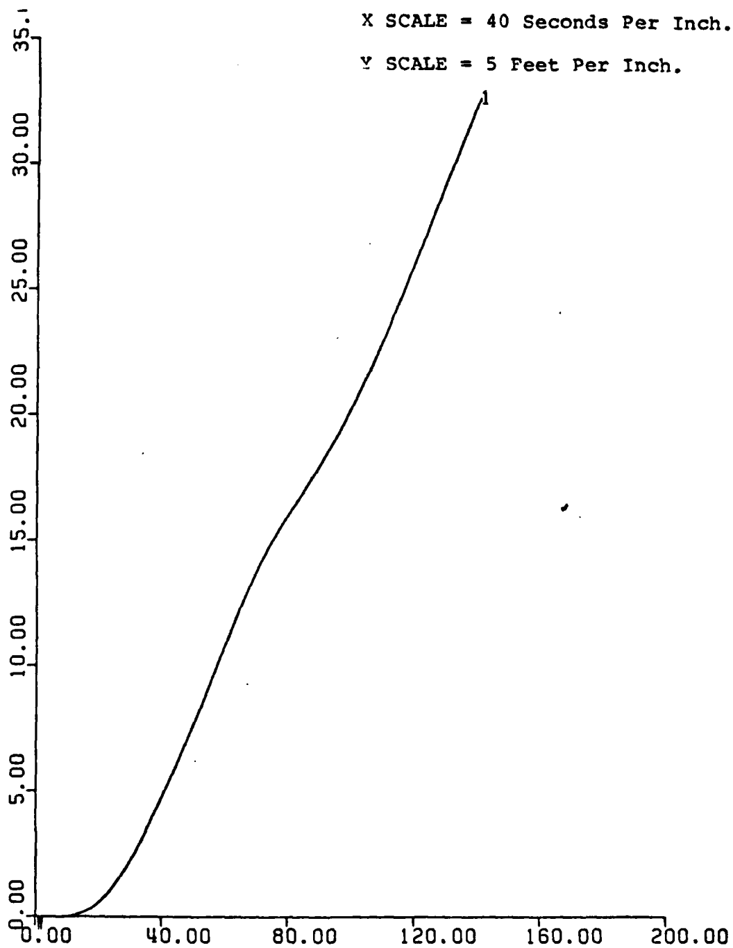
Figure 40. Depth vs. Time. With Depth-Pitch Controller. UCK = 6 Knots. Rudder Ordered = 35^{\circ} .
