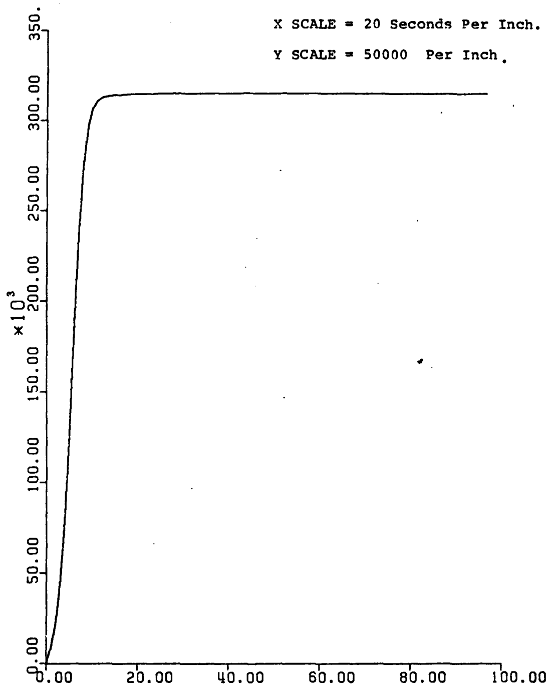
Figure 34. K33 vs. Time. UCK = 15 Knots. D = 8000, A = 0, E = 10, B = 0, C = 100.
