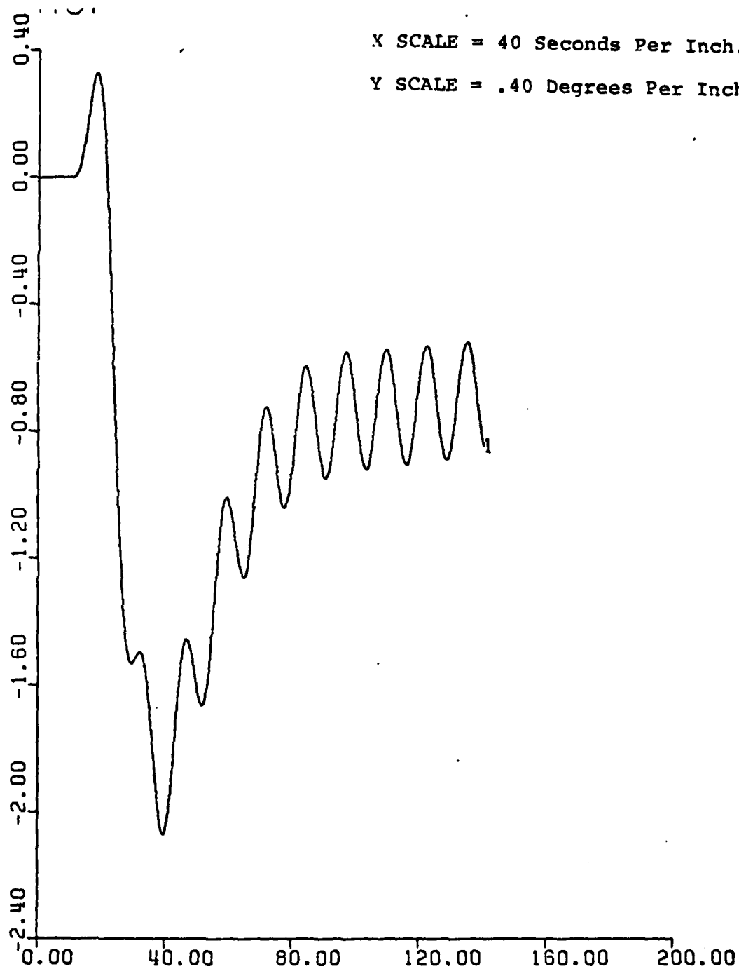
Figure 22. Roll vs. Time. With No Controller. UCK = 6 Knots. Rudder Ordered = 35^{\circ} .
