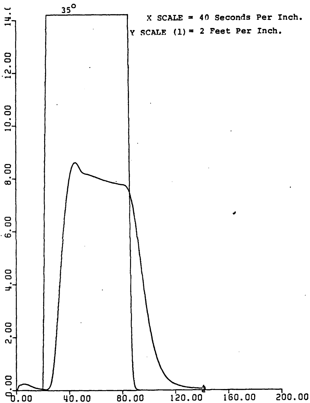
Figure 73.1. Depth vs. Time. Final Result With Roll Error Limiter. K_1 = 3 , K_2 = 10 . UCK = 24 Knots. Initial Roll Angle = -20^\circ . .2. Rudder Response vs. Time. (Pudder Ordered = 35^\circ ).
