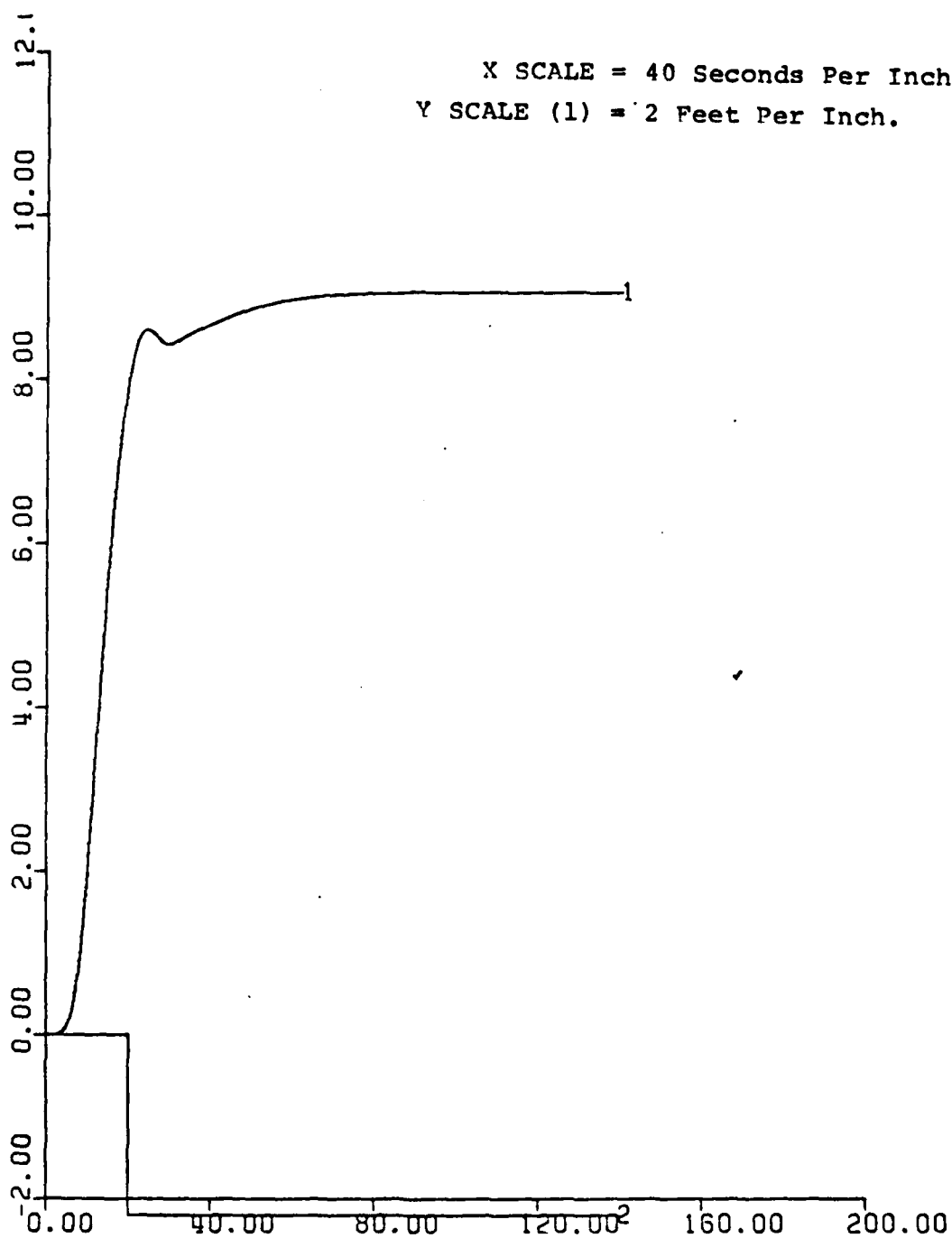
Figure 106.1. Depth vs. Time. Roll Stability Step Test.
