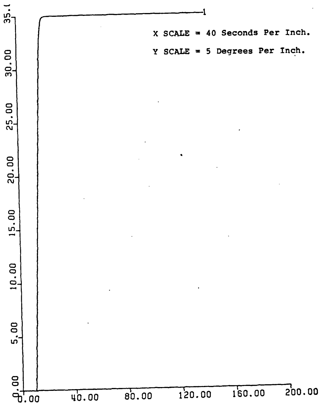
Figure 25. Rudder Response vs. Time. With No Controller. UCK = 6 Knots. Rudder Ordered = 35^{\circ} .
