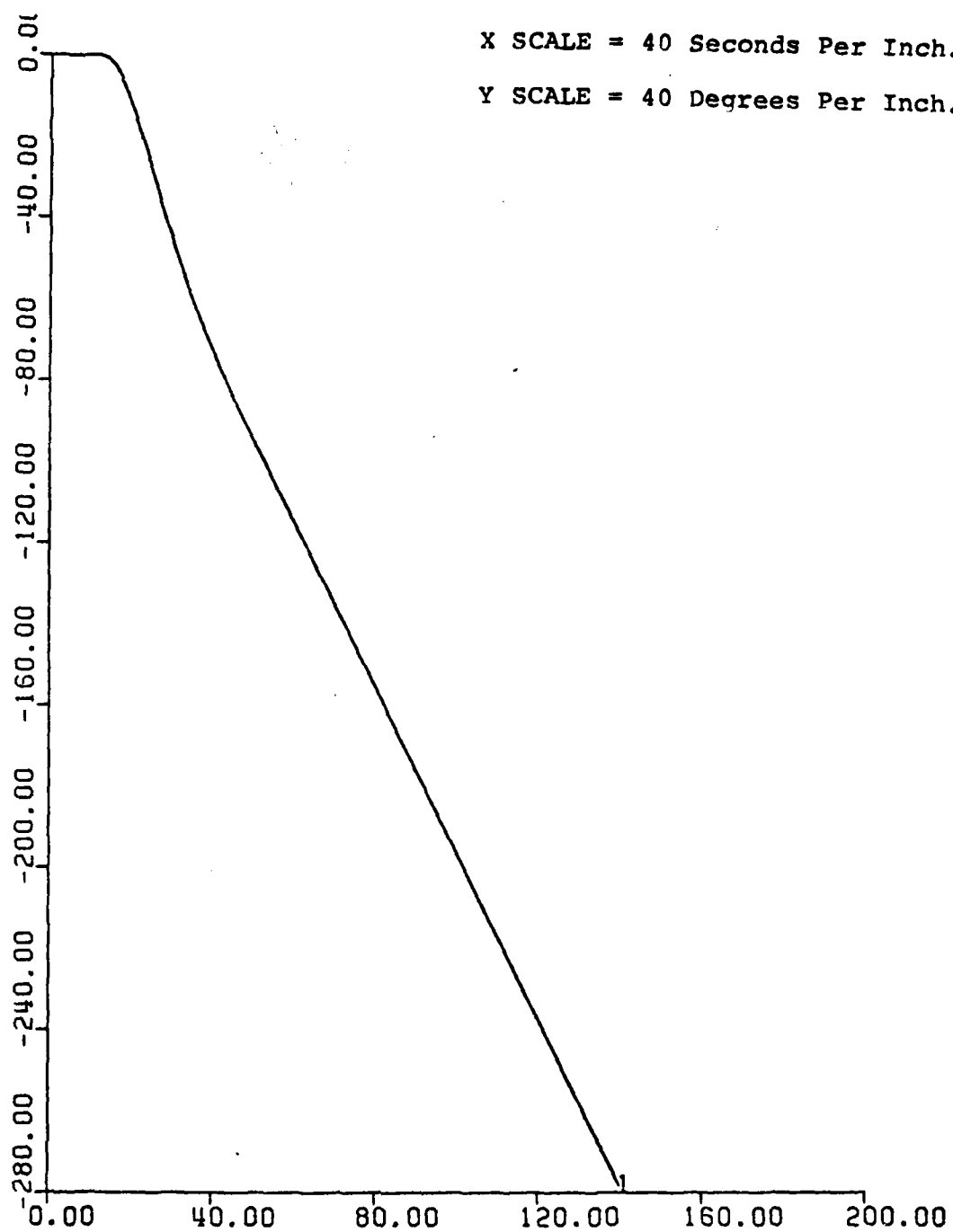
Figure 18. Yaw vs. Time. With No Controller. UCK = 12 Knots. Rudder Ordered = 35^{\circ} .
