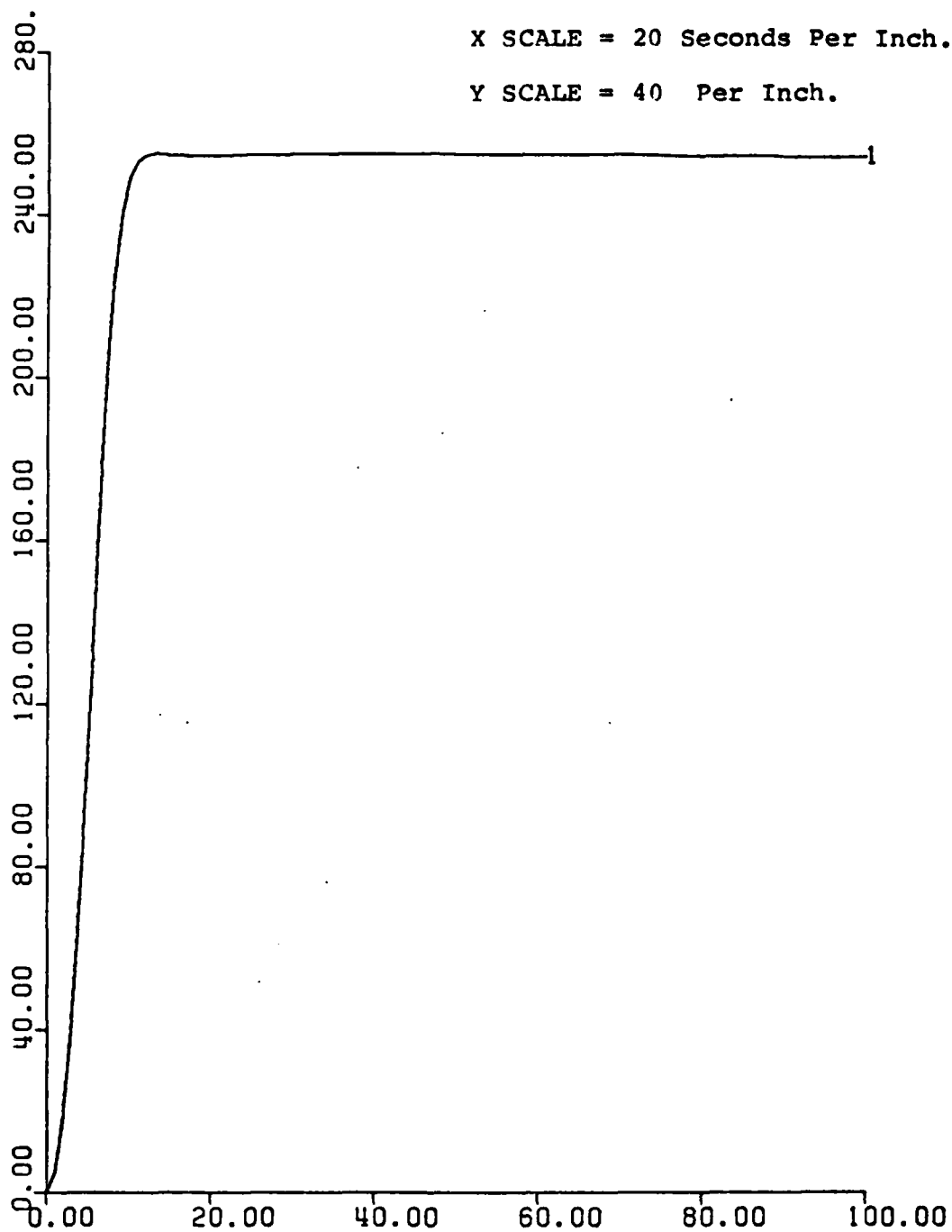
Figure 28. K12 vs. Time. UCK = 15 Knots.
