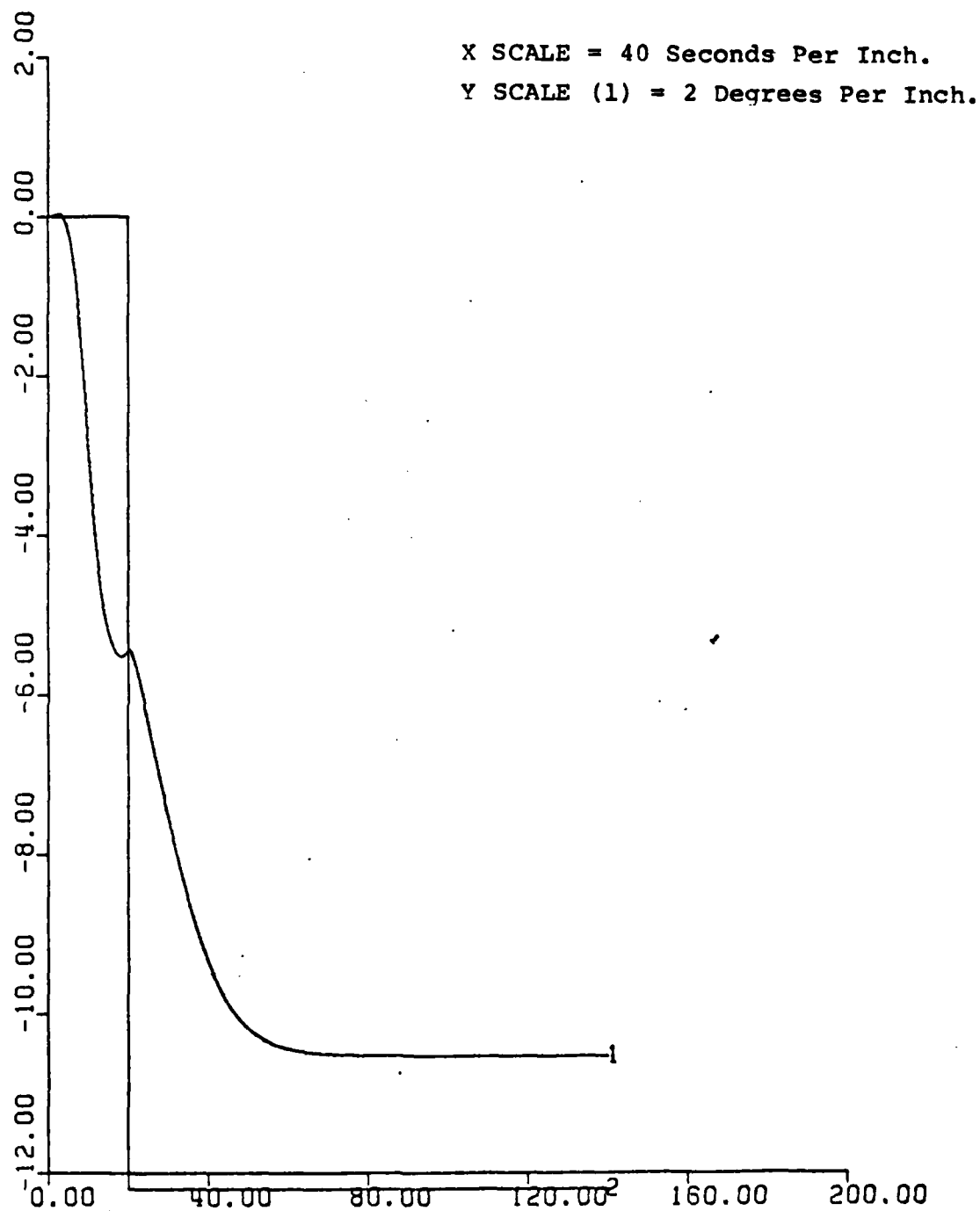
Figure 108.1. Roll vs. Time. Roll Stability Step Test. UCK = 24 Knots. Rudder Ordered = 35^{\circ} .
