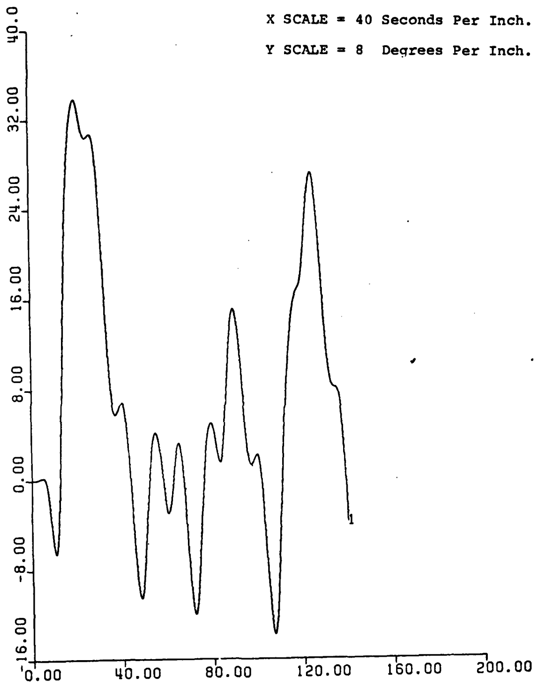
Figure 64. Pitch vs. Time. K1 = 3 . UCK = 24 Knots. Rudder Ordered = 35^\circ . Initial Roll Angle = -5^\circ .
