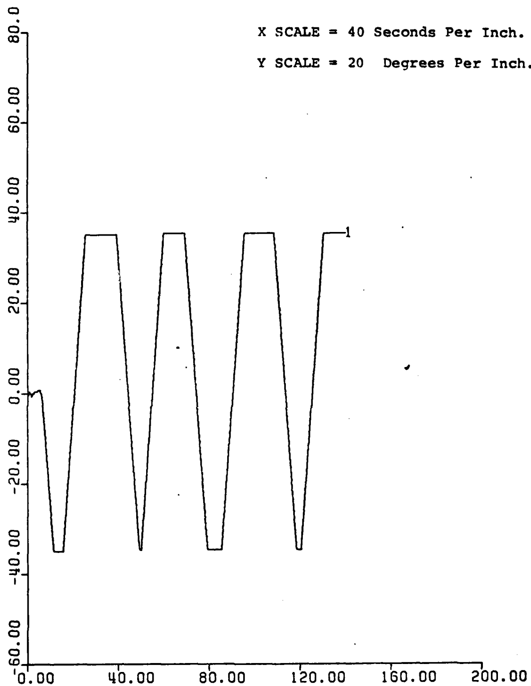
Figure 55. Sternplane Angle vs. Time. With Depth-Pitch Controller. UCK = 24 Knots. Rudder Ordered = 35^{\circ} .
