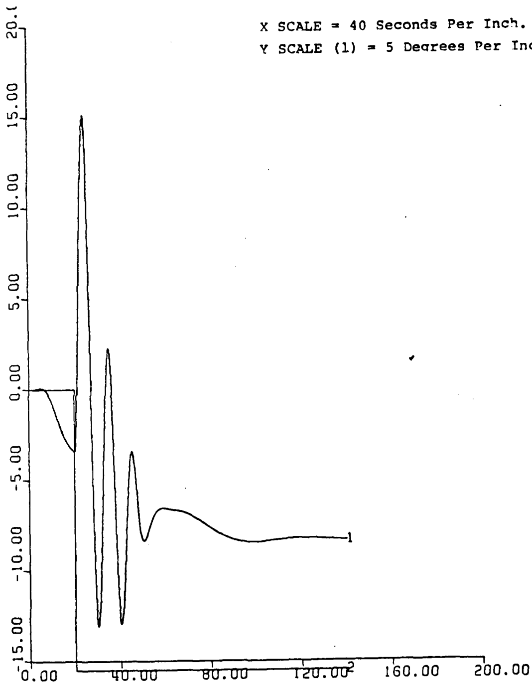
Figure 118.1. Roll vs. Time. Roll Stability Step Test.
