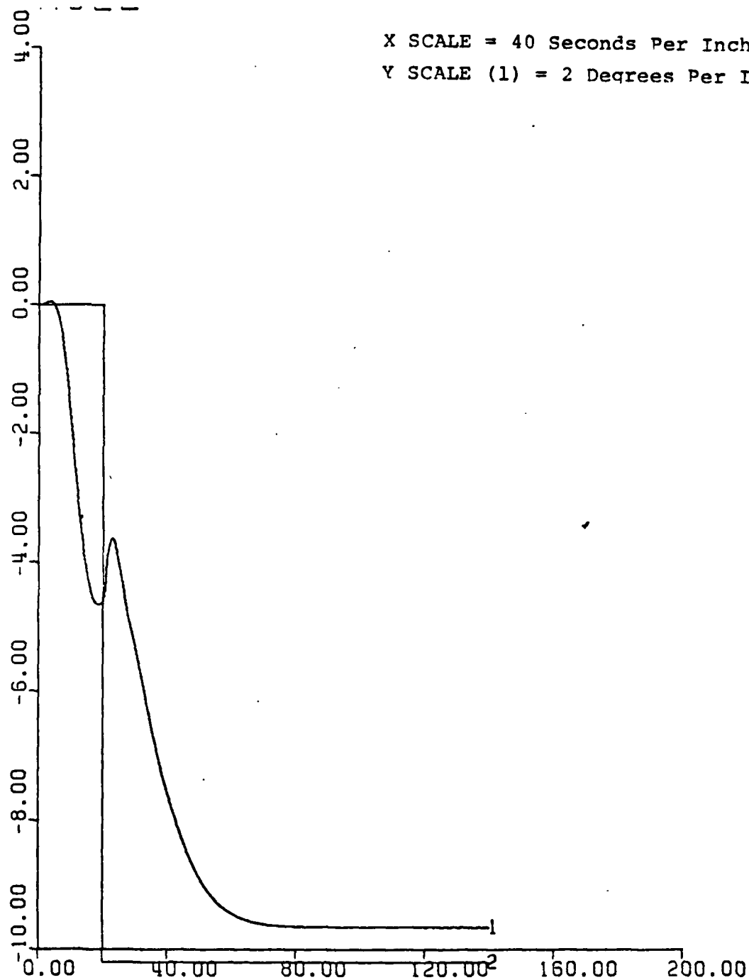
Figure 113.1. Roll vs. Time. Roll Stability Step Test.
