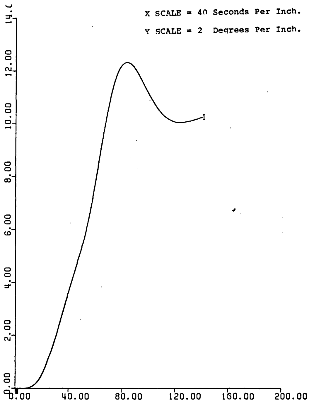
Figure 41. Pitch vs. Time. With Depth-Pitch Controller. UCK = 6 Knots. Rudder Ordered = 35^{\circ} .
