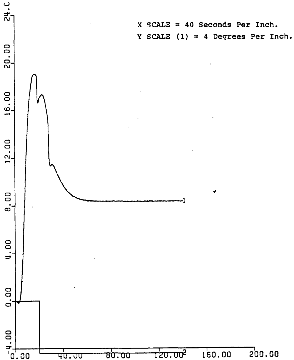
Figure 109.1. Sternplane Angle vs. Time. Roll Stability Step Test. UCK = 24 Knots. Rudder Ordered = 35^{\circ} . .2. Disturbance Moment vs. Time ( 1.1028 \times 10^7 ft-lb.).
