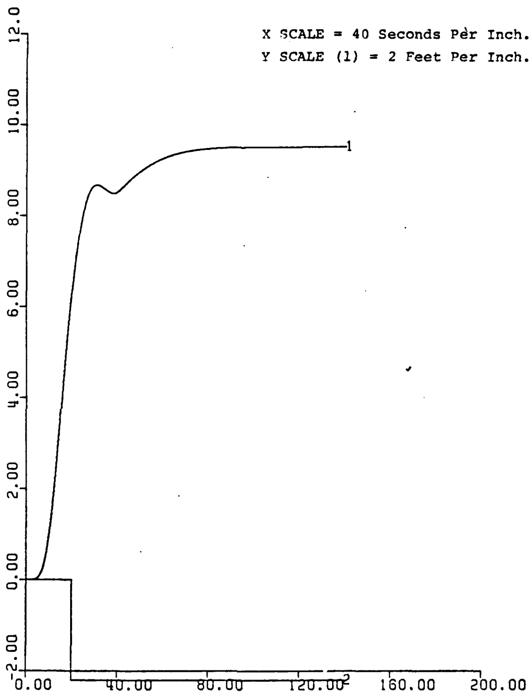
Figure 111.1. Depth vs. Time. Roll Stability Step Test.
