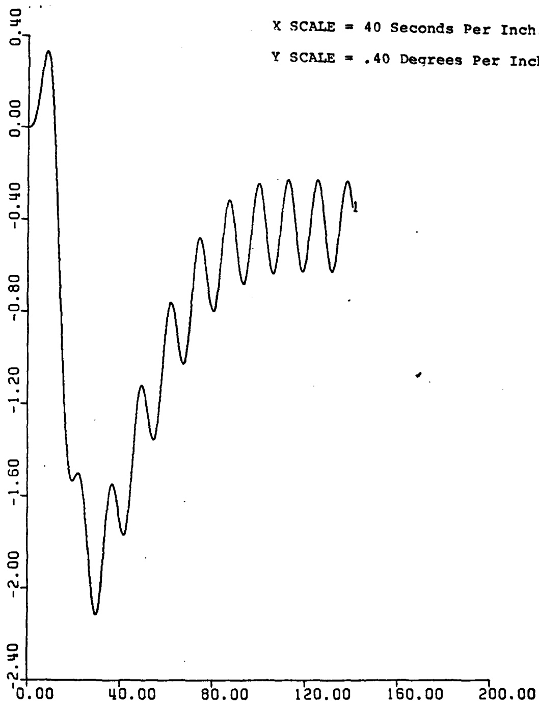
Figure 42. Roll vs. Time. With Depth-Pitch Controller. UCK = 6 Knots. Rudder Ordered = 35^{\circ} .
