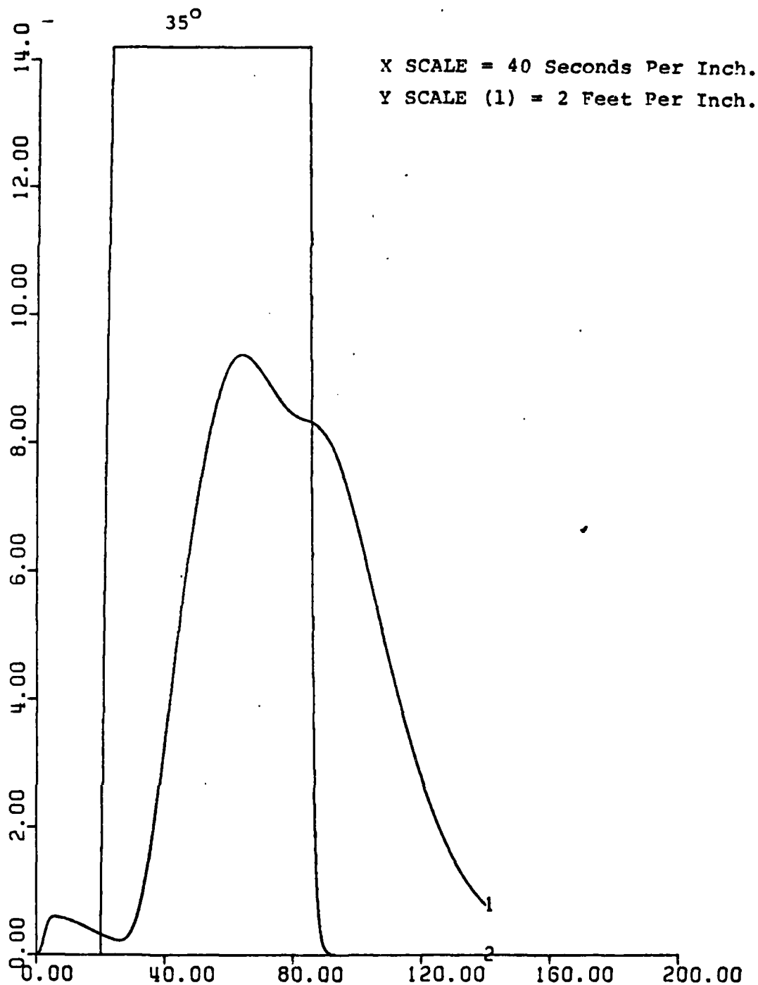
Figure 83.1. Depth vs. Time Final Result With Roll Error Limiter. K1 = 5 , K2 = 10 . UCK = 12 Knots. Initial Roll Angle = -20^\circ .
