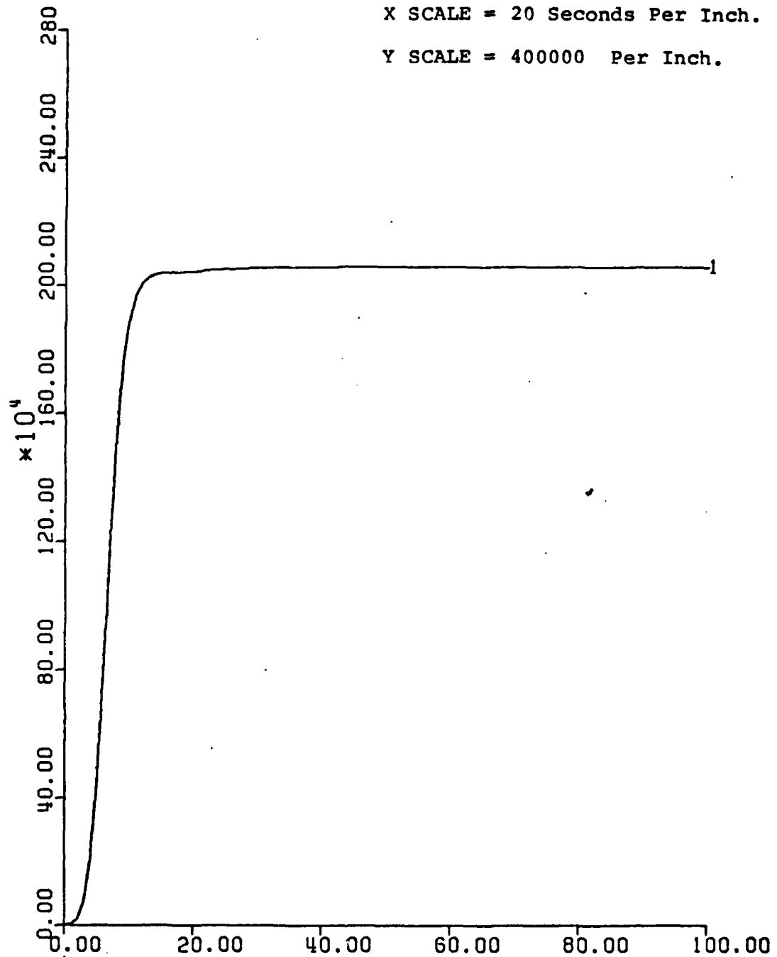
Figure 36. K44 vs. Time. UCK = 15 Knots. D = 8000, A = 0, E = 10, B = 0, C = 100.
