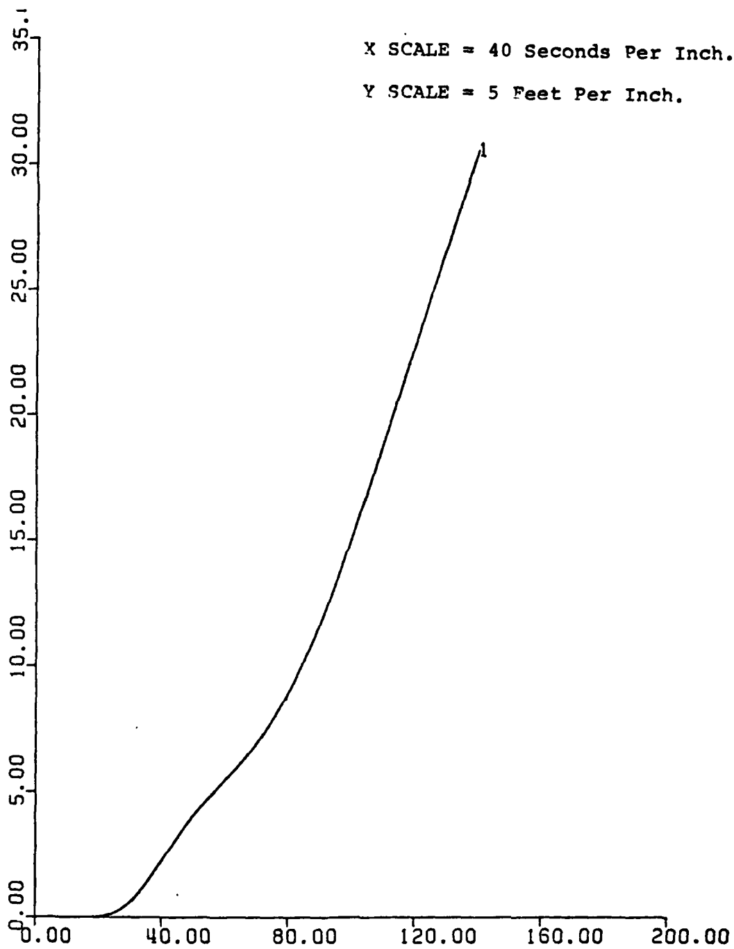
Figure 20. Depth vs. Time. With No Controller. UCK = 6 Knots. Rudder Ordered = 35^{\circ} .
