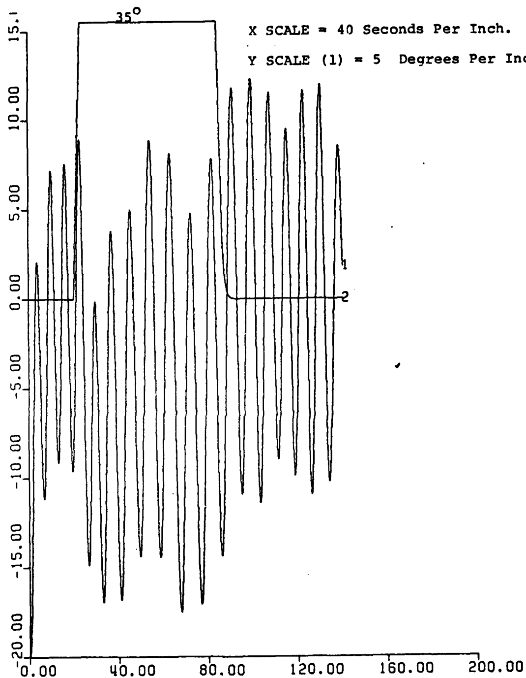
Figure 69.1. Roll vs. Time. K_1 = 3 , K_2 = 10 . UCK = 24 Knots. Initial Roll Angle = -20^\circ . .2. Rudder Response vs. Time (Rudder Ordered = 35^\circ .)
