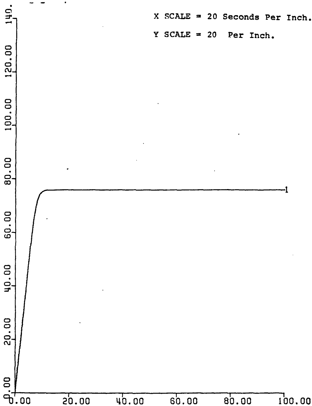
Figure 27. K11 vs. Time. UCK = 15 Knots. D = 8000, A = 0, E = 10, B = 0, C = 100.
