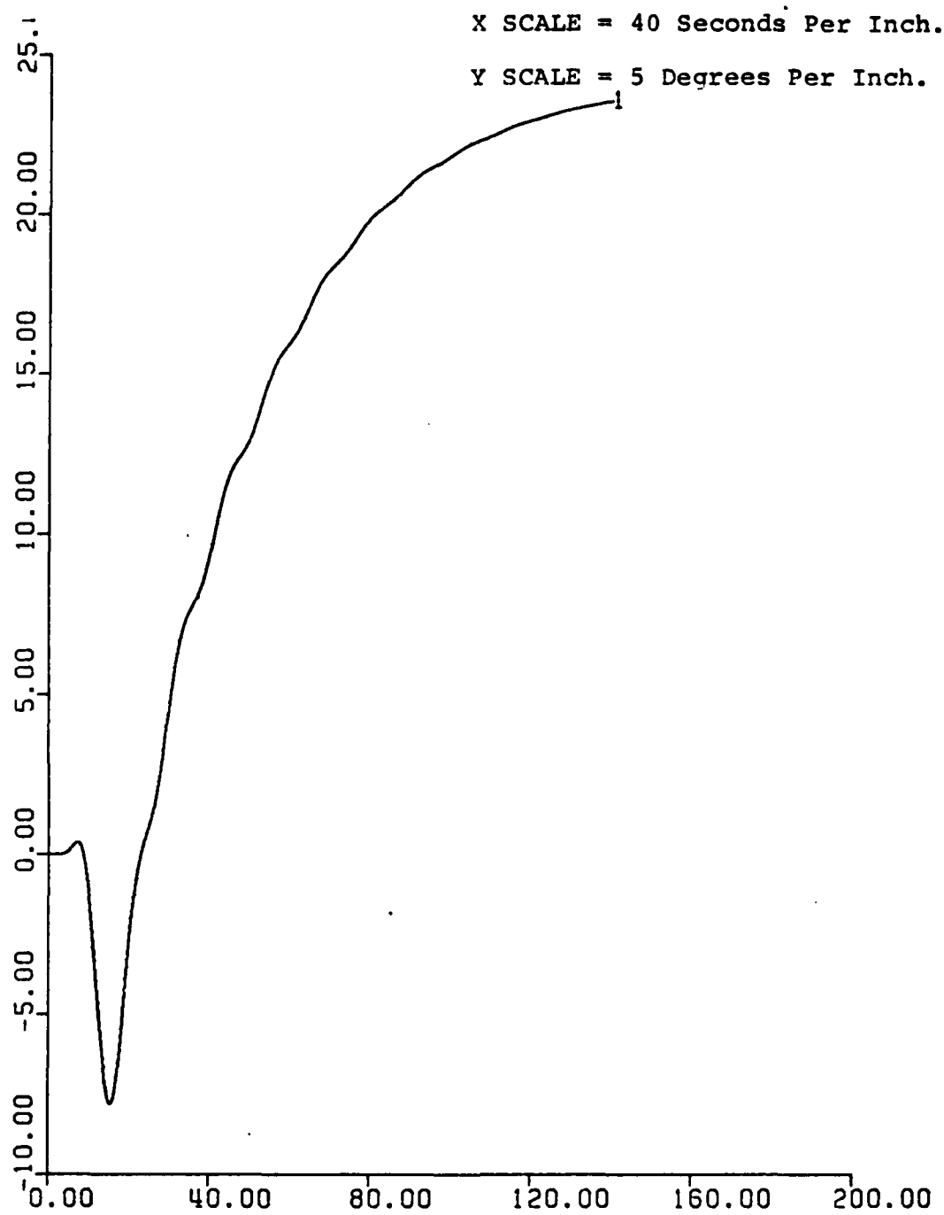
Figure 4. Pitch vs. Time. With No Controller. UCK = 24 Knots. Rudder Ordered = 35^{\circ} .
