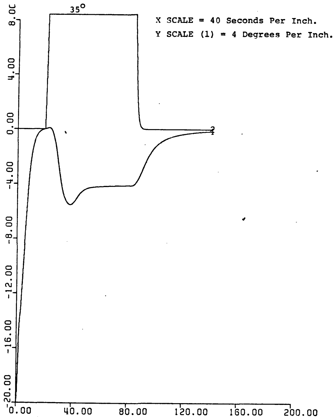
Figure 75.1. Roll vs. Time. Final Result With Roll Error Limiter. K_1 = 3 , K_2 = 10 . UCK = 24 Knots. Initial Roll Angle = -20^\circ .
