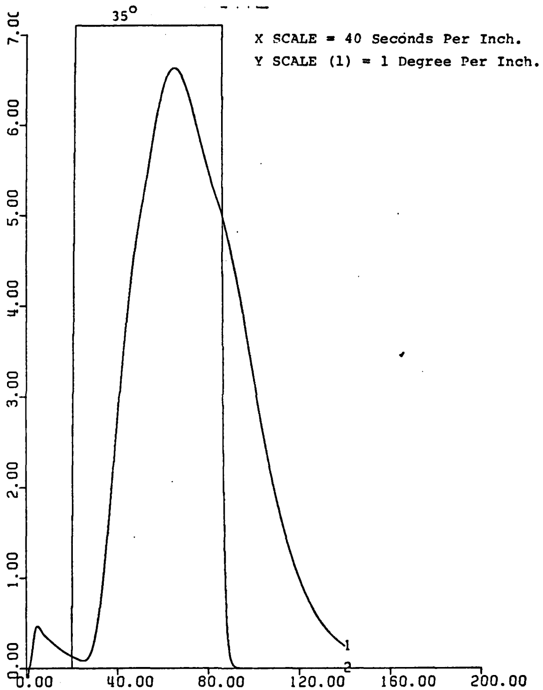
Figure 84.1. Pitch vs. Time. Final Result With Roll Error Limiter. K1 = 3, K2 = 10, UCK = 12 Knots. Initial Roll Angle = -20°.
