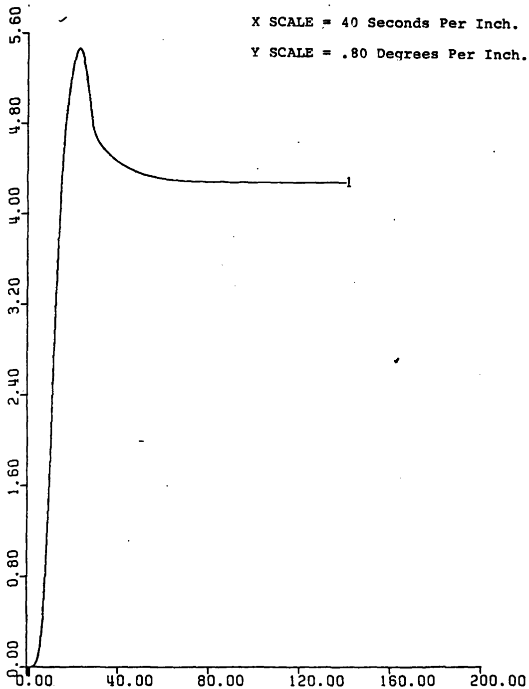
Figure 59. Pitch vs. Time. K_1 = 3 . UCK = 24 Knots. Rudder Ordered = 35^\circ . Initial Roll Angle = 0^\circ .
