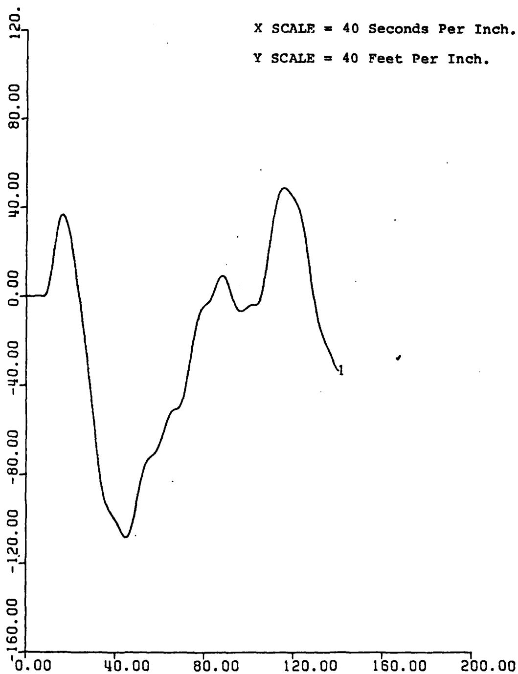
Figure 63. Depth vs. Time. K1 = 3 . UCK = 24 Knots. Rudder Ordered = 35^\circ . Initial Roll Angle = -5^\circ .
