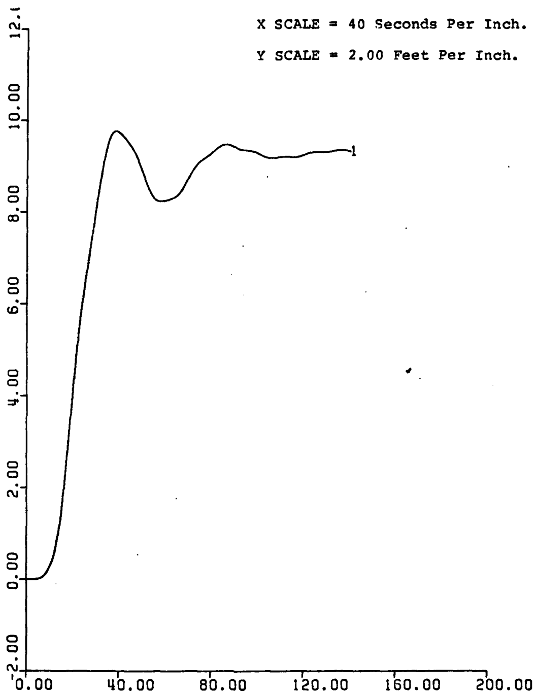
Figure 44. Depth vs. Time. With Depth-Pitch Controller. UCK = 12 Knots. Rudder Ordered = 35^{\circ} .
