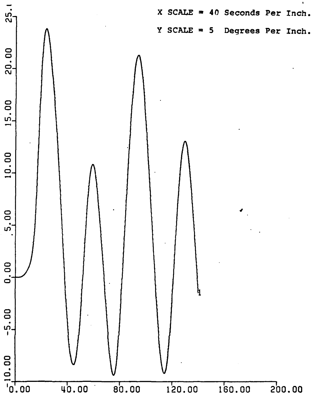
Figure 53. Pitch vs. Time. With Depth-Pitch Controller. UCK = 24 Knots. Rudder Ordered = 35^{\circ} .
