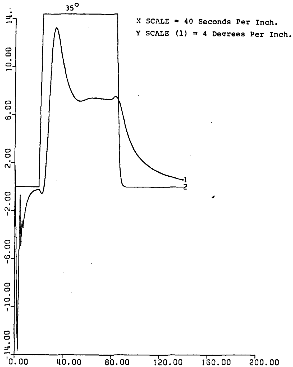
Figure 82.1. Sailplane Angle vs. Time. Final Result With Roll Error Limiter. K_1 = 3 , K_2 = 10 . UCK = 18 Knots. Initial Roll Angle = -20^\circ . .2. Rudder Response vs. Time (Rudder Ordered = 35^\circ ).
