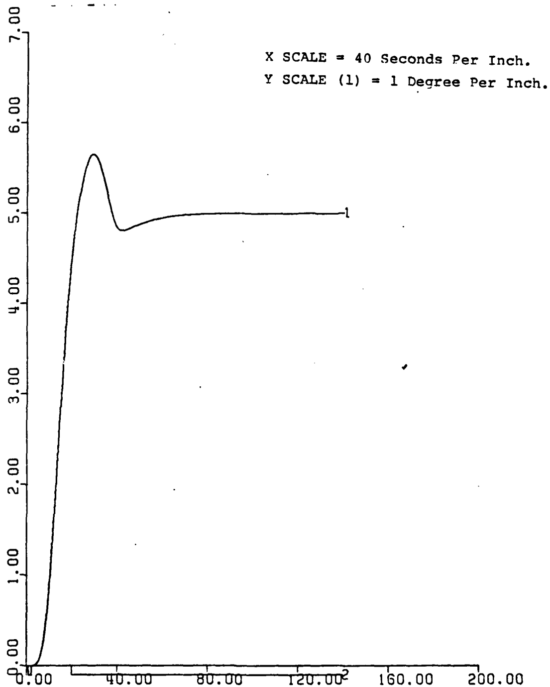
Figure 112.1. Pitch vs. Time. Roll Stability Step Test.
