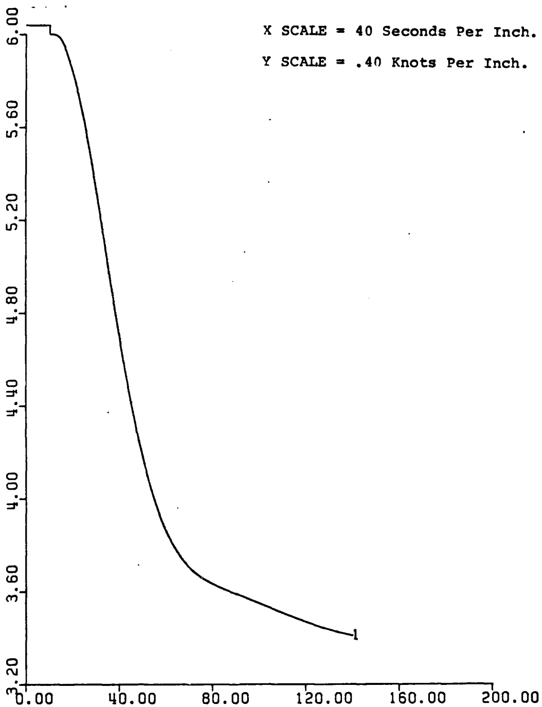
Figure 23. Speed Change vs. Time. With No Controller. UCK = 6 Knots. Rudder Ordered = 35^{\circ} .
