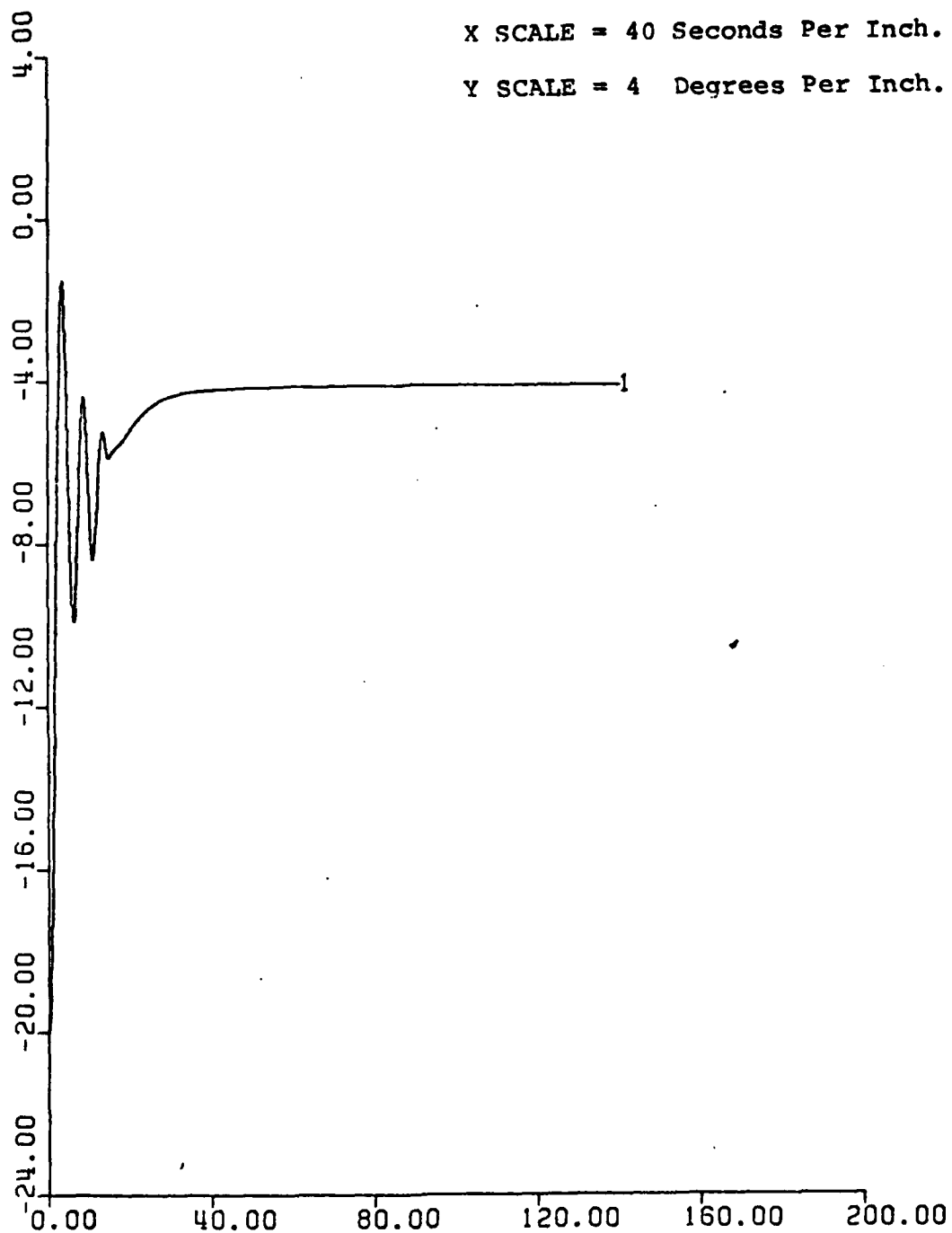
Figure 66. Roll vs. Time. K_1 = 3 , K_2 = 10 . UCK = 24 Knots. Rudder Ordered = 35^\circ . Initial Roll Angle = -20^\circ .
