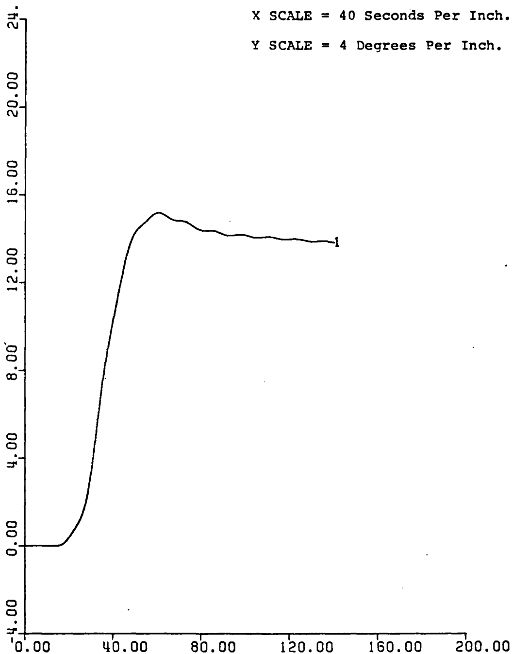
Figure 15. Pitch vs. Time. With No Controller. UCK = 12 Knots. Rudder Ordered = 35^{\circ} .
