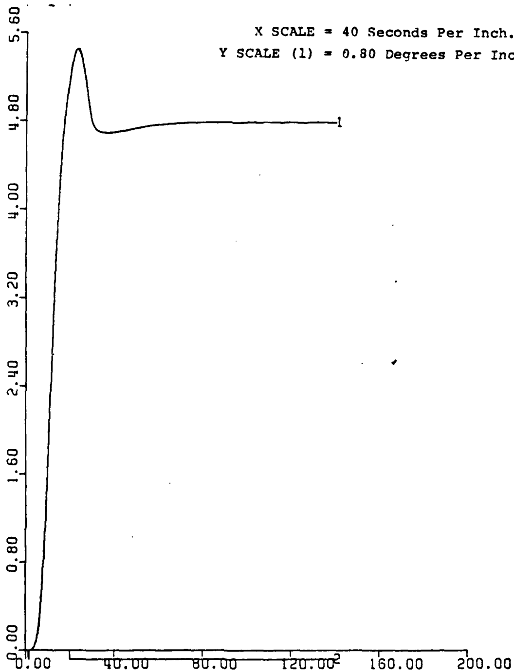
Figure 107.1. Pitch vs. Time. Roll Stability Step Test. UCK = 24 Knots. Rudder Ordered = 35^{\circ} . .2. Disturbance vs. Time. ( 1.1028 \times 10^7 ft-lb.).
