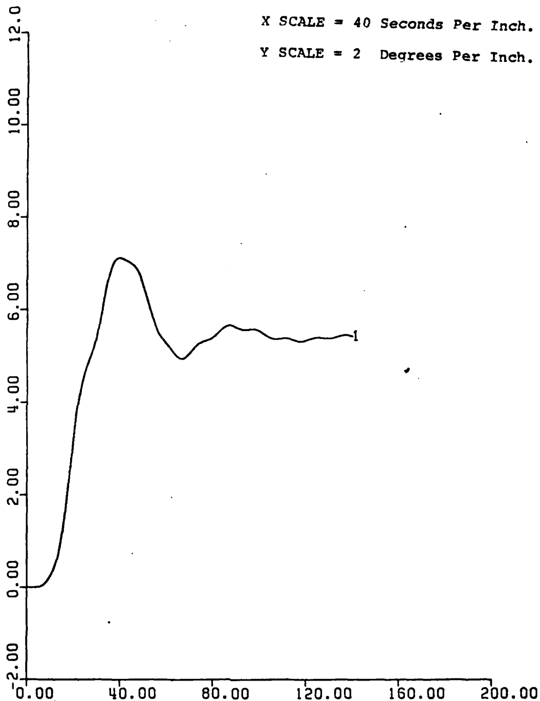
Figure 45. Pitch vs. Time. With Depth-Pitch Controller. UCK = 16 Knots. Rudder Ordered = 35^{\circ} .
