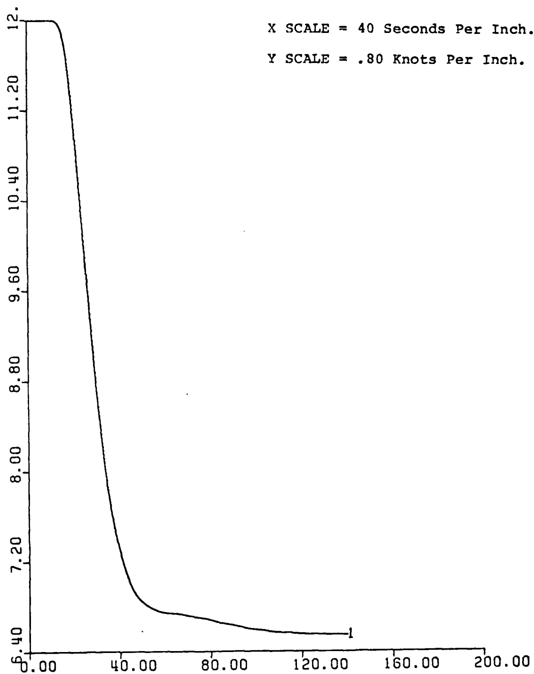
Figure 17. Speed Change vs. Time. With No Controller. UCK = 12 Knots. Rudder Ordered = 35^{\circ} .
