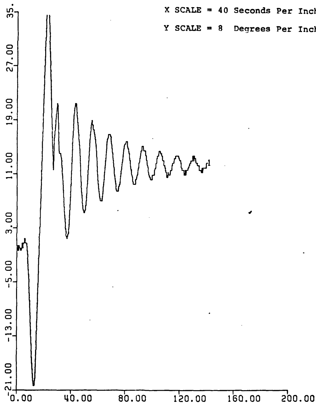
Figure 51. Sternplane Angle vs. Time. With Depth-Pitch Controller. UCK = 18 Knots. Rudder Ordered = 35^{\circ} .
