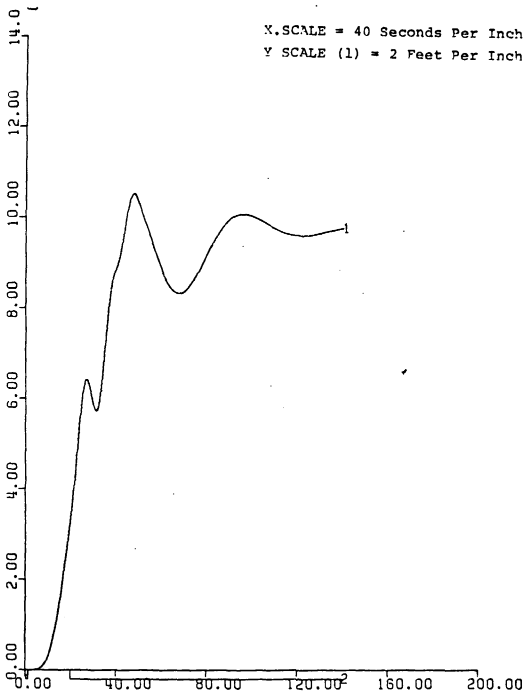
Figure 116.1. Depth vs. Time. Roll Stability Step Test.
