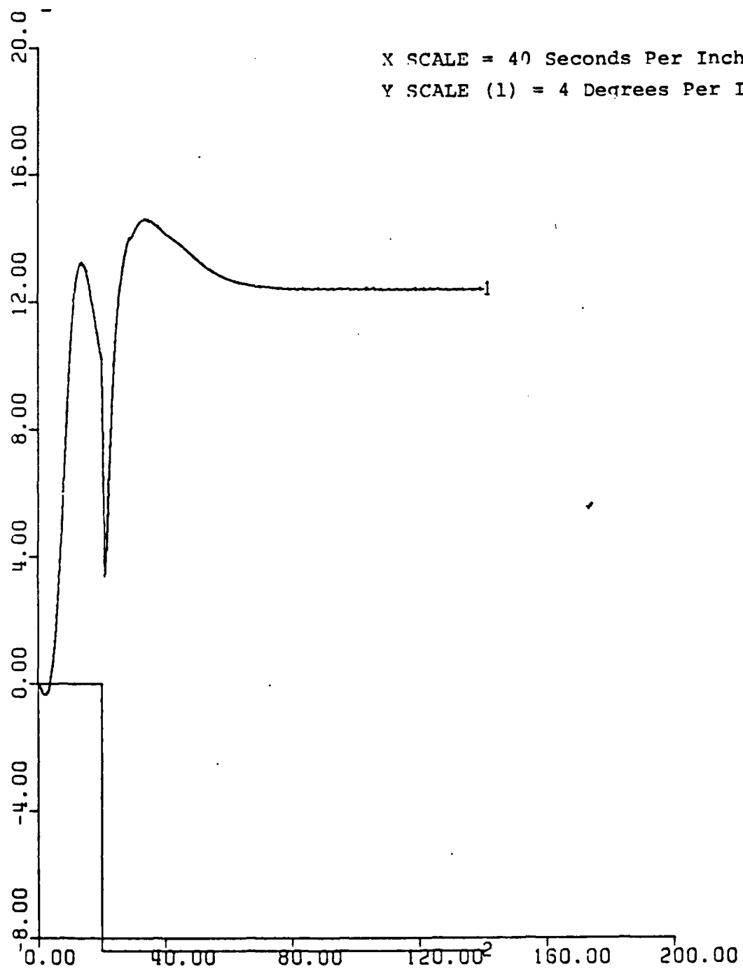
Figure 115.1. Sailplane Angle vs. Time. Roll Stability Step Test. UCK = 24 Knots. Rudder Ordered = 35^{\circ} .
