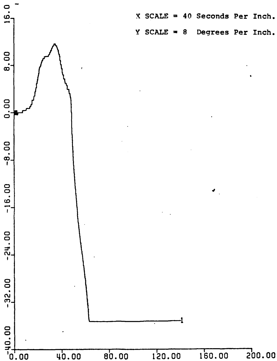
Figure 43. Sternplane Angle vs. Time. With Depth-Pitch Controller. UCK = 6 Knots. Rudder Ordered = 35^{\circ} .
