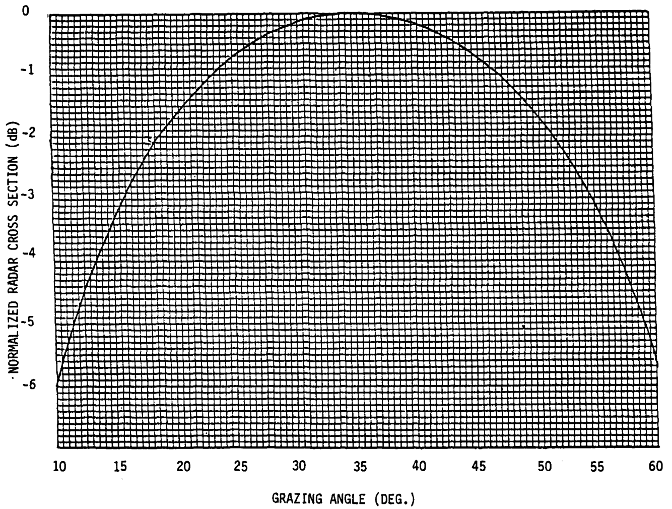
Figure 5-5. Normalized Radar Cross Section vs Grazing Angle for a Triangular Trihedral Corner Reflector.
