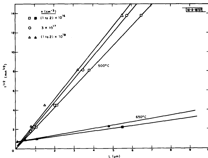
Fig. V-2. P-n junction depth ( L ) as a function of square root of diffusion time ( t^{1/2} ) for Zn diffusion into n-InP at 500^\circ and 650^\circ\text{C} using a \text{ZnP}_2 source.
