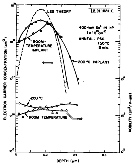
Fig. III-2. Electron carrier concentration and mobility vs depth measured in InP implanted at room temperature and 200^\circ\text{C} with 1 \times 10^{14} \text{ cm}^{-2} of 400-keV Se ions. Also shown is Se distribution expected from LSS range theory.
