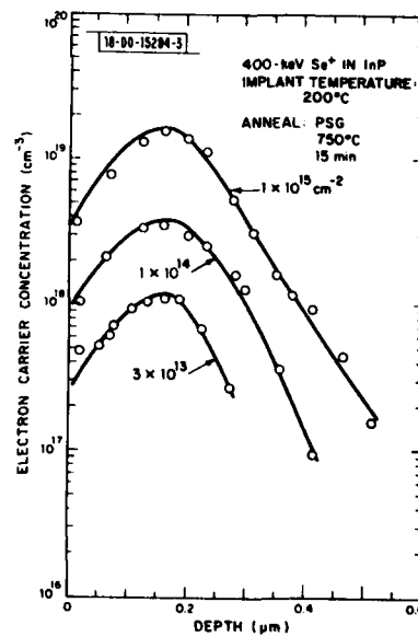
Fig. III-3. Electron carrier concentration vs depth for InP samples implanted at 200^\circ\text{C} with 3 \times 10^{13} , 1 \times 10^{14} , and 1 \times 10^{15} \text{ cm}^{-2} of 400-keV Se.
