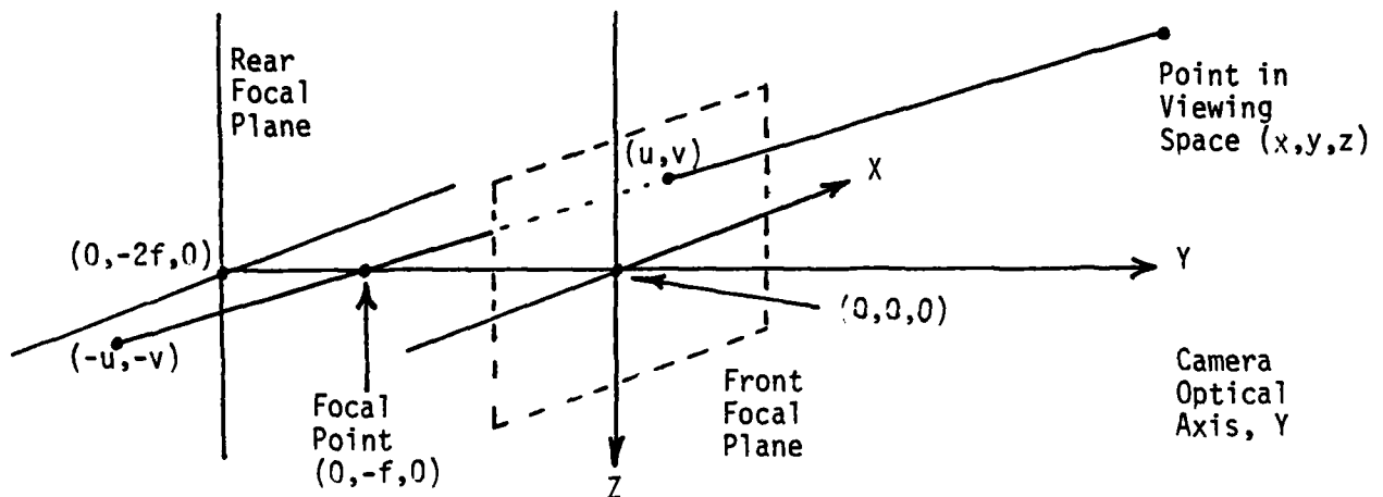
Figure 1 Camera Geometry
