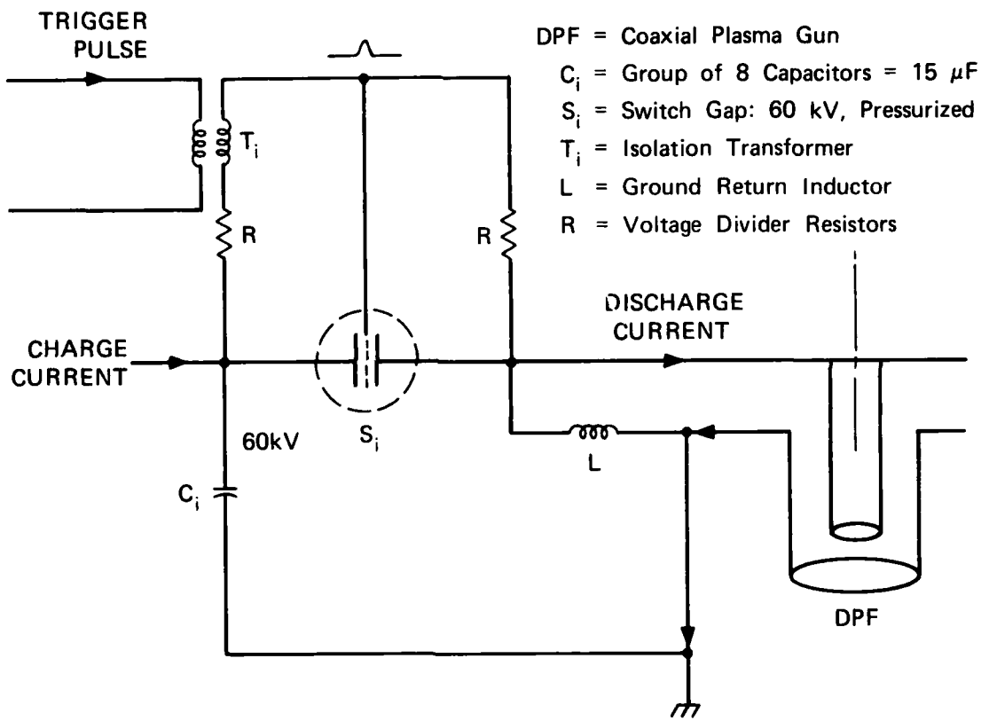
FIGURE 2 DPF SYSTEM
