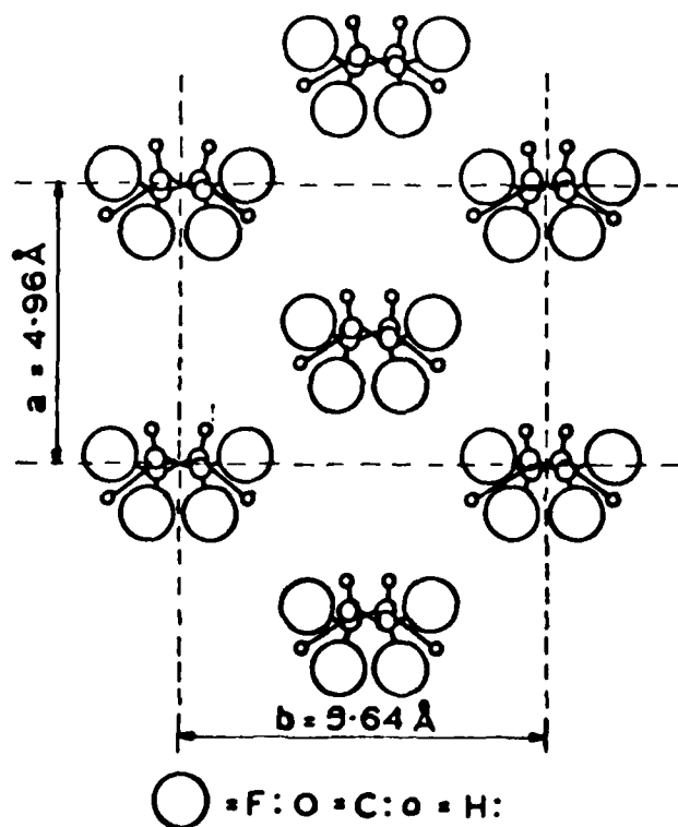
Fig. 24. Suggested intermediate form after corona charging.
