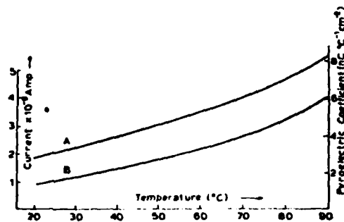
FIGURE 2 Thermally stimulated current and pyroelectric coefficient with 25 \mu\text{m} thick and corona charged \text{PVF}_2 during the second cycle (reversible pyroelectric current). Poling conditions for Curves A and B and the heating rate are the same as in Figure 1.
