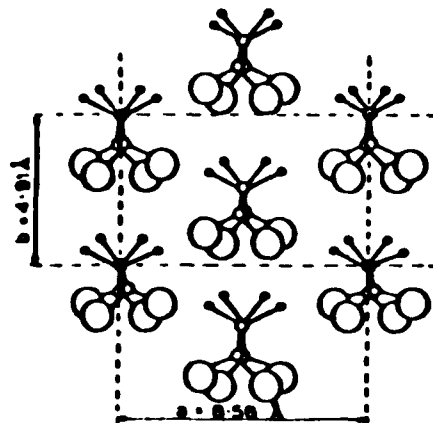
Figure 1. Form I PVF_2 viewed along c-axis (along main chains)
