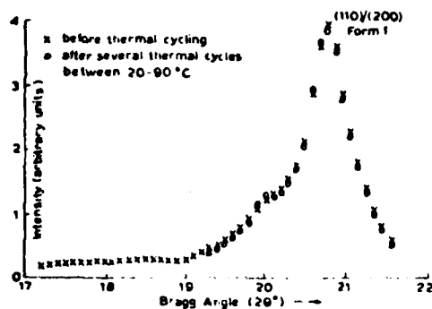
FIGURE 5 Effect of thermal aging on the X-ray diffraction profiles of corona charged (10 kV) \text{PVF}_2 of 25 \mu\text{m} thickness.
