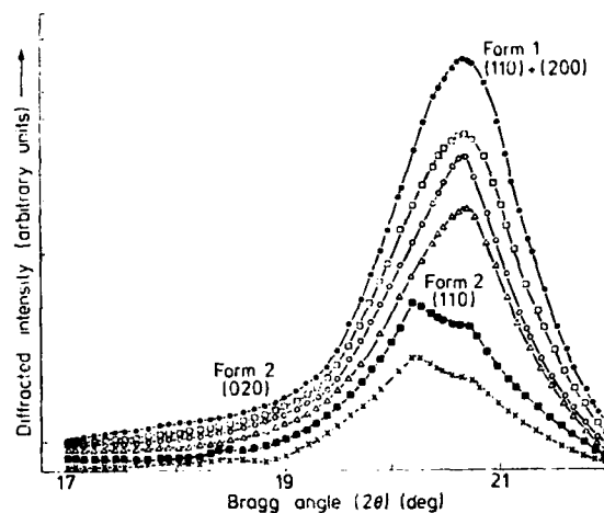
Figure 2. X-ray diffraction profiles of uniaxially stretched \text{PVF}_2 films (2:1 to 7:1 stretch ratio) after corona charging to a surface potential of 6 kV. Symbols: same as for figure 1.
