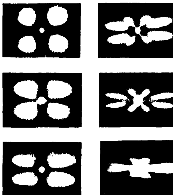
Fig. 10. Small Angle Light Scattering Patterns (SALS) of \text{PVF}_2 with different stretch ratios. a, b, c, d, e and f represent no stretch, 10%, 30%, 60%, 95% and 140% stretch ratios respectively.
