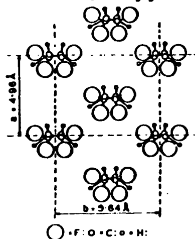
Figure 3. Suggested intermediate form after corona charging.
