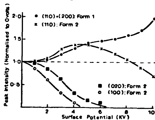
Variation of Intensities of Major Peaks after Corona Charging (25 \mu m sample)
