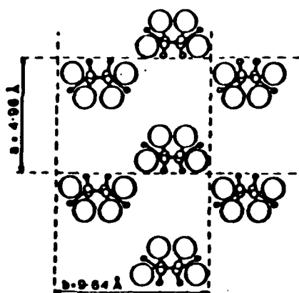
Form II PVF_2 viewed along c-axis (along main chains) ○ = F : ○ = C : ○ = H :
