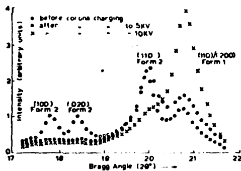
FIGURE 4 X-ray diffraction pattern of 25 \mu\text{m} thick \text{PVF}_2 before and after corona poling. Poling time and temperature are the same as in Figure 1.
