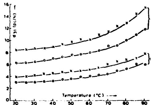
FIGURE 3 The behavior of the piezoelectric strain coefficient d_{31} of corona charged \text{PVF}_2 with temperature. Poling conditions are as in Figure 1; X first cycle and O second cycle.
