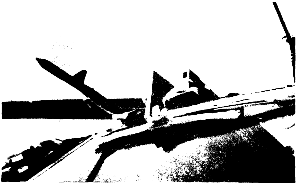
Photo 5. Ice Formation on Windshield Wiper Assembly (52 min in Natural Cloud of 0.08 to 0.11 g/m^3 and -8°C).
