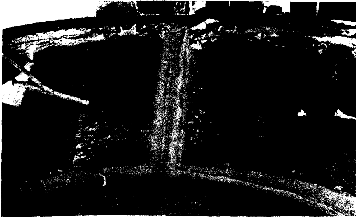
Photo 16. Windshield Obscured by Ice Formation (22.5 min in HISS Plume with LWC of 0.25 \text{ g/m}^3 and -15^\circ\text{C} ).
