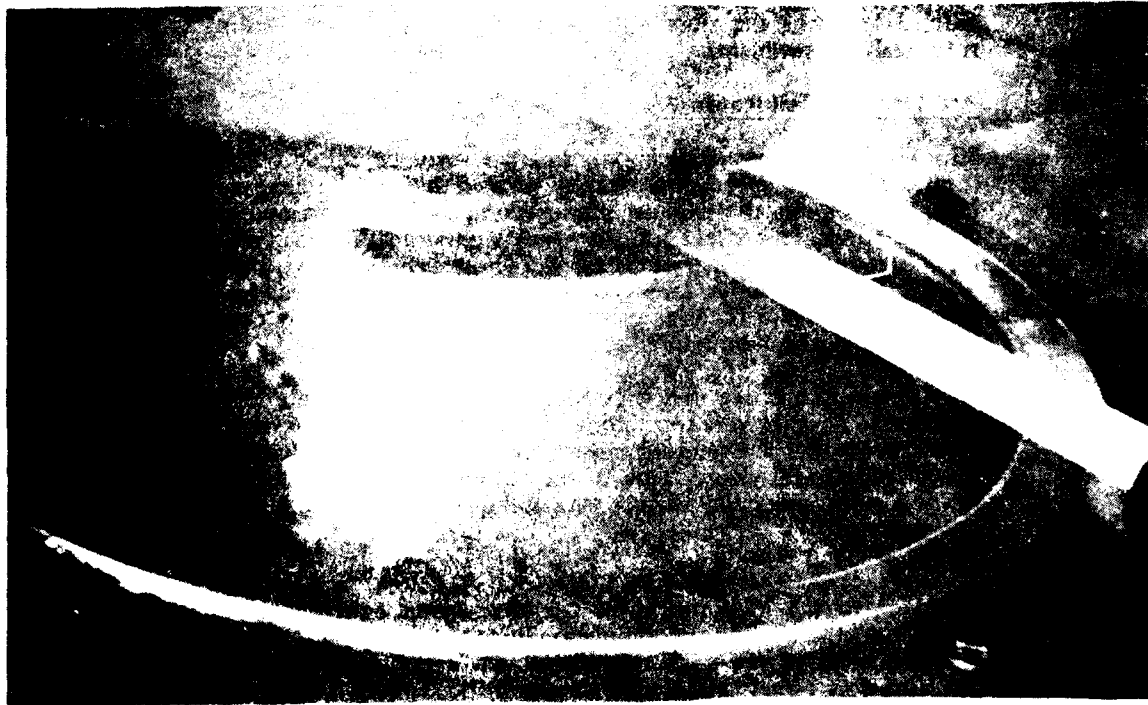
Photo 8. Ice Accumulation on Stationary Components (24 mm) in HISS Plume with IWC of 0.5 \text{ g m}^{-3} and -15 \text{ C} .
