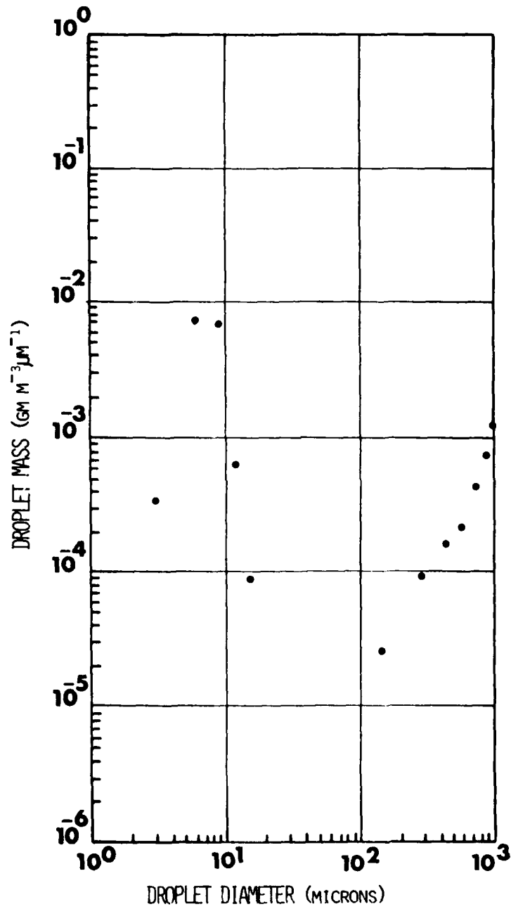
FIGURE 13 FREEZING RAIN
