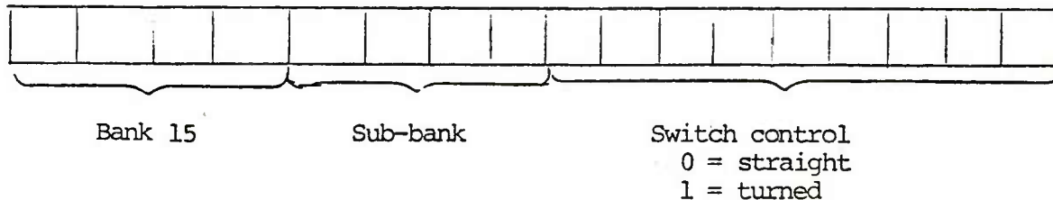
Figure 9. Switch Control Word
