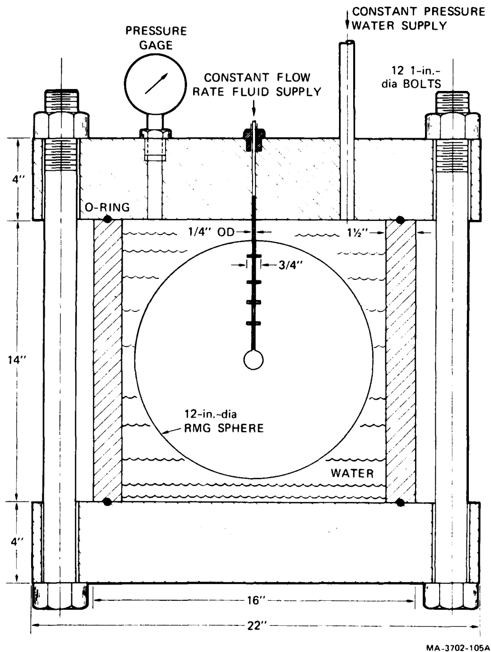
FIGURE 2.2 CONTAINMENT EXPERIMENT APPARATUS
