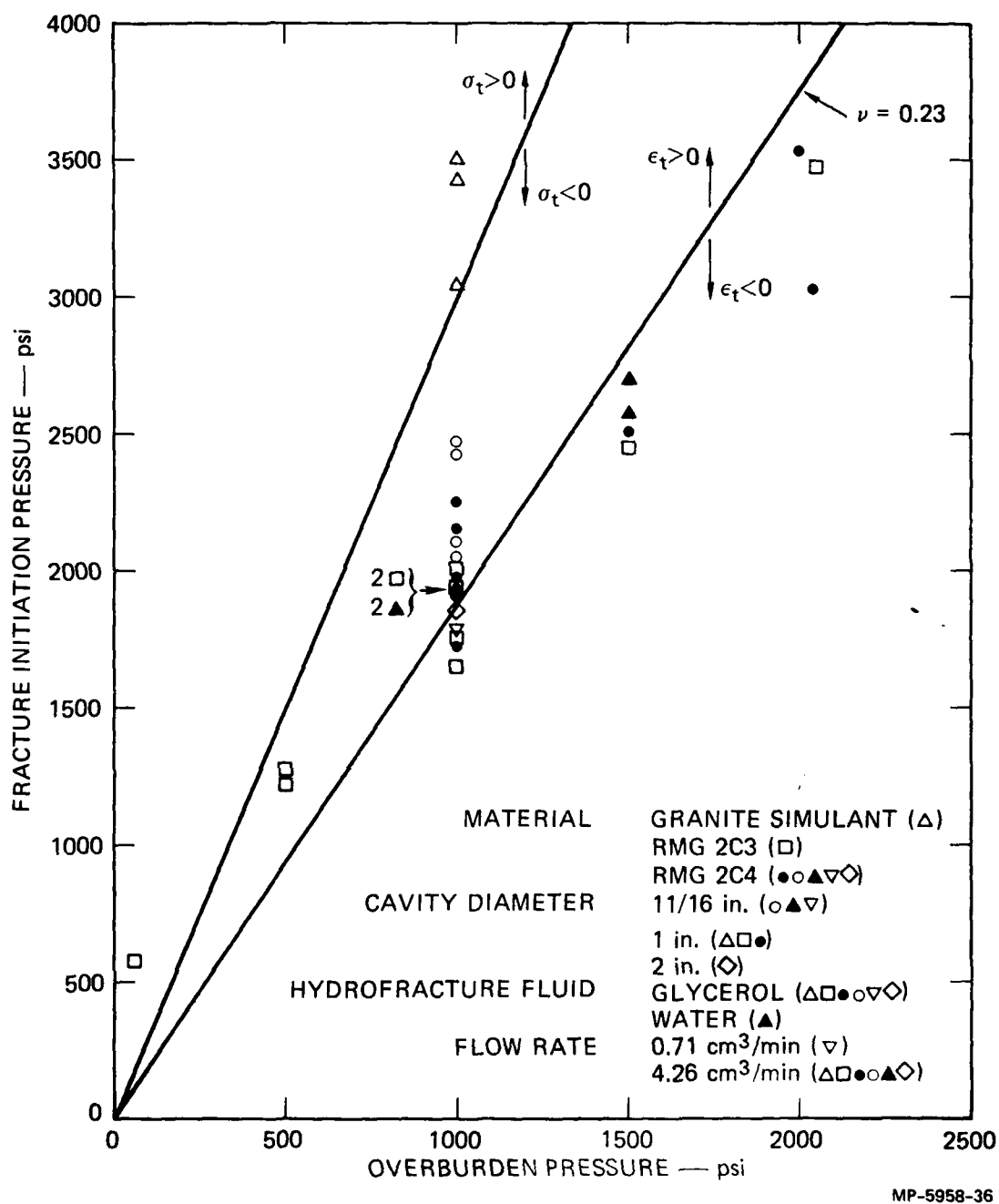
FIGURE 3.9 FRACTURE INITIATION PRESSURE VERSUS OVERBURDEN PRESSURE FOR UNEXPLODED CAVITIES
