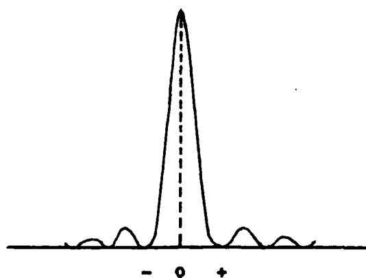
Fig. 4. Intensity distribution upon addition of the cubic perturbation term to the cylindrical surface of large radius of curvature.
