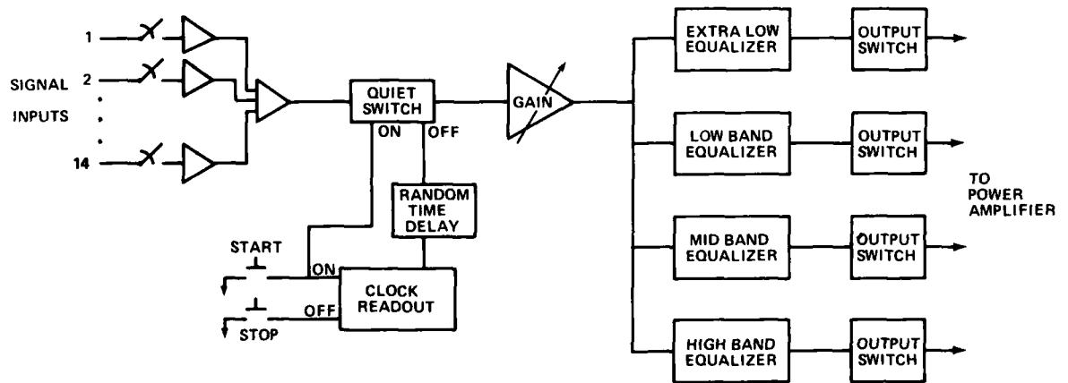
Figure 2. Signal control and equalization circuitry.
