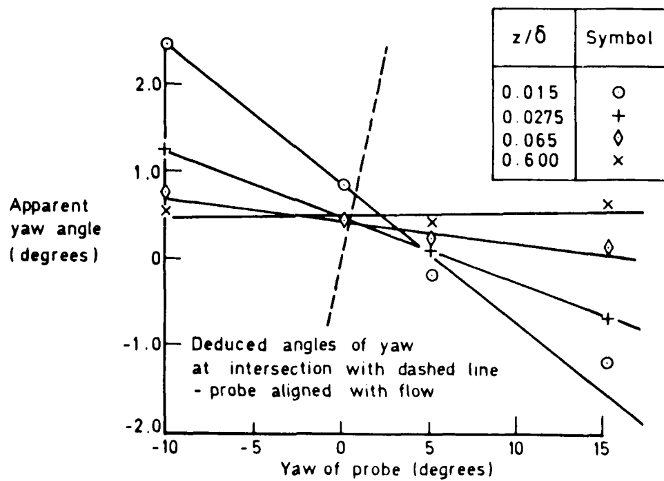
Fig 19 Measurement of yaw angles in a boundary layer
