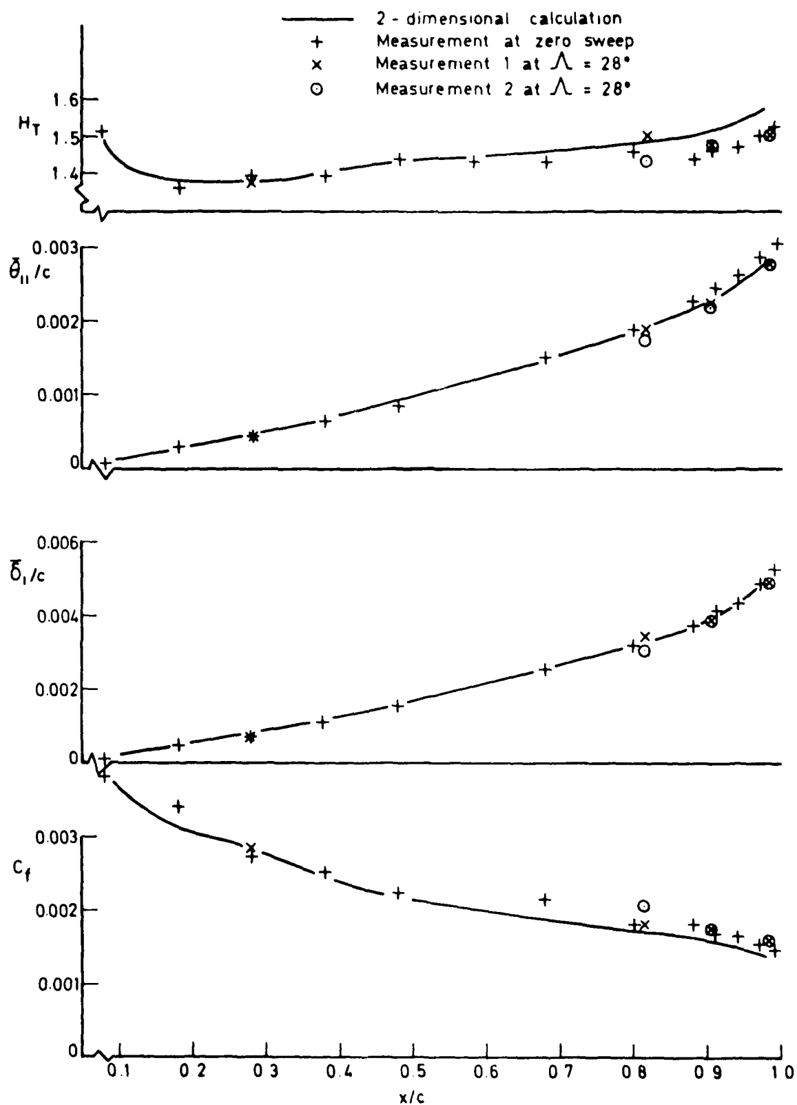
Fig 34a Comparison with two-dimensional calculation and measurement on the upper surface at M_N = 0.675 and \alpha_N = +2^\circ
