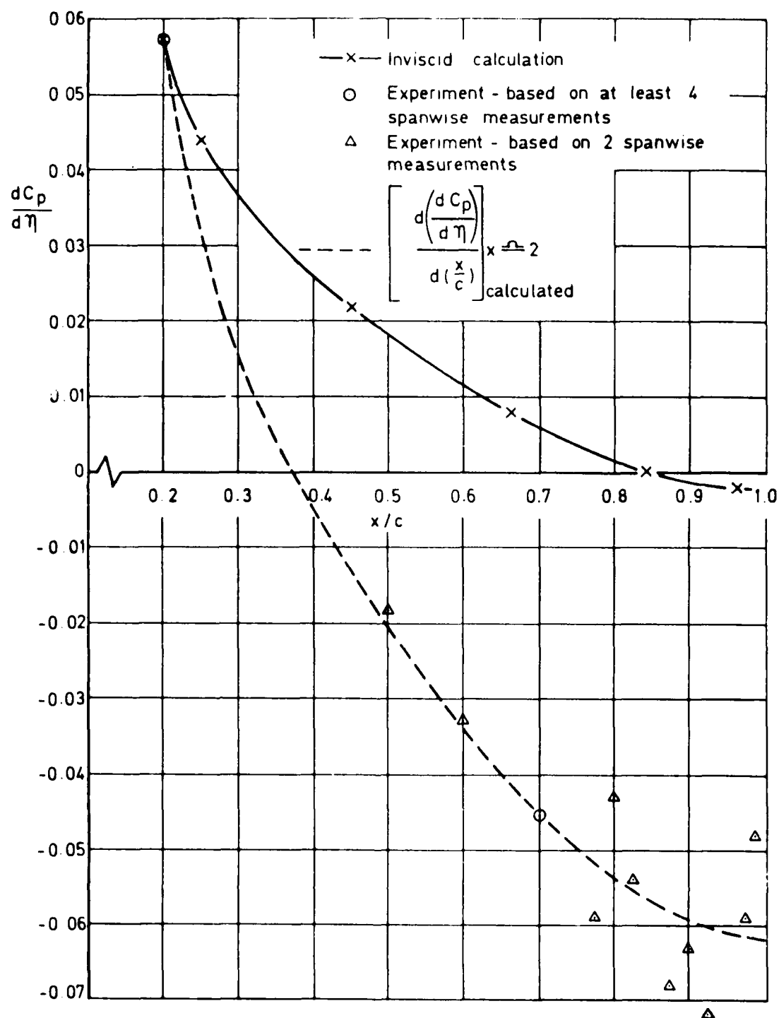
Fig 27 Rate of change of upper surface pressure across the span at \Lambda = 28^\circ , M_N = 0.4 , \alpha_N = +2^\circ
