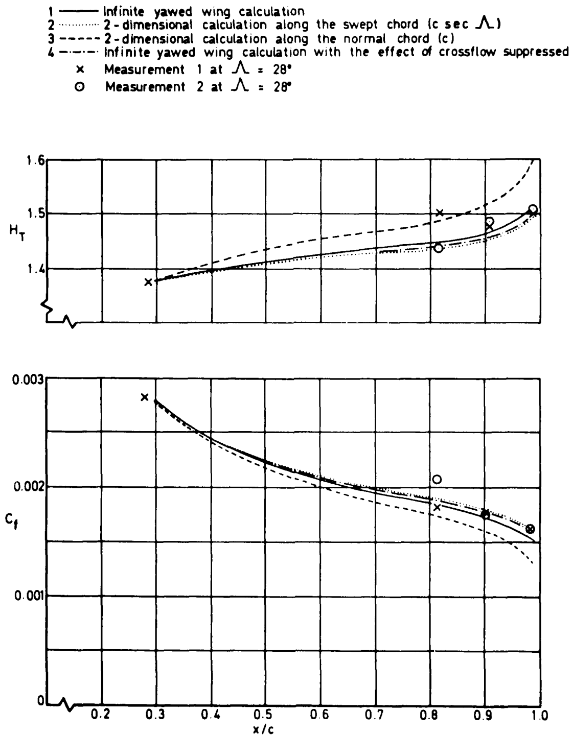
Fig 35b Comparison between two-dimensional and three-dimensional calculations on the upper surface at \Lambda = 28^\circ , M_N = 0.675 , \alpha_N = +2^\circ
