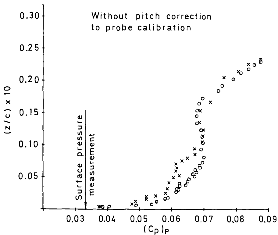
Fig 23c Static pressure profile at x/c = 0.903 for \Lambda = 28^\circ , M_N = 0.675 , \alpha_N = +2^\circ
