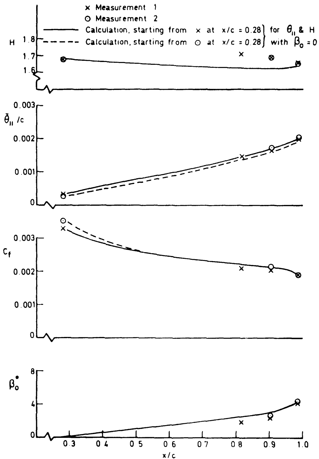
Fig 30j Comparison with yawed wing calculation for \Lambda = 20^\circ , M_N = 0.675 , \alpha_N = -2^\circ
