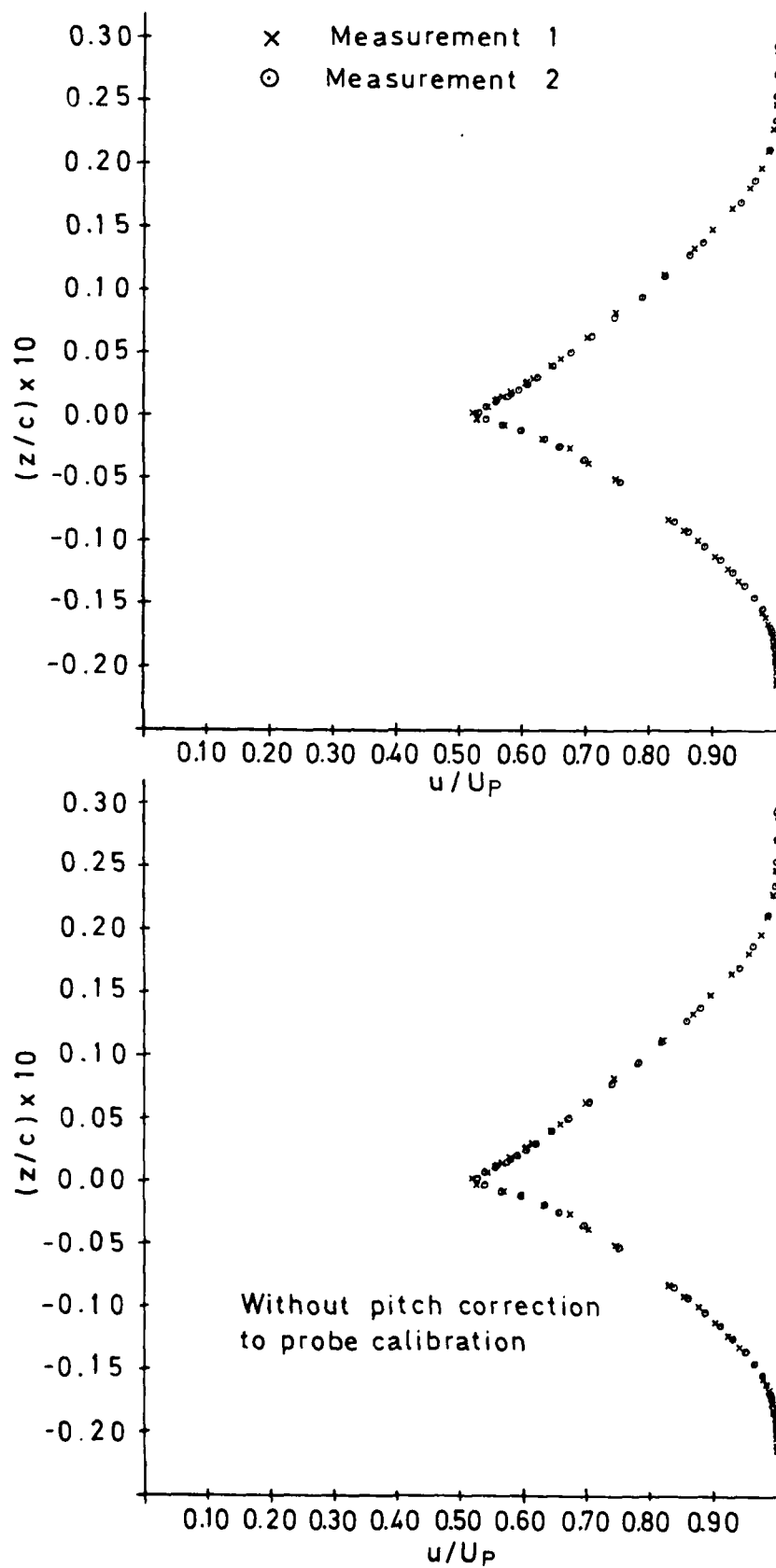
Fig 25b Velocity profile at x/c = 1.010 for \Lambda = 28^\circ , M_N = 0.675 , \alpha_N = +2^\circ
