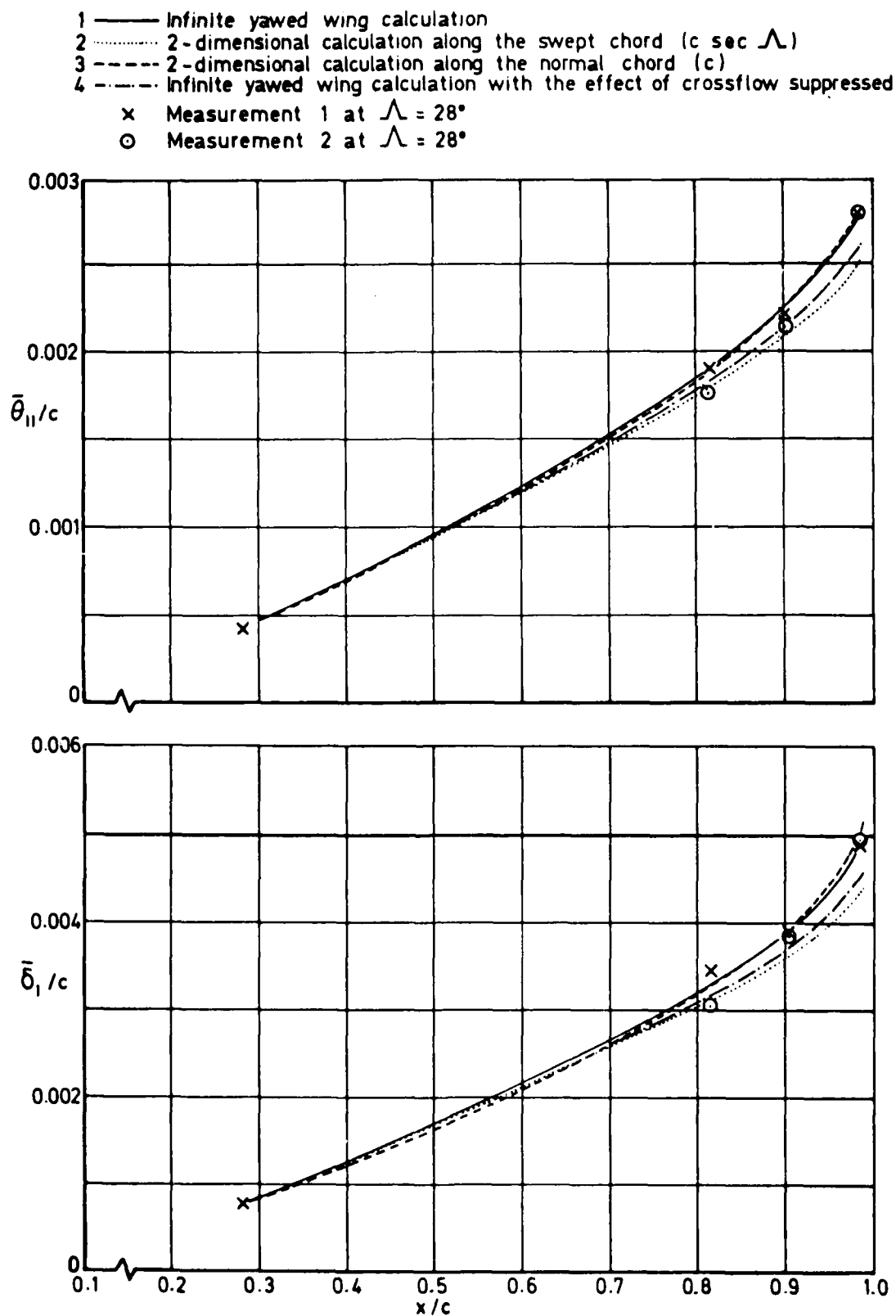
Fig 35a Comparison between two-dimensional and three-dimensional calculations on the upper surface at \Lambda = 28^\circ , M_N = 0.675 , \alpha_N = +2^\circ
