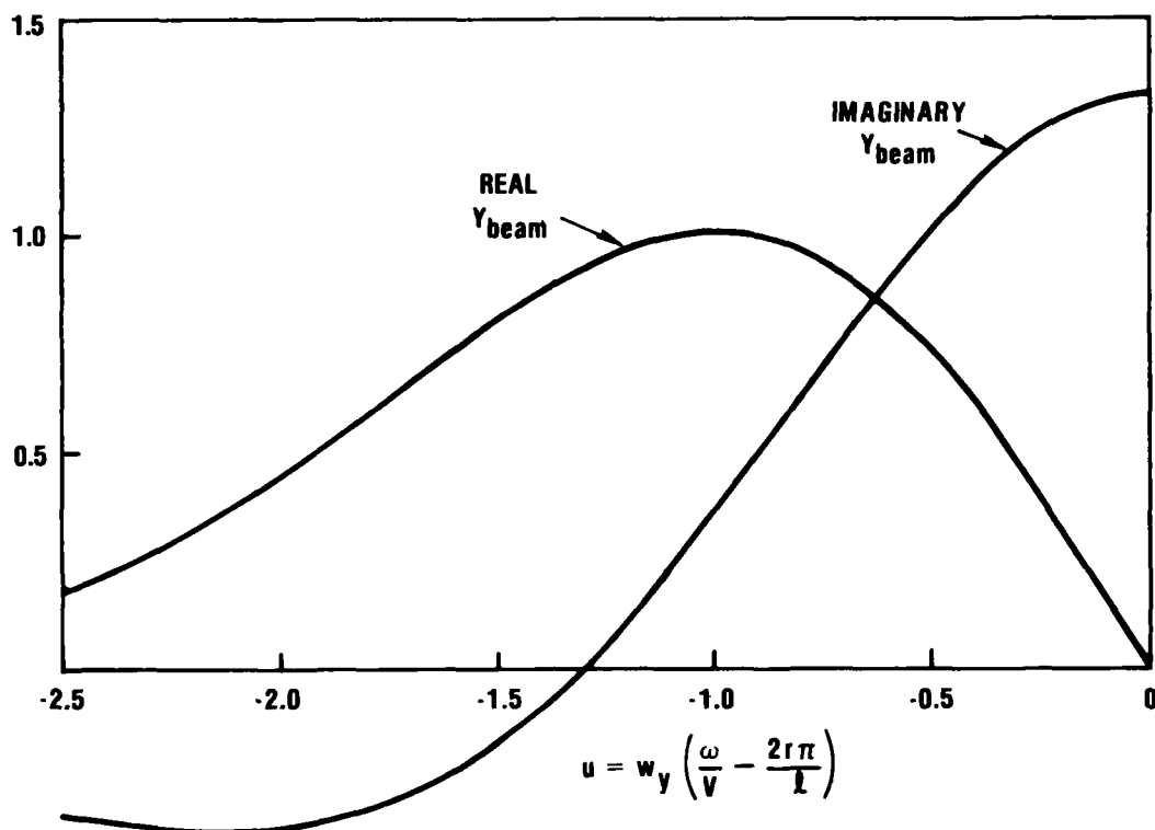
Figure 3. Real and imaginary parts of normalized electron beam admittance at I_0 = I_s (min).
