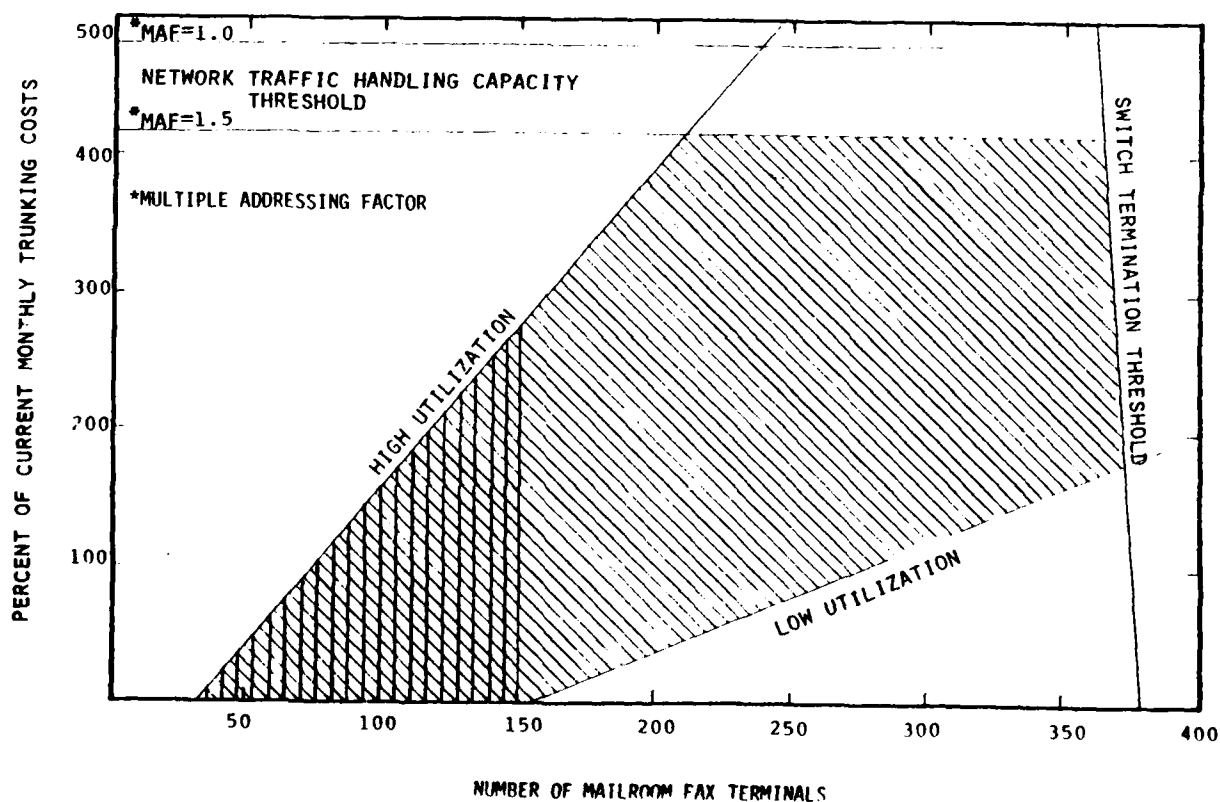
Figure 38. Additional Costs to Maintain Current AUTODIN Speed of Service With Increasing FAX Demand - Pacific AUTODIN (Expected Usage)
