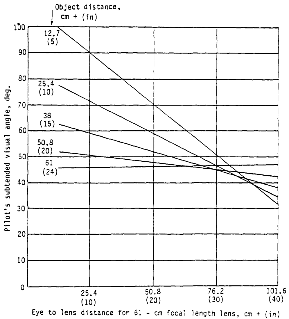
Figure 4. Relationship between pilot's subtended visual angle, object distance, and eye-to-lens distance for a 61-cm focal length lens (Ganzler, 1971).
