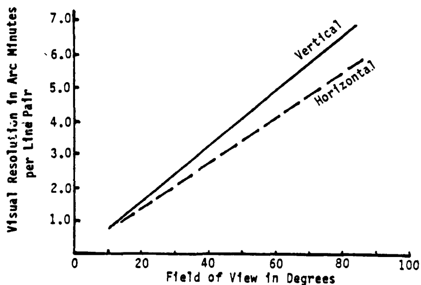
Figure 5. Interrelationship of visual resolution and field of view for a 1000 line visual system.
