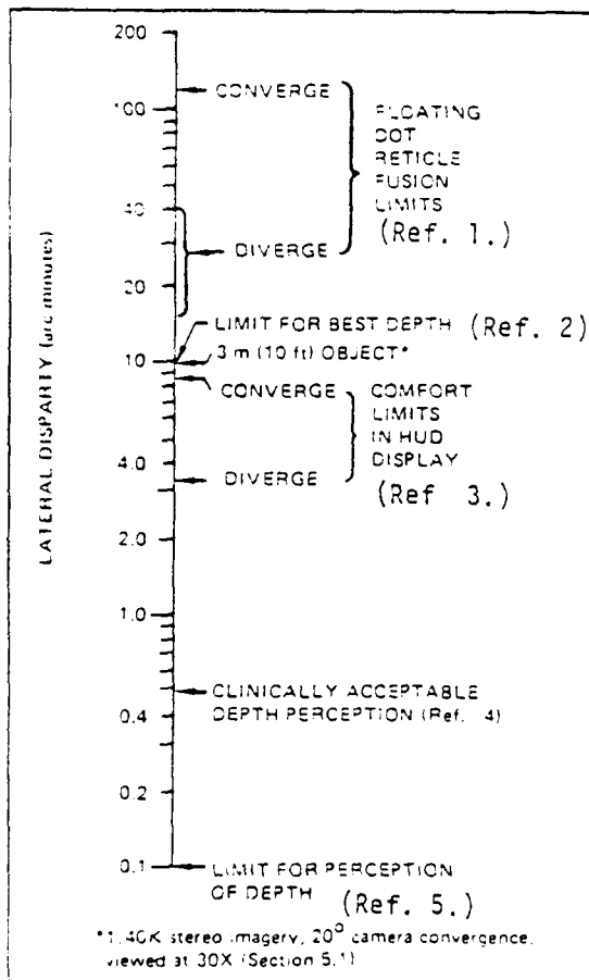
Figure 10. Effects of specific lateral disparities. (Farrell & Booth, 1975)
