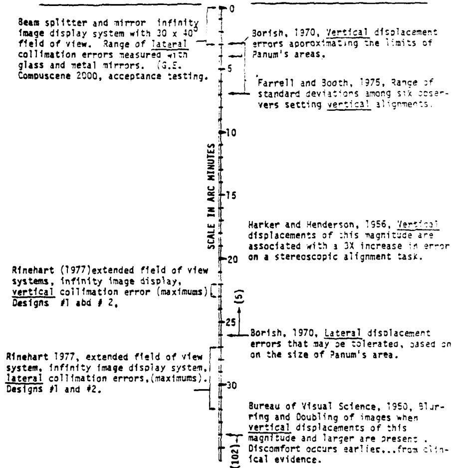
Figure 46. Comparison between collimation errors in two display systems and physiological and behavioral data applicable to collimation limits.
