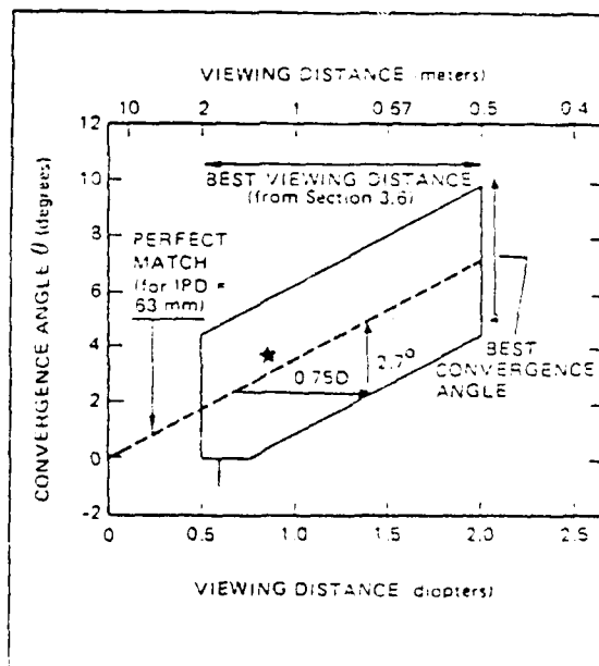
Figure 44. Reprinted page from 'Design Handbook for Imagery Interpretation Equipment.' (Farrell & Booth, 1975).
