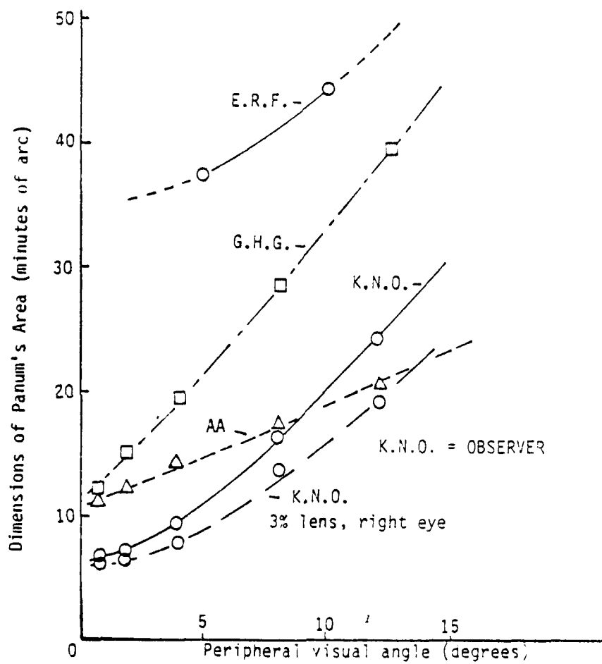
Figure 8. Relationship of magnitude of transverse extent of Panum's fusional areas with peripheral angle for several observers. (Ogle, 1950)
