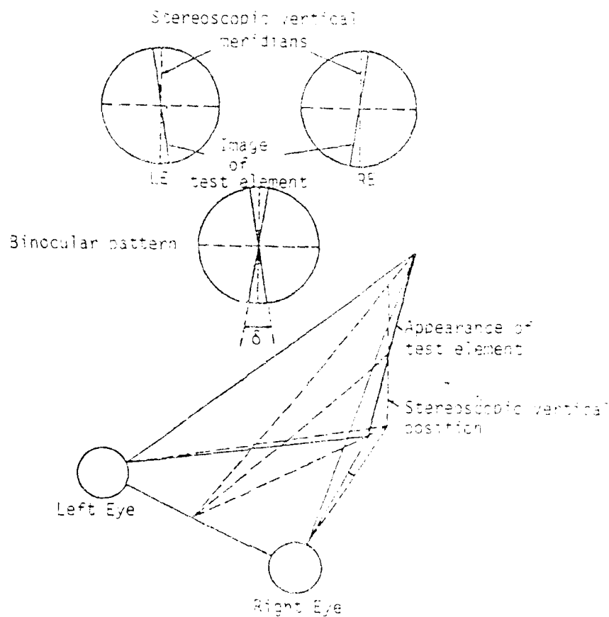
Figure 13. Top: The images of the test element are rotated from the stereoscopic vertical meridians. Bottom: The binocular spatial localization of the test element. (Allerbrook, 1954)
