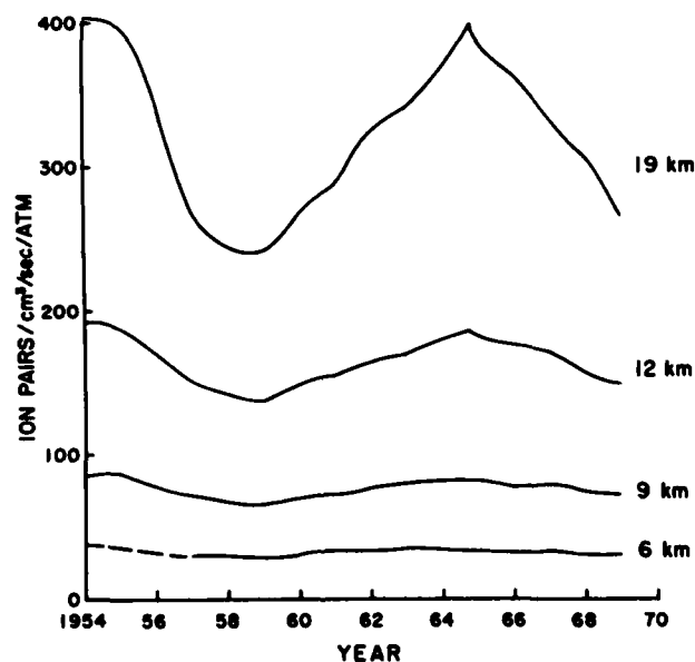
Figure 1. Galactic radiation level (indicated by air ionization) as related to phase of solar cycle and altitude at 88^\circ\text{N} geomagnetic latitude (3). (These curves do not accurately reflect relative amounts of variation in absorbed dose rate or dose-equivalent rate.)
