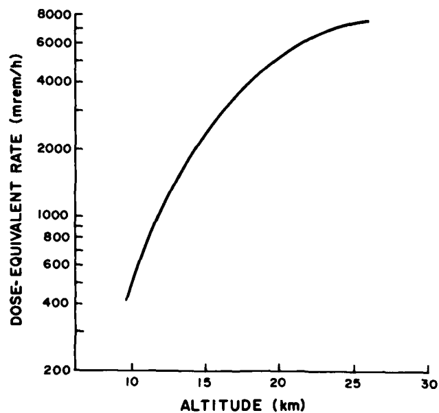
Figure 4. Upper limit estimate of dose-equivalent rate (extremity dose) versus altitude for the solar flare of February 23, 1956 (8).
