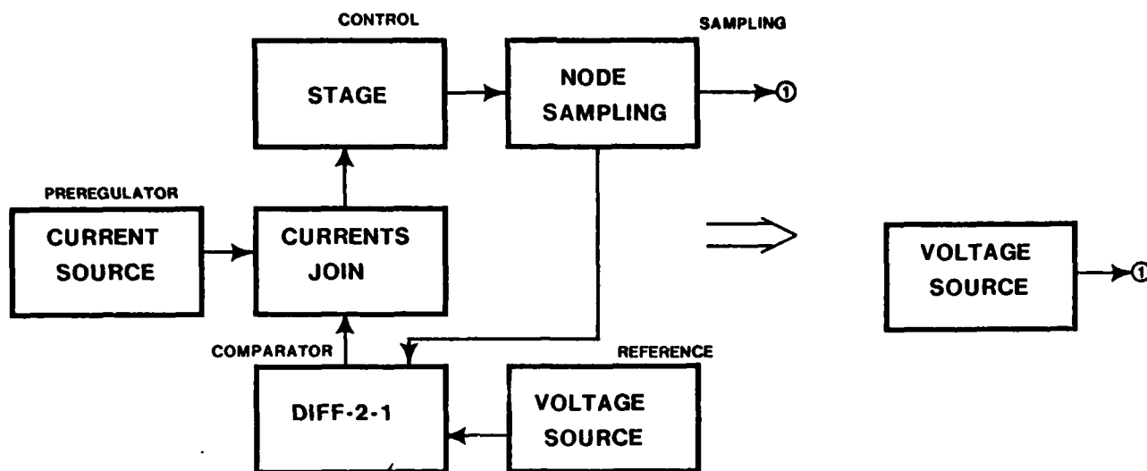
Figure 18 : Rule VOLTAGE-COMPLEX-SERIES-PASS
