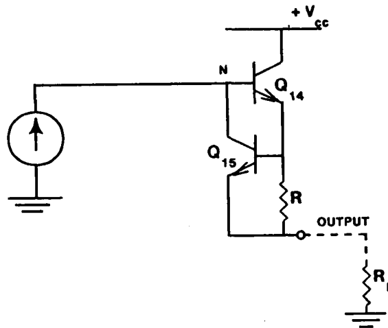
Figure 16 : Current Limiter
