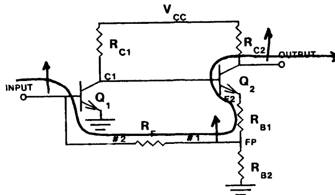
Figure 2 : Feedback Amplifier
