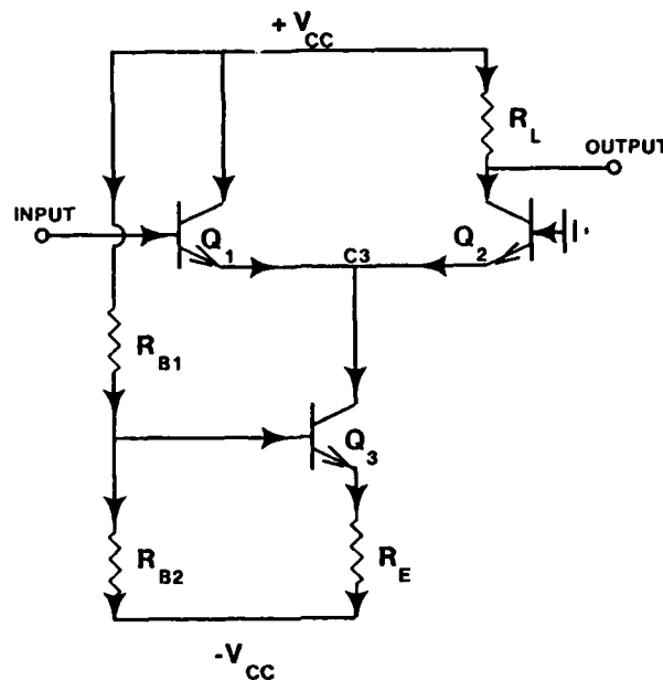
Figure 11 : Emitter-Coupled Pair
