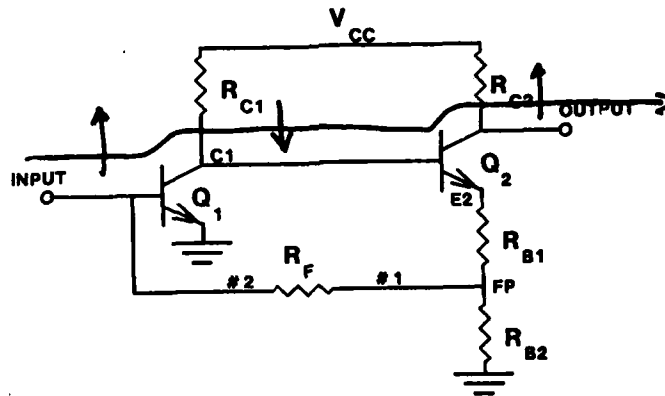
Figure 1 : Feedback Amplifier
