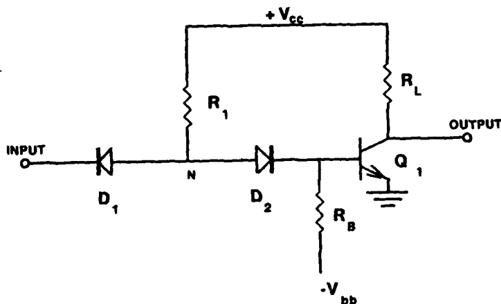
Figure 7 : DTL-inverter
