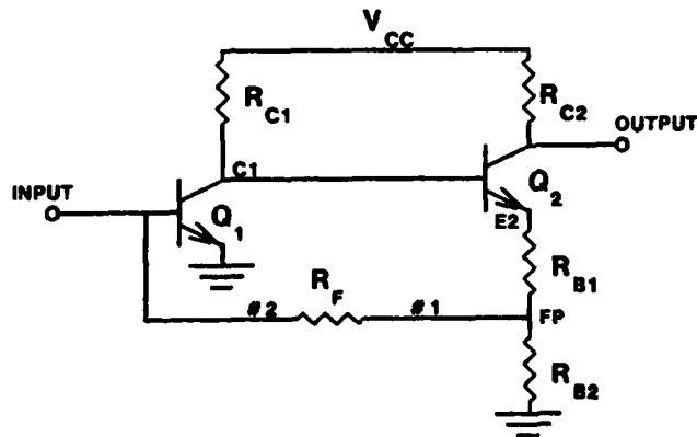
Figure 4 : CE-FEEDBACK
