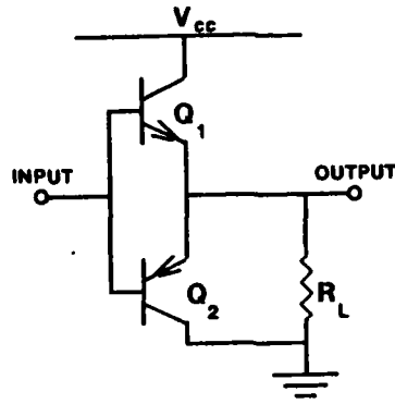
Figure 9 : Unbiased Complementary Pair
