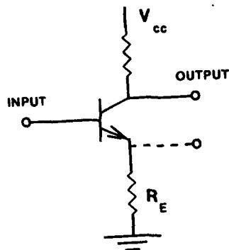
Figure 13 : Common-Emitter Amplifier
