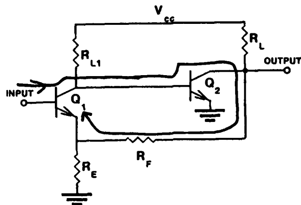
Figure 11 : Loop-Node Feedback Amplifier
