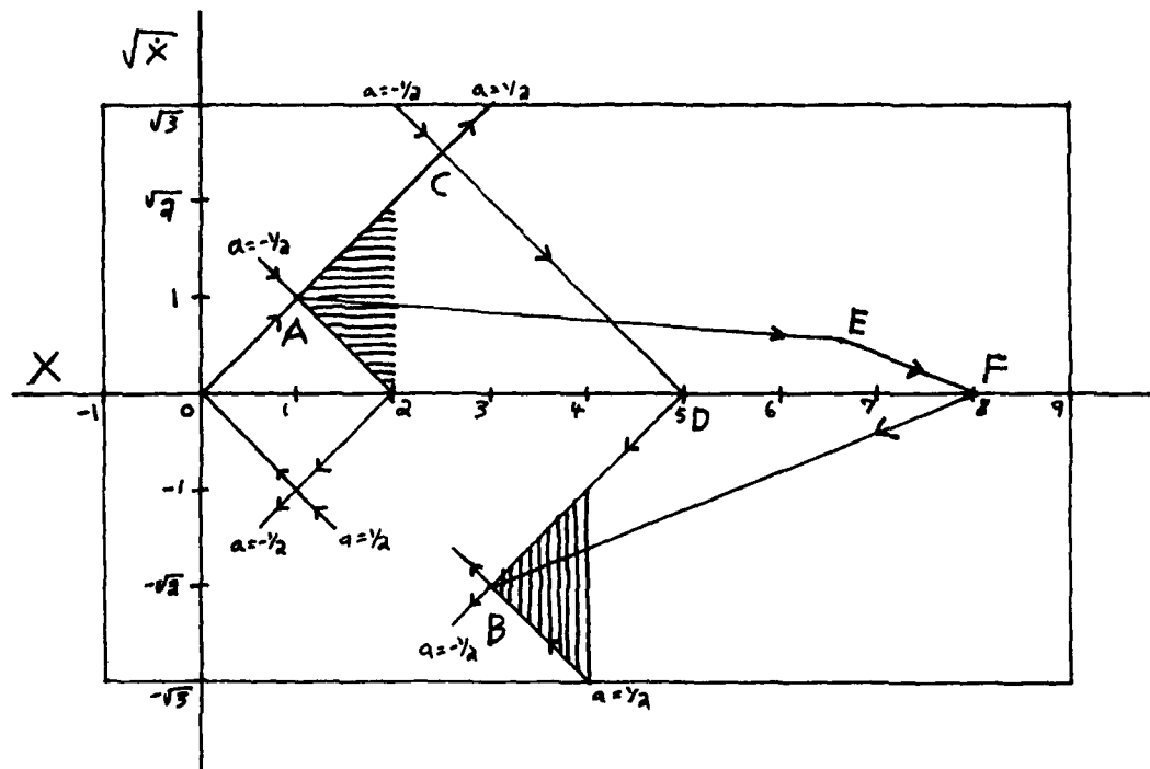
Figure 5: Phase space graph for trajectories.
