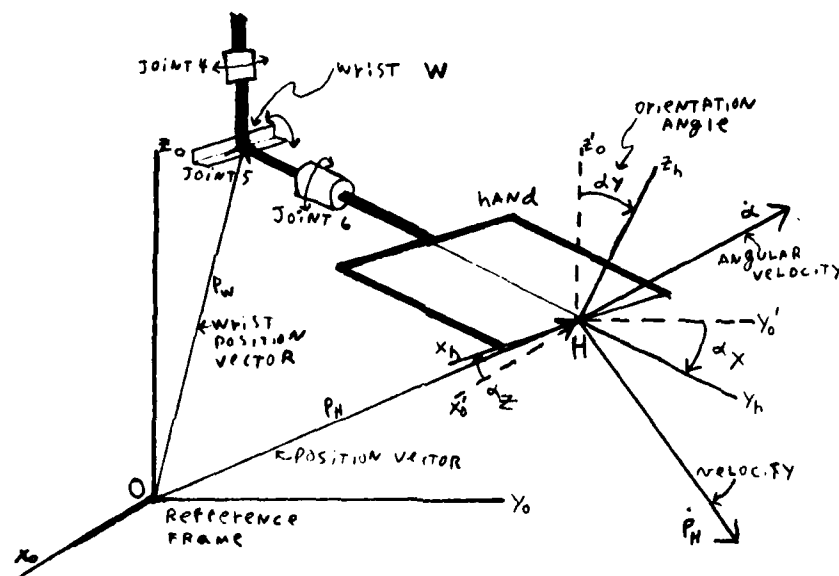
Figure 4: Hand oriented coordinates for the Scheinman arm.
