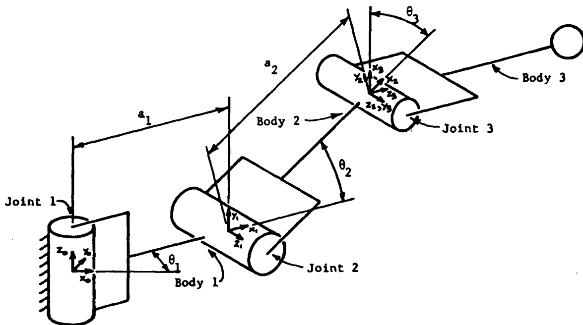
Figure 2: Schematic of a three joint arm.
