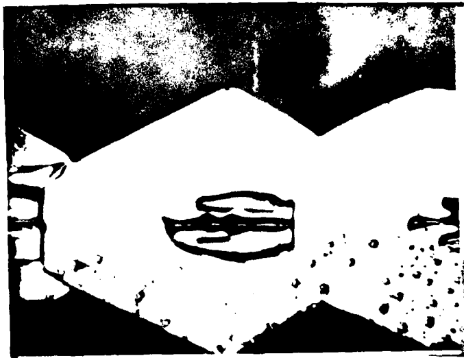
Figure 11 Typical Dendrite Surface at 100X.
